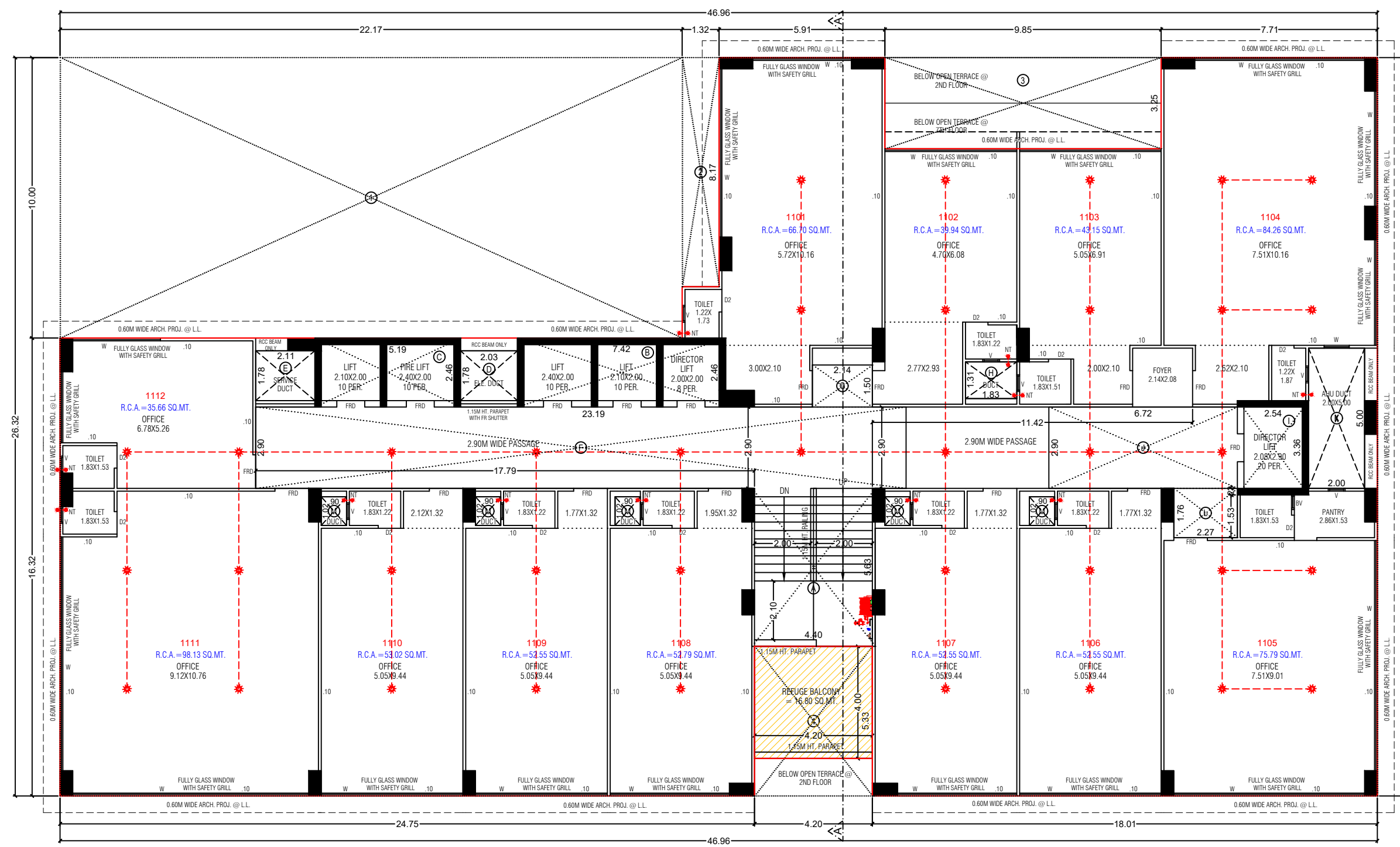
11TH FLOOR PLAN
