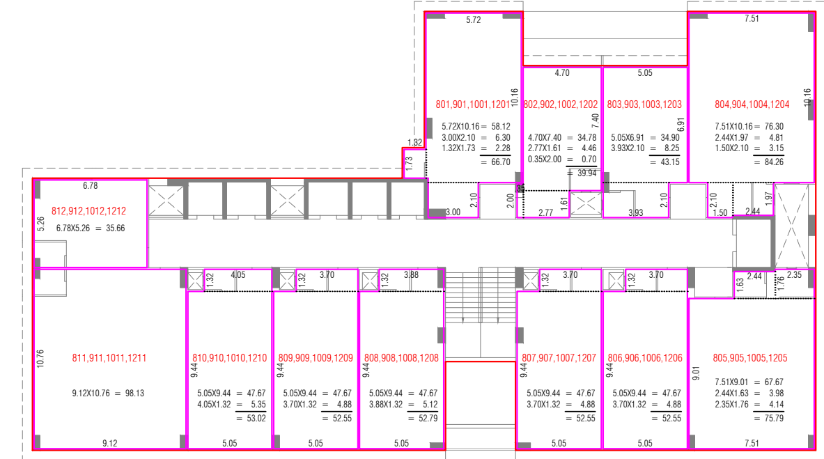
RERA CARPET AREA CAL. (8TH, 9TH, 10TH & 12TH FLOOR PLAN)
