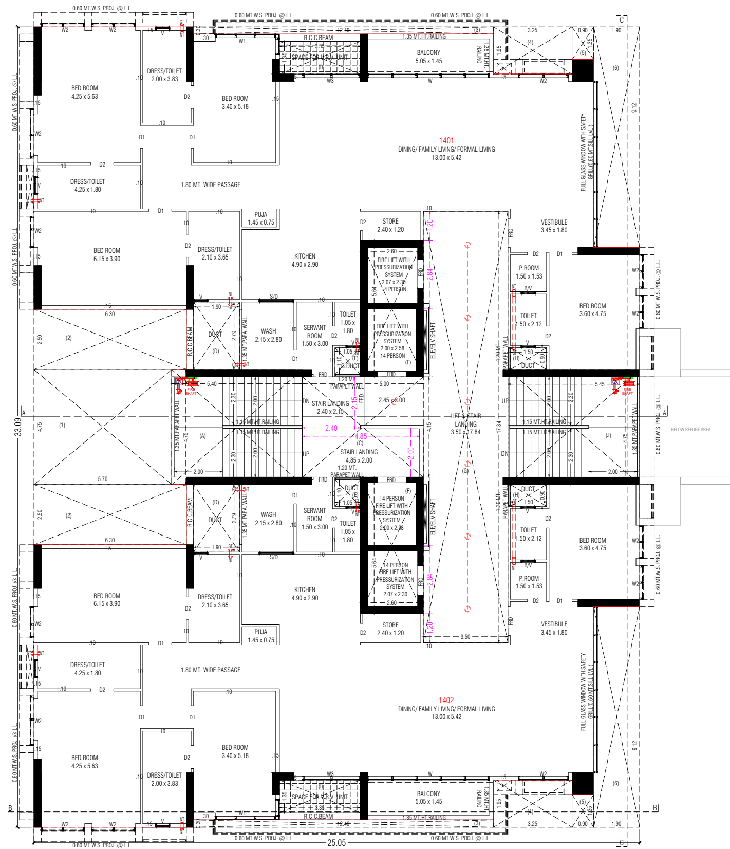
14TH. FLOOR PLAN
