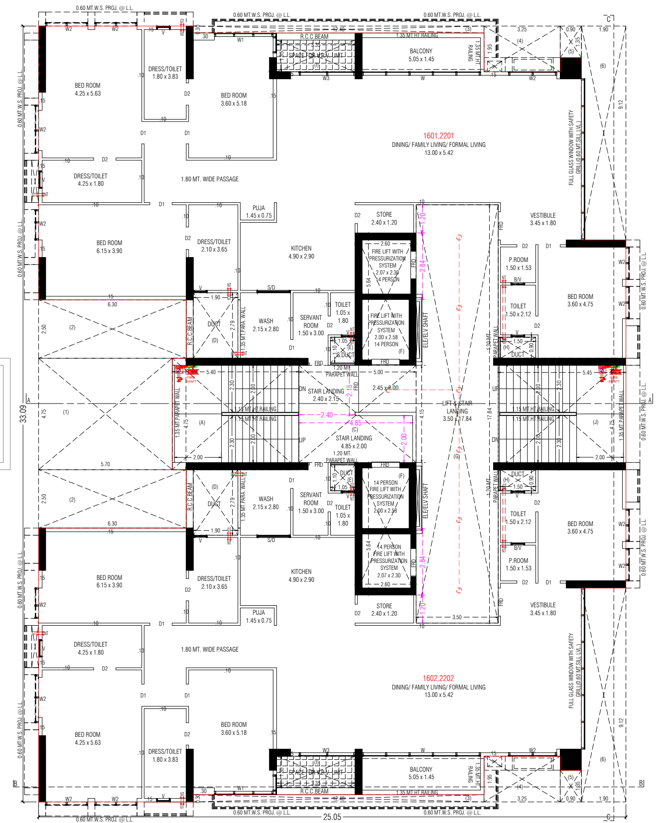
16TH. & 22ND. FLOOR PLAN
