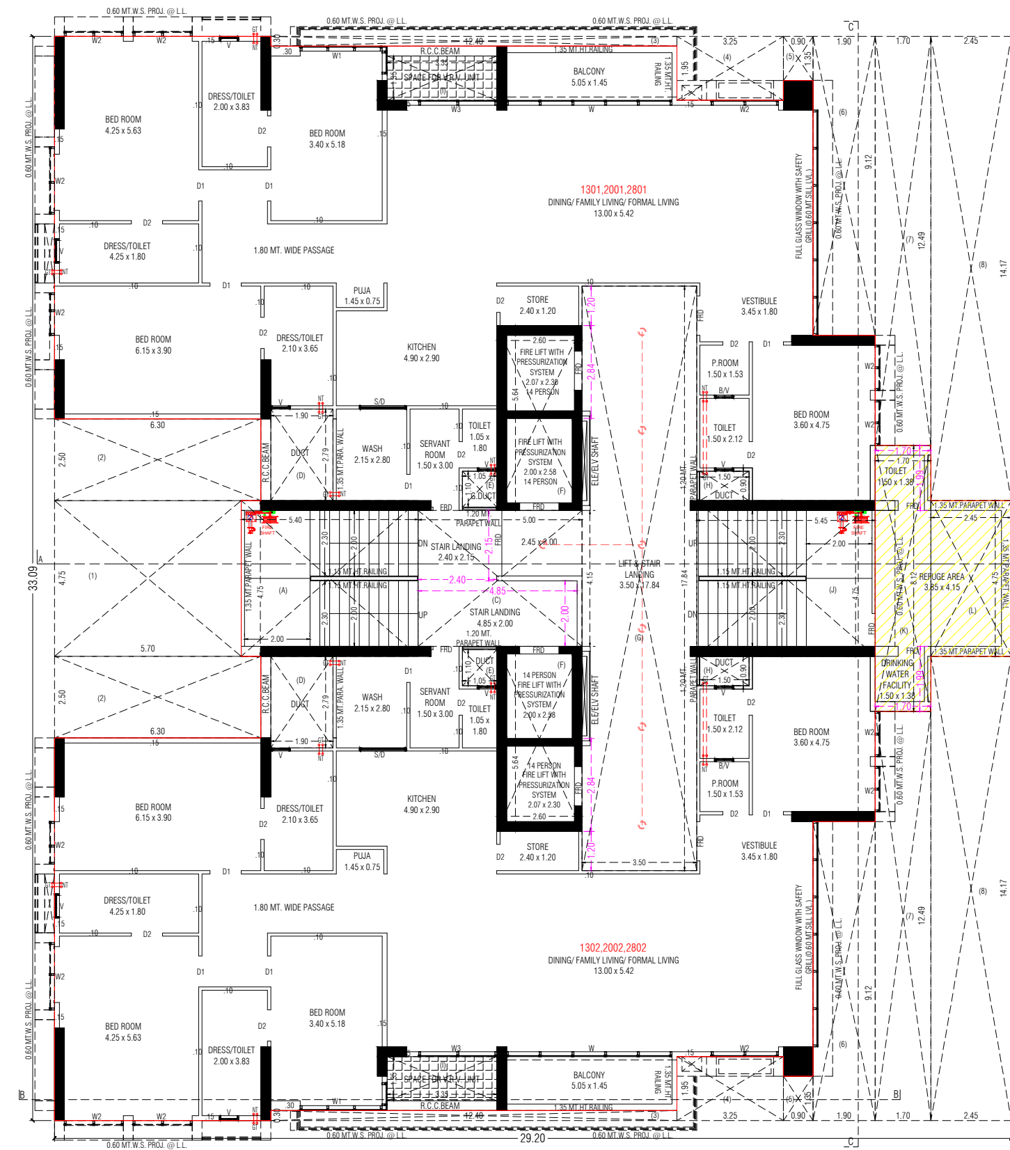
13TH., 20TH. & 28TH. FLOOR PLAN
