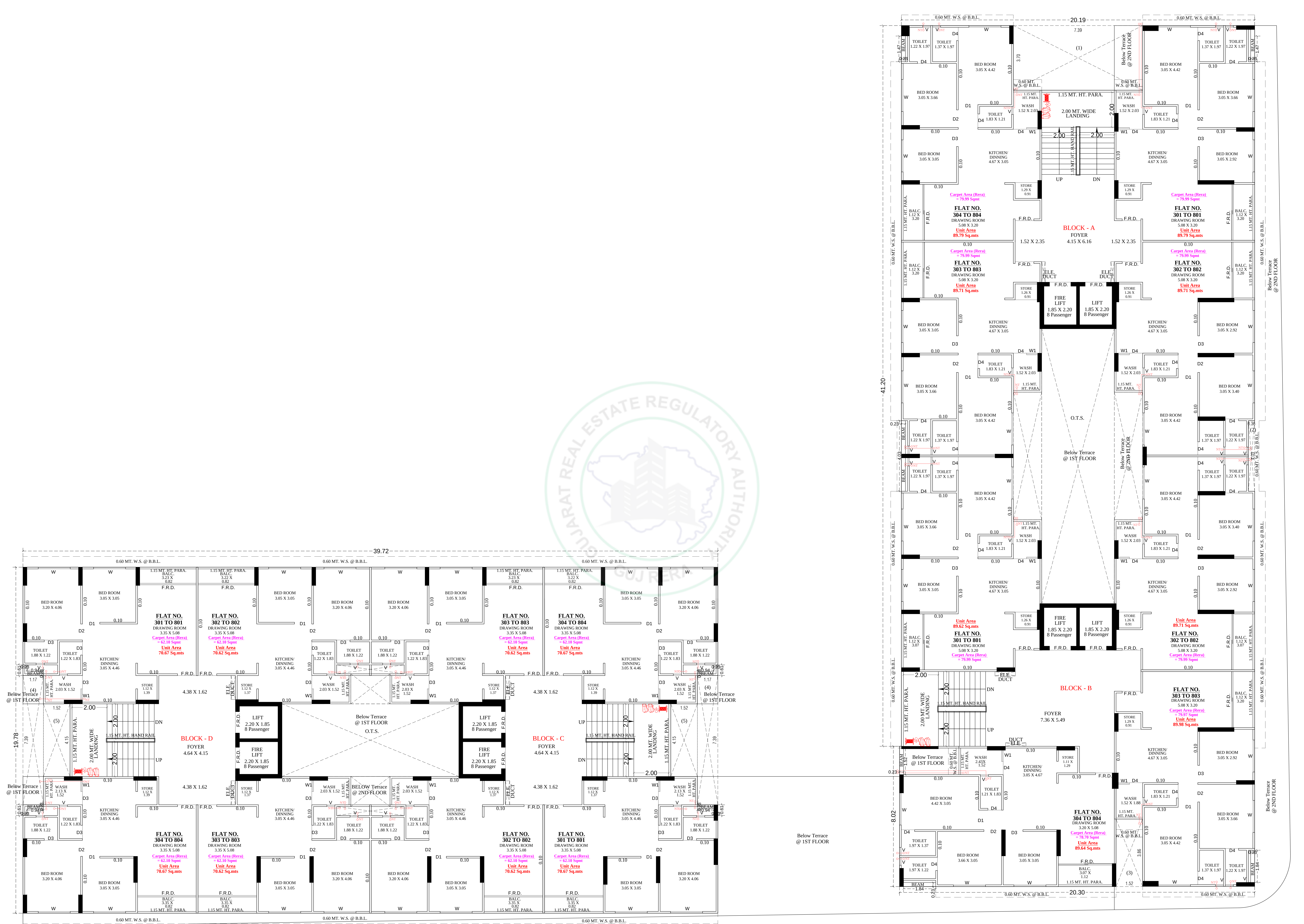
3RD TO 8TH FLOOR PLAN NOTE :- ALL OUTER & INTERNAL WALL ARE OF 0.115 MT. TH. B/K WALL
