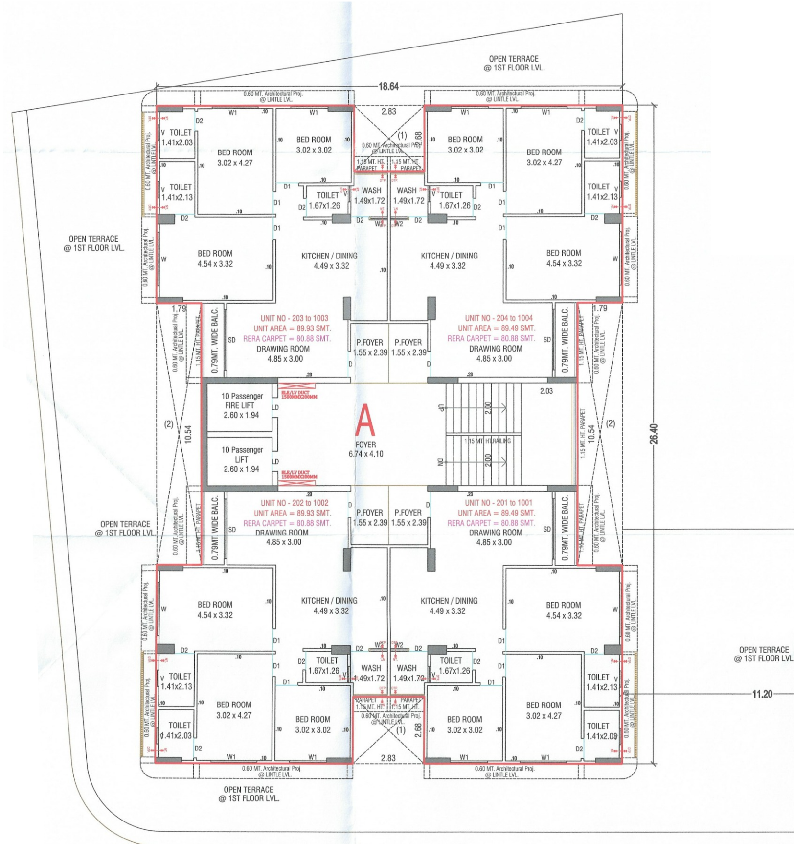
2ND TO 10TH FLOOR PLAN
