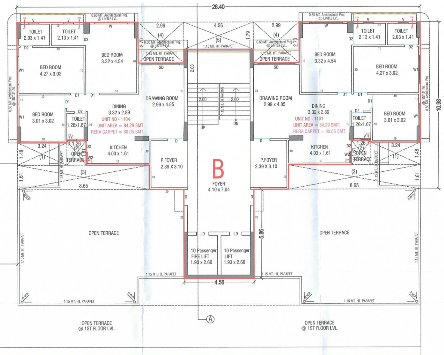
11TH FLOOR PLAN
