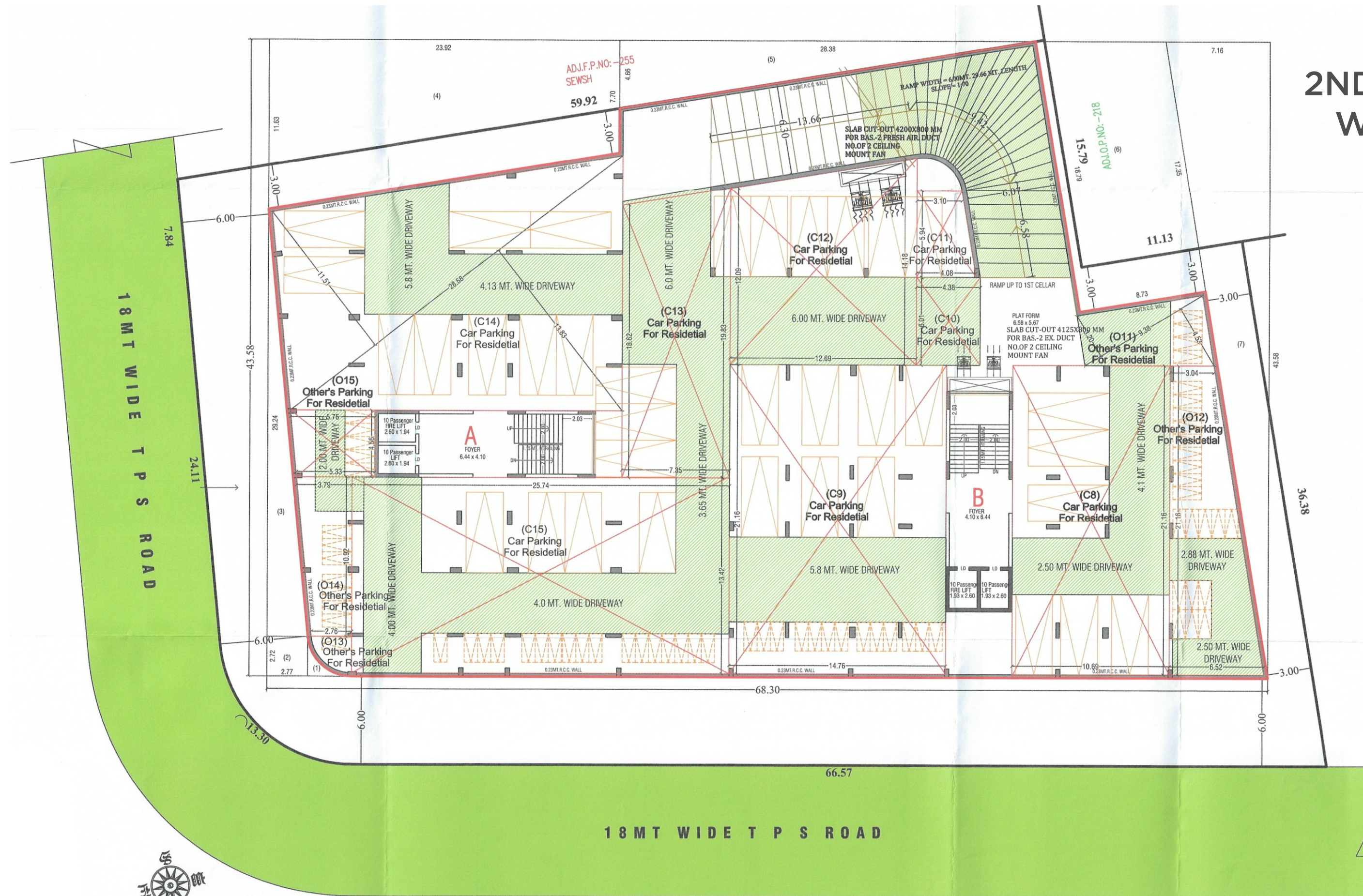
2ND BASEMENT WITH LAYOUT PLAN SCALE :1 C.M.= 2 MT.
