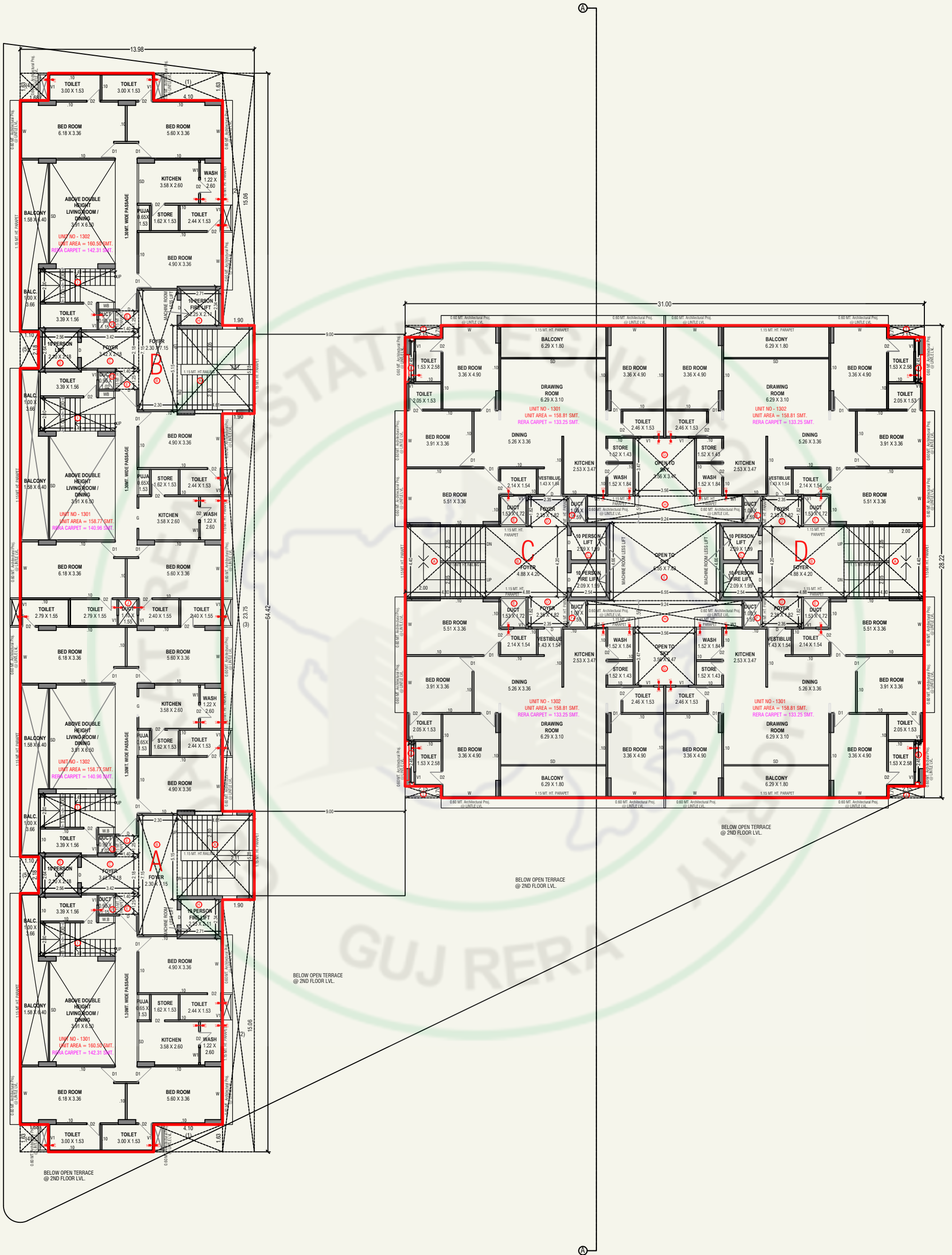
13TH FLOOR PLAN
