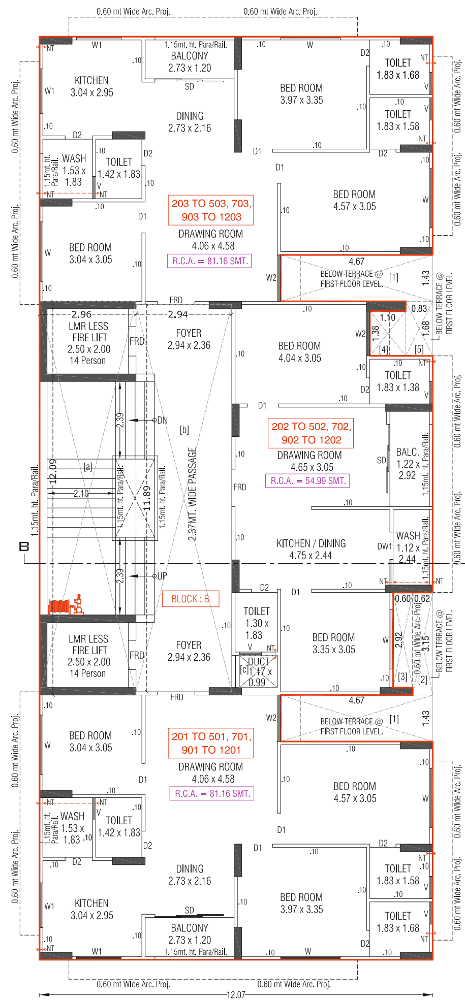
TYPICAL FLOOR PLAN (2nd. TO 5th., 7th., 9th. to 12th. FLOOR PLAN)
