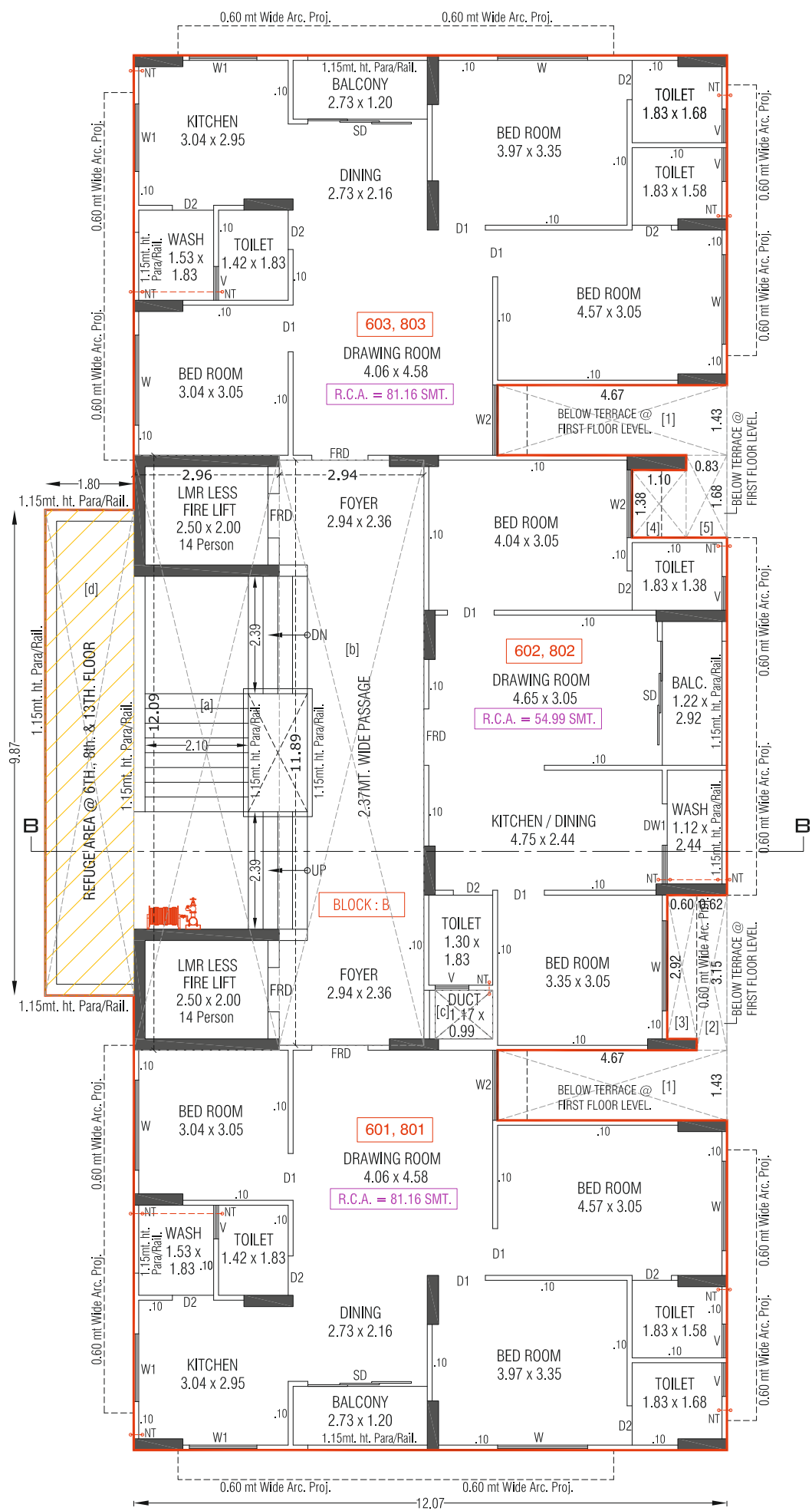
TYPICAL FLOOR PLAN (6th. & 8th. FLOOR PLAN WITH REFUGE AREA)
