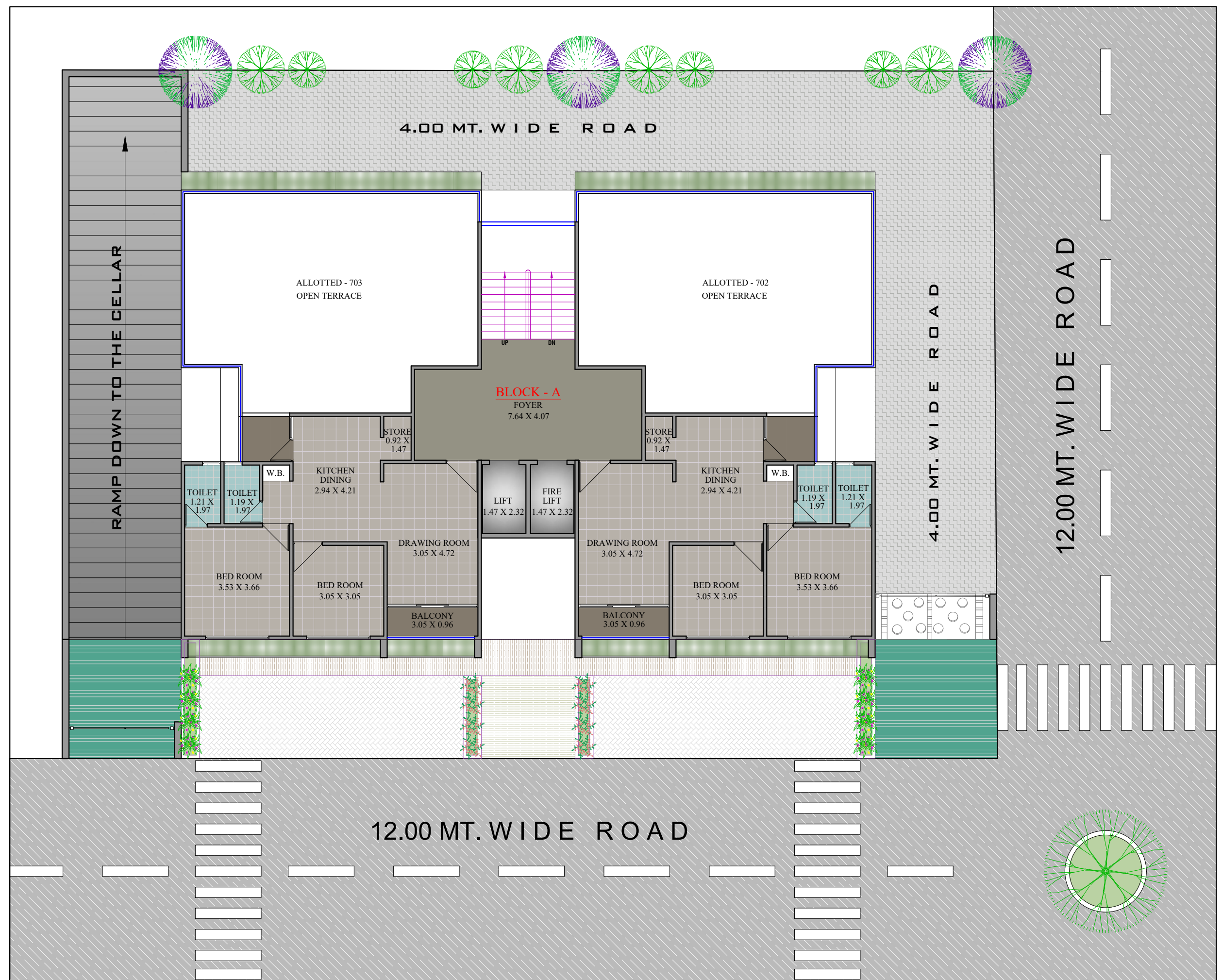
7TH FLOOR PLAN LAYOUT PLAN
