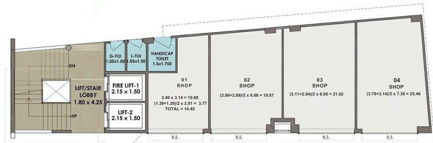
FLOOR PLAN | GROUND LEVEL RETAIL
