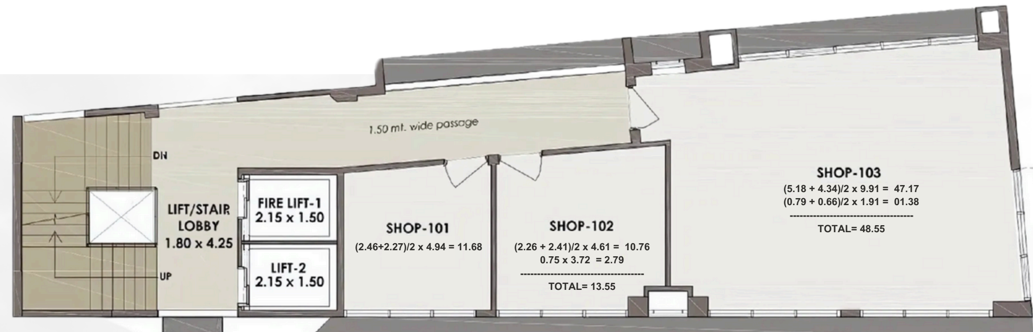
FLOOR PLAN | FIRST LEVEL RETAIL
