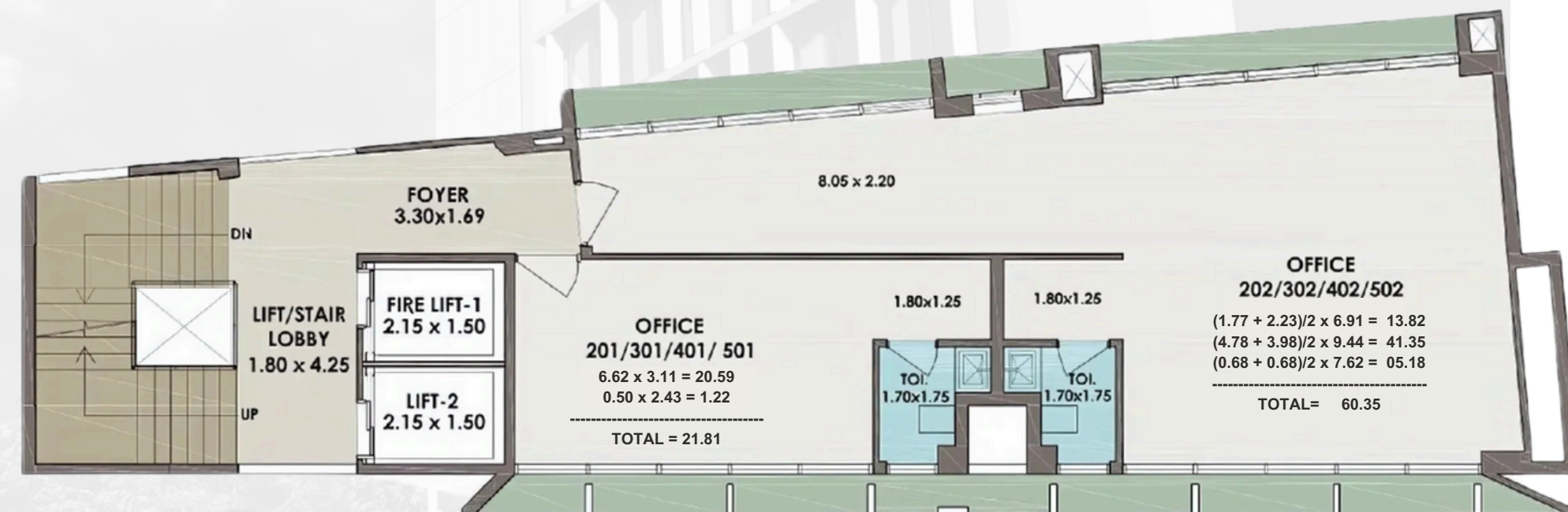
FLOOR PLAN | TYPICAL LEVEL OFFICE - 2 | 3 | 4 | 5
