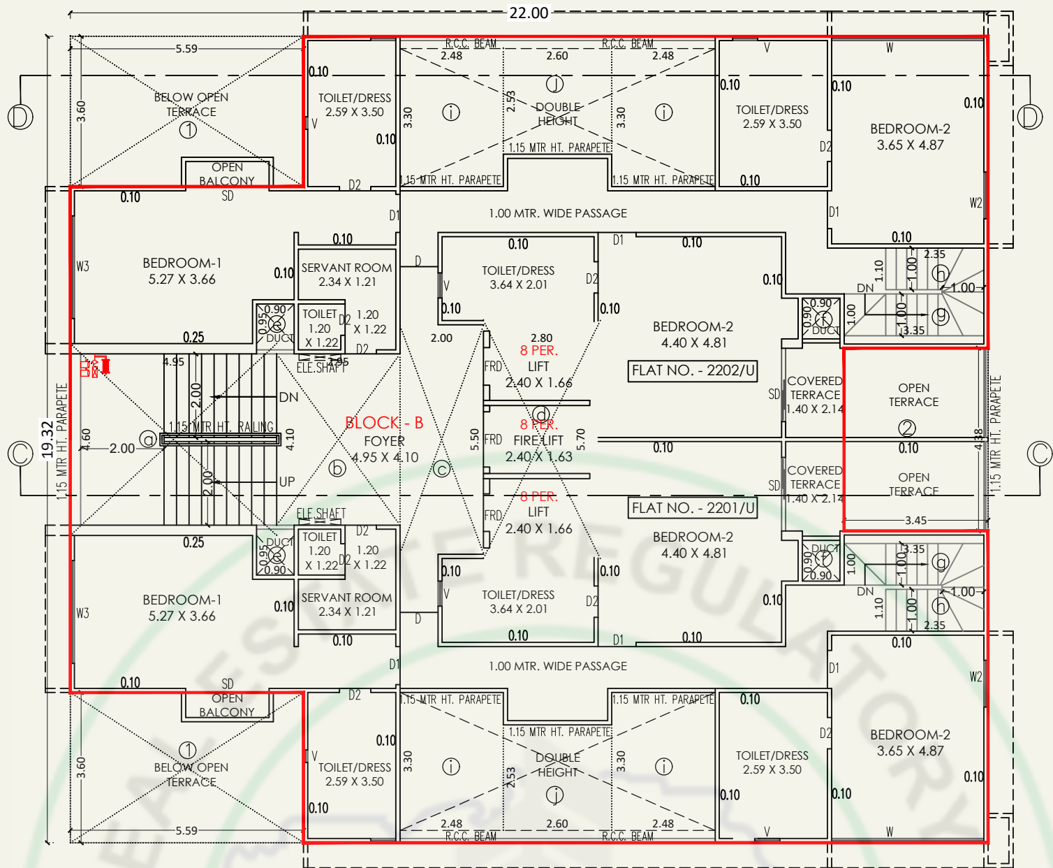
23rd FLOOR PLAN (BLOCK-B)
