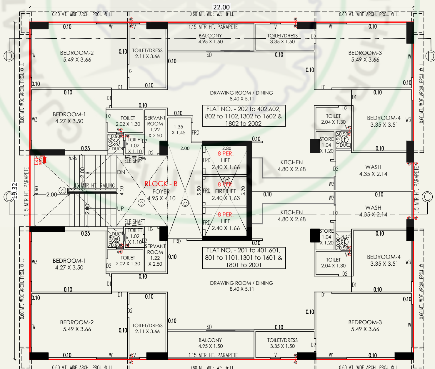
2nd to 4th, 6th, 8th to 11th, 13th to 16th, 18th to 20th FLOOR PLAN (BLOCK-B)
