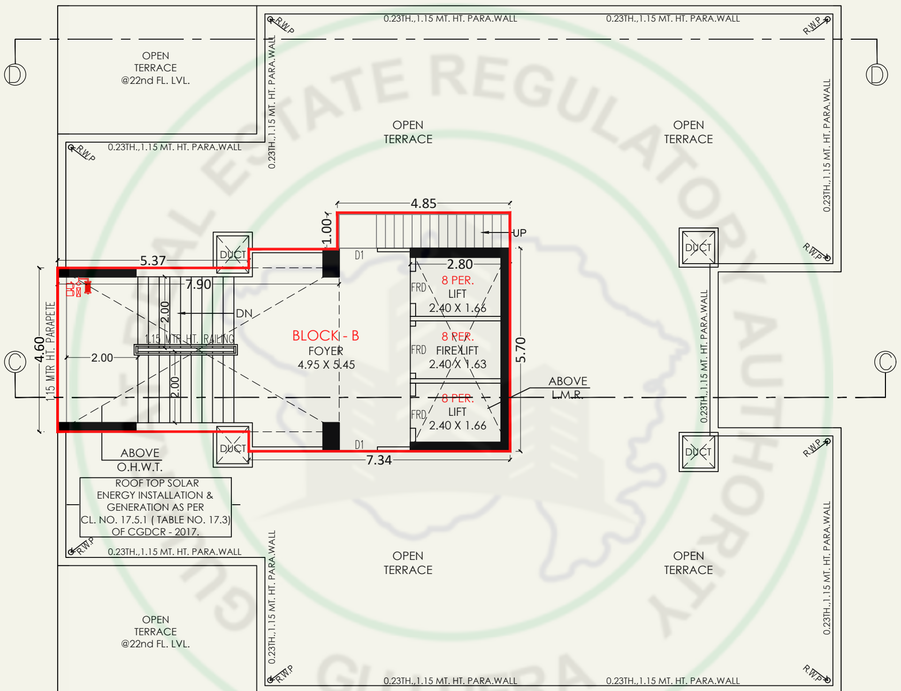
TERRACE PLAN (BLOCK-B)
