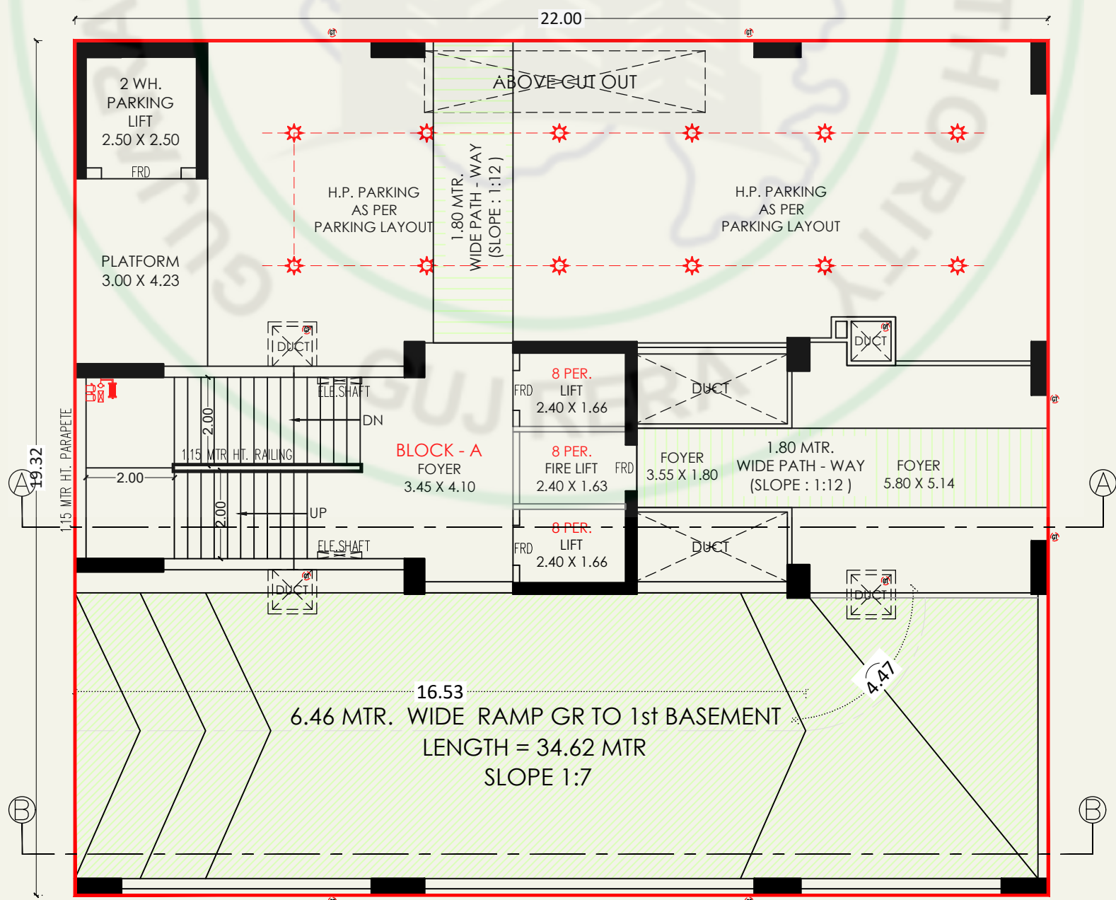
GROUND FLOOR PLAN (BLOCK-A)
