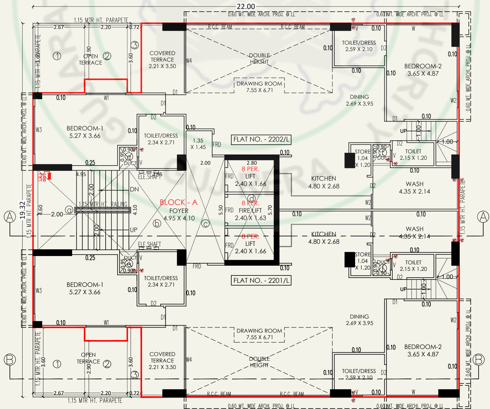
22nd FLOOR PLAN (BLOCK-A)
