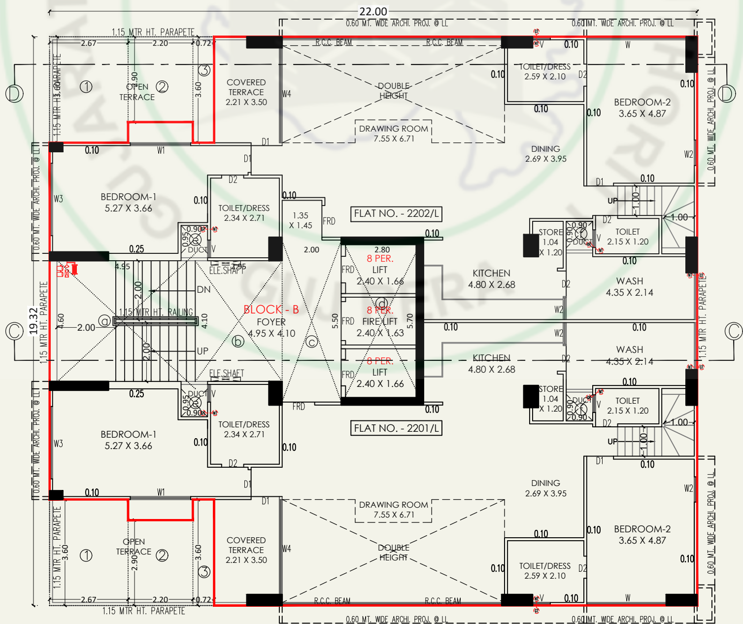
22nd FLOOR PLAN (BLOCK-B)
