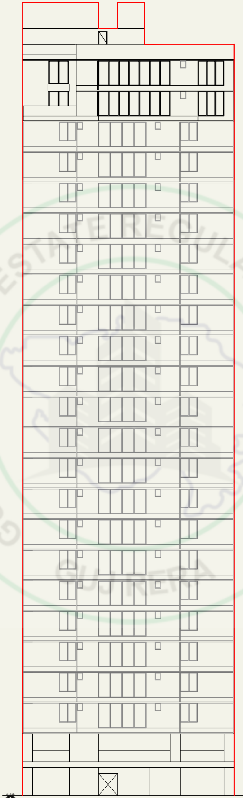
ELEVATION (BLOCK-B)
