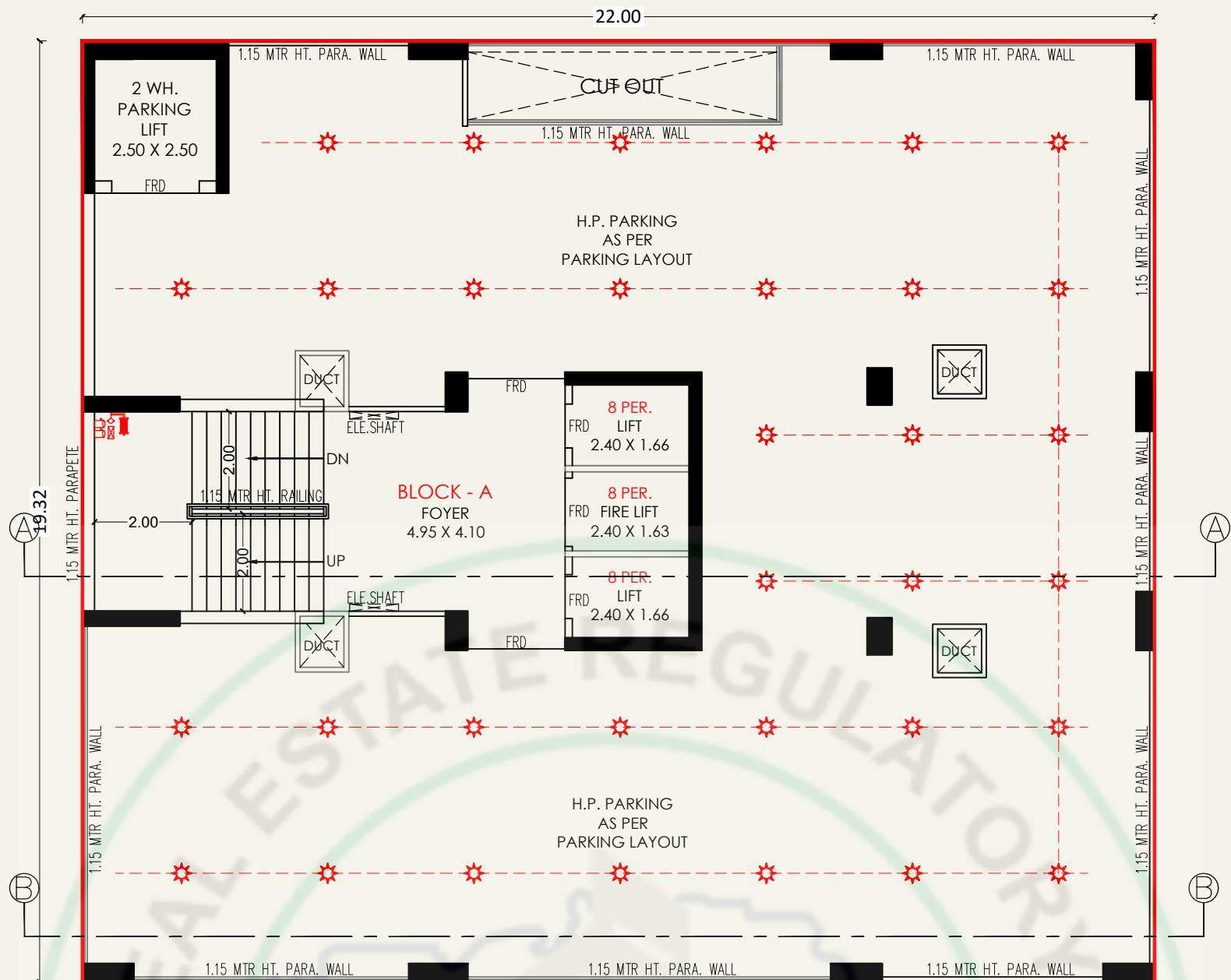
FIRST FLOOR PLAN (BLOCK-A)
