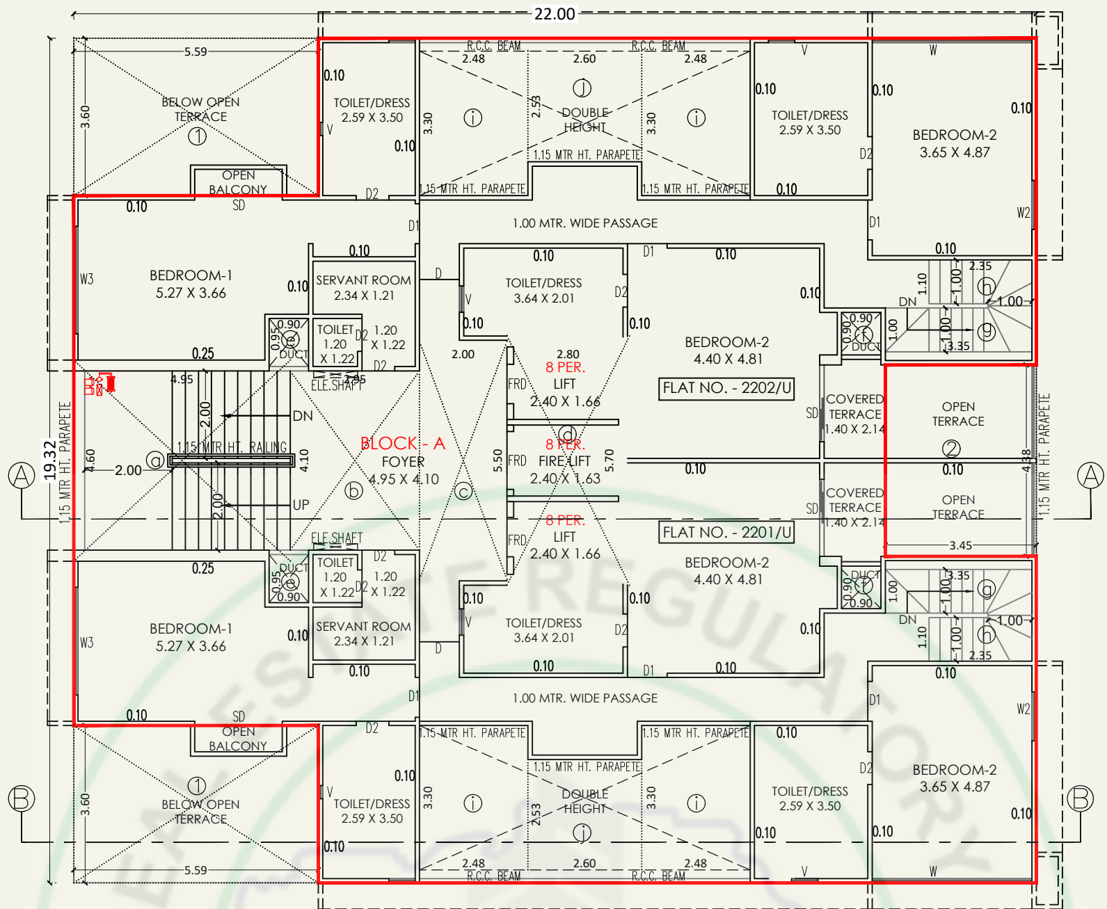
23rd FLOOR PLAN (BLOCK-A)
