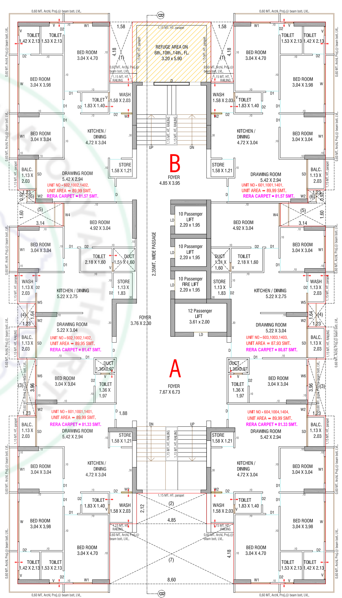
REFUGE AREA FLOOR PLAN 6TH,10TH,14TH, FLOOR PLAN
