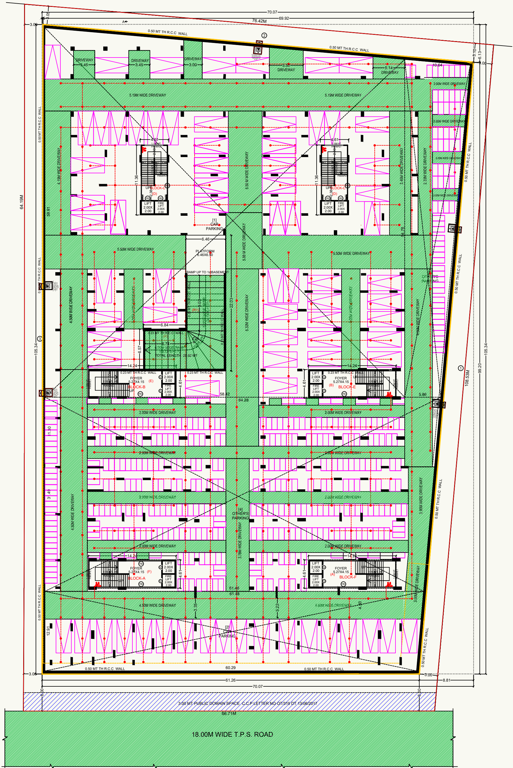
2ND BASEMENT PLAN
