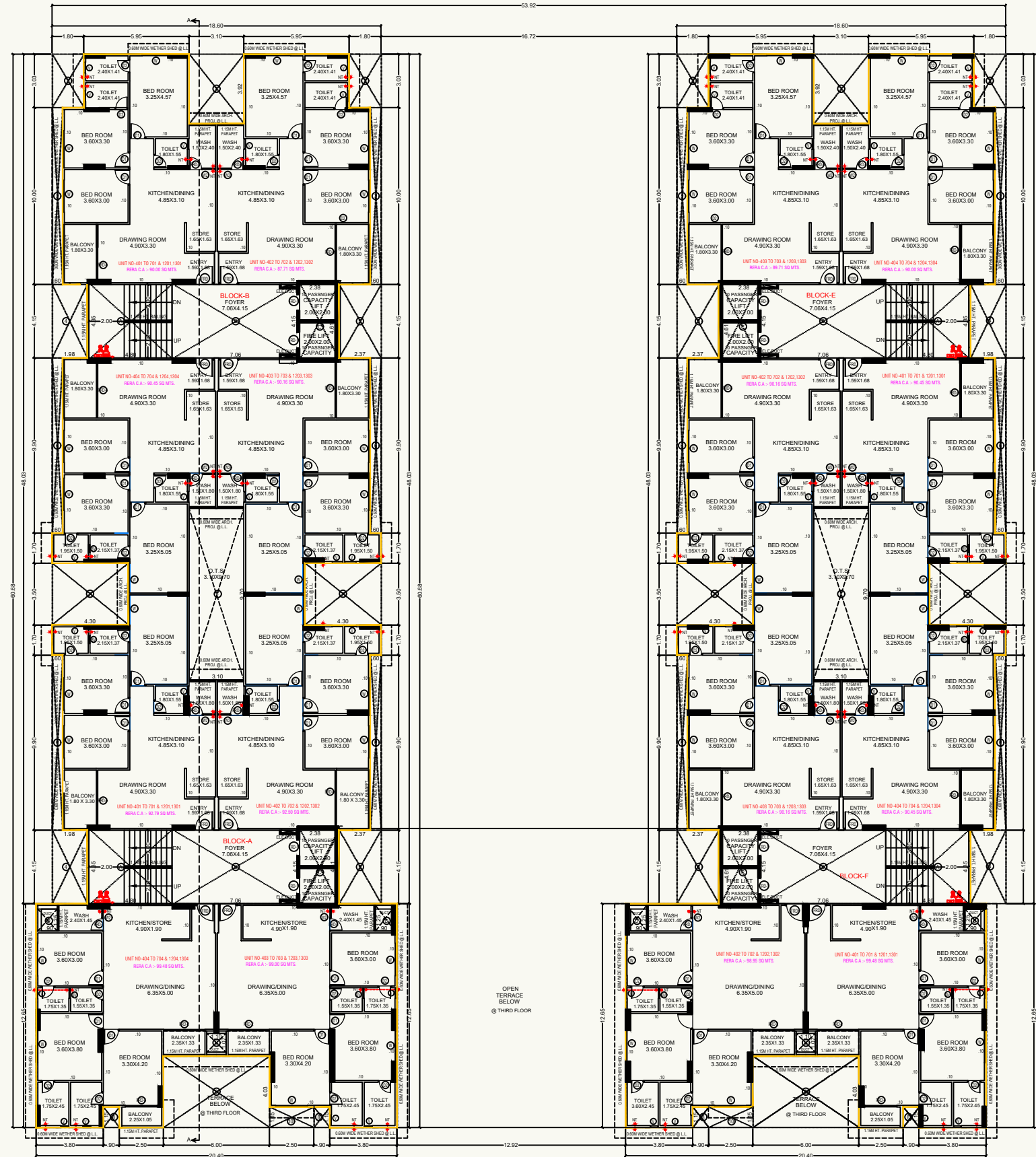
4TH TO 7TH, 12TH & 13TH FLOOR PLAN (BLOCK-A+B+E+F)
