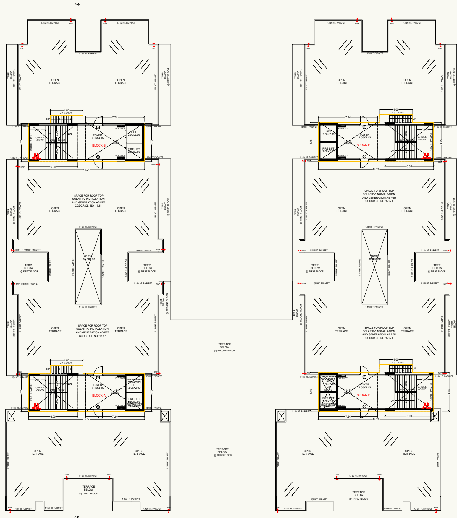
STAIR CABIN & TERRACE PLAN (BLOCK-A+B+E+F)
