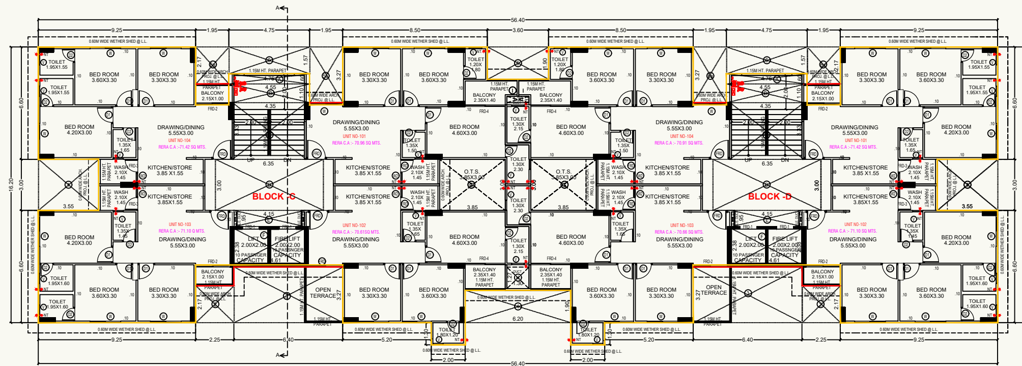
FIRST FLOOR PLAN (BLOCK-C+D)
