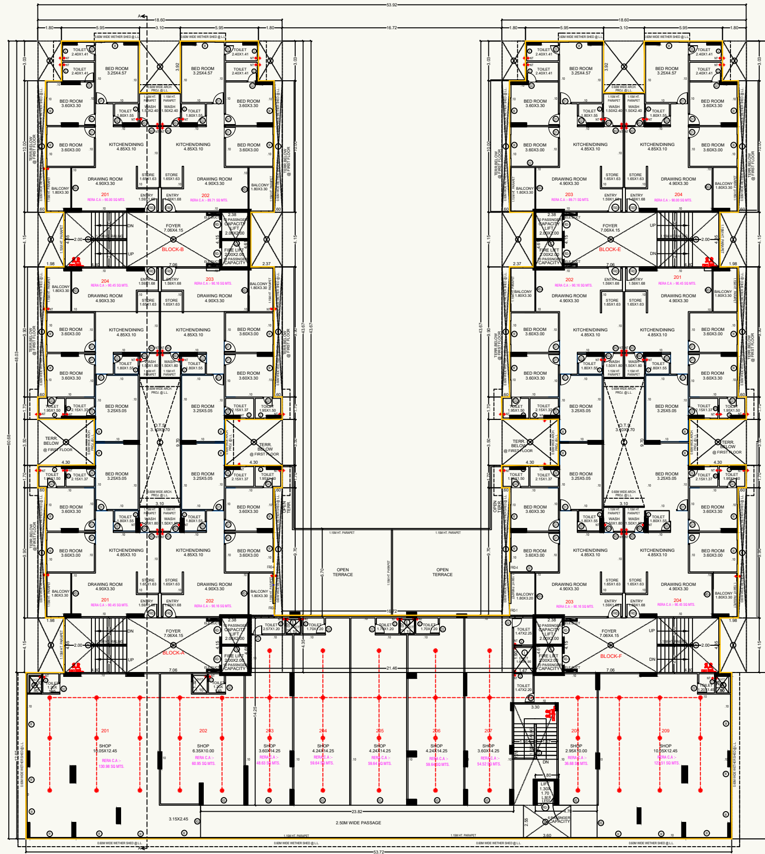
2ND FLOOR PLAN (BLOCK-A+B+E+F)
