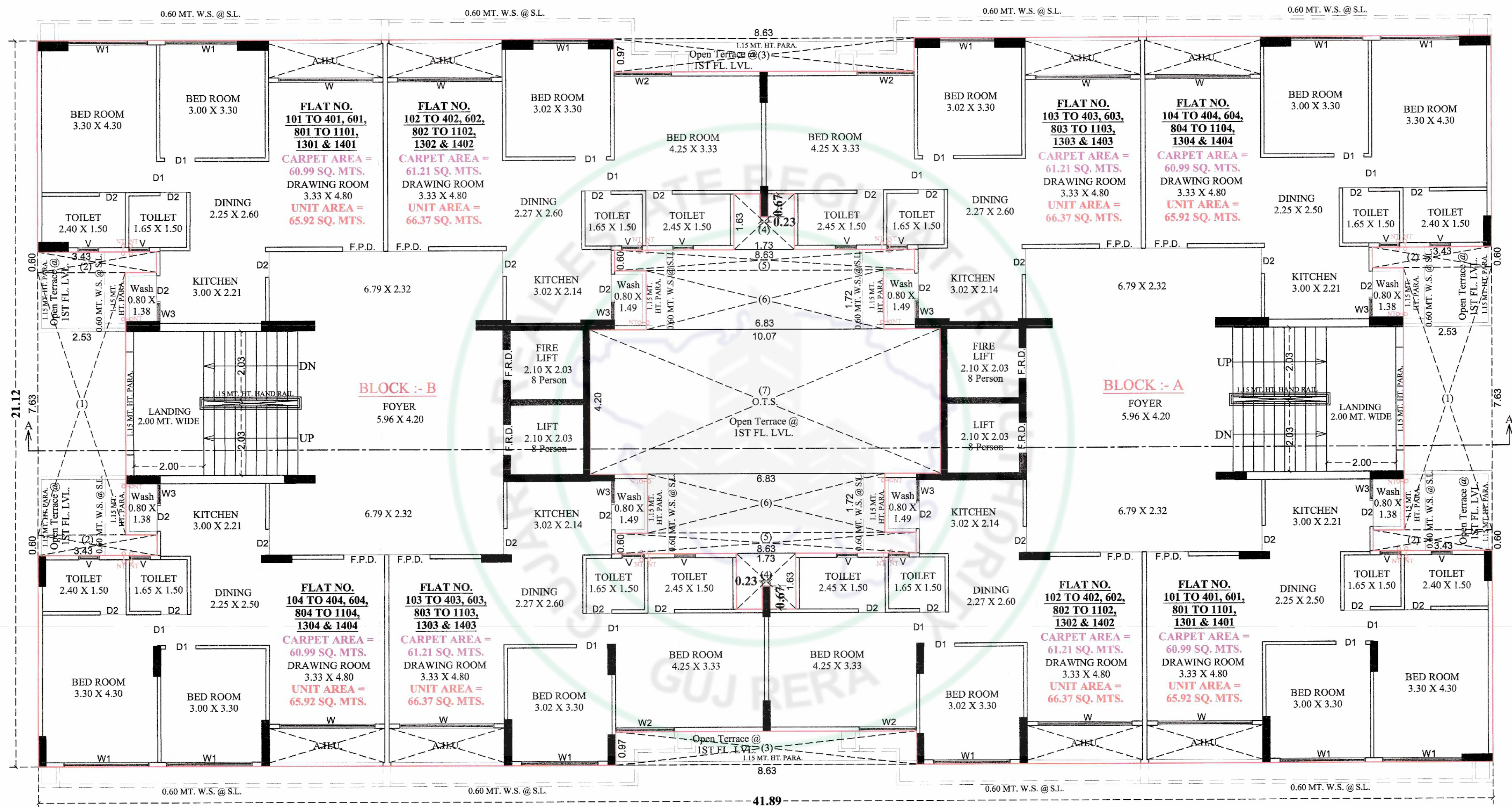
1ST TO 4TH, 6TH, 8TH TO 11TH, 13TH & 14TH FLOOR PLAN
