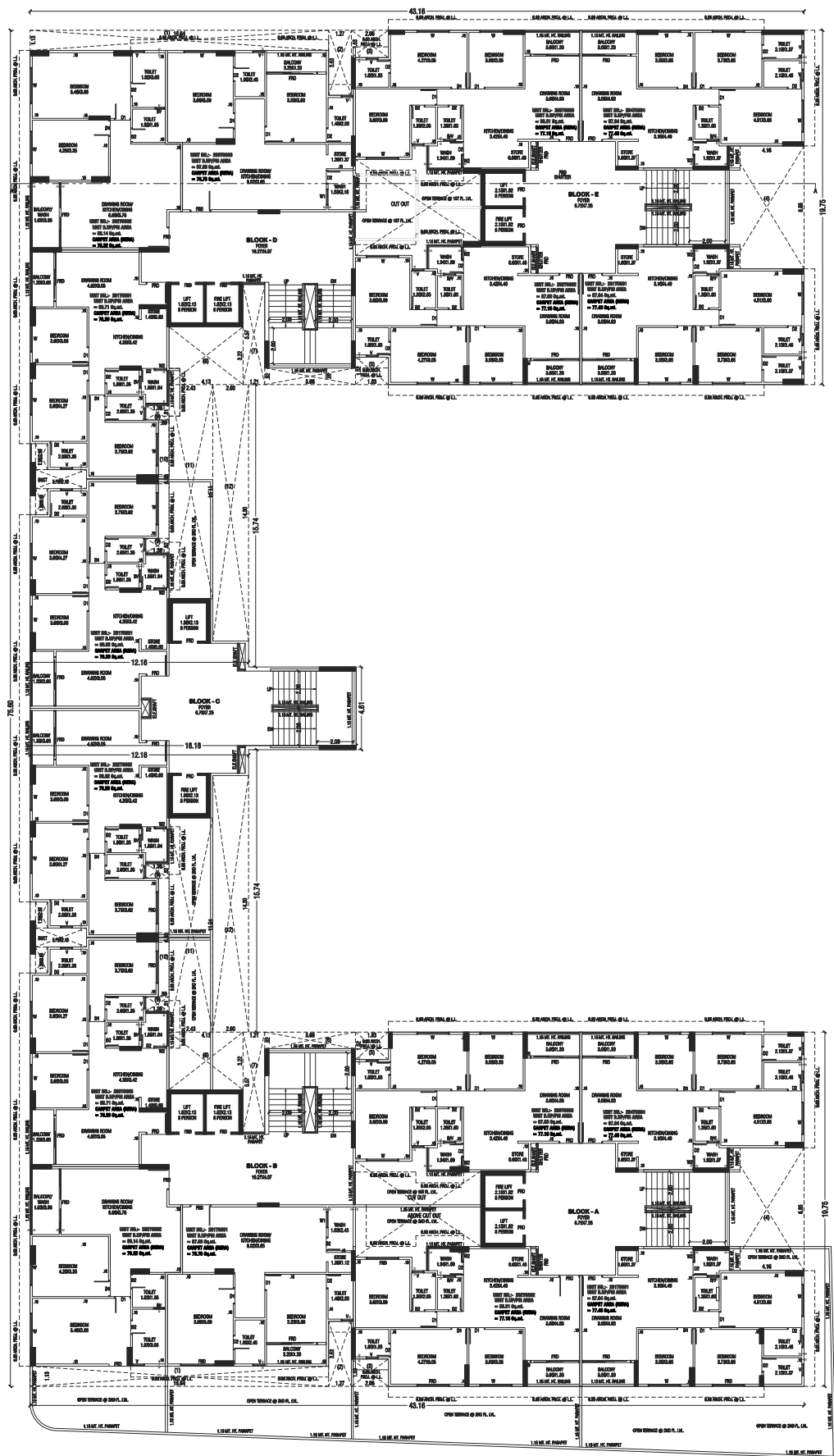
2ND FLOOR TO 9TH FLOOR PLAN LAYOUT PLAN
