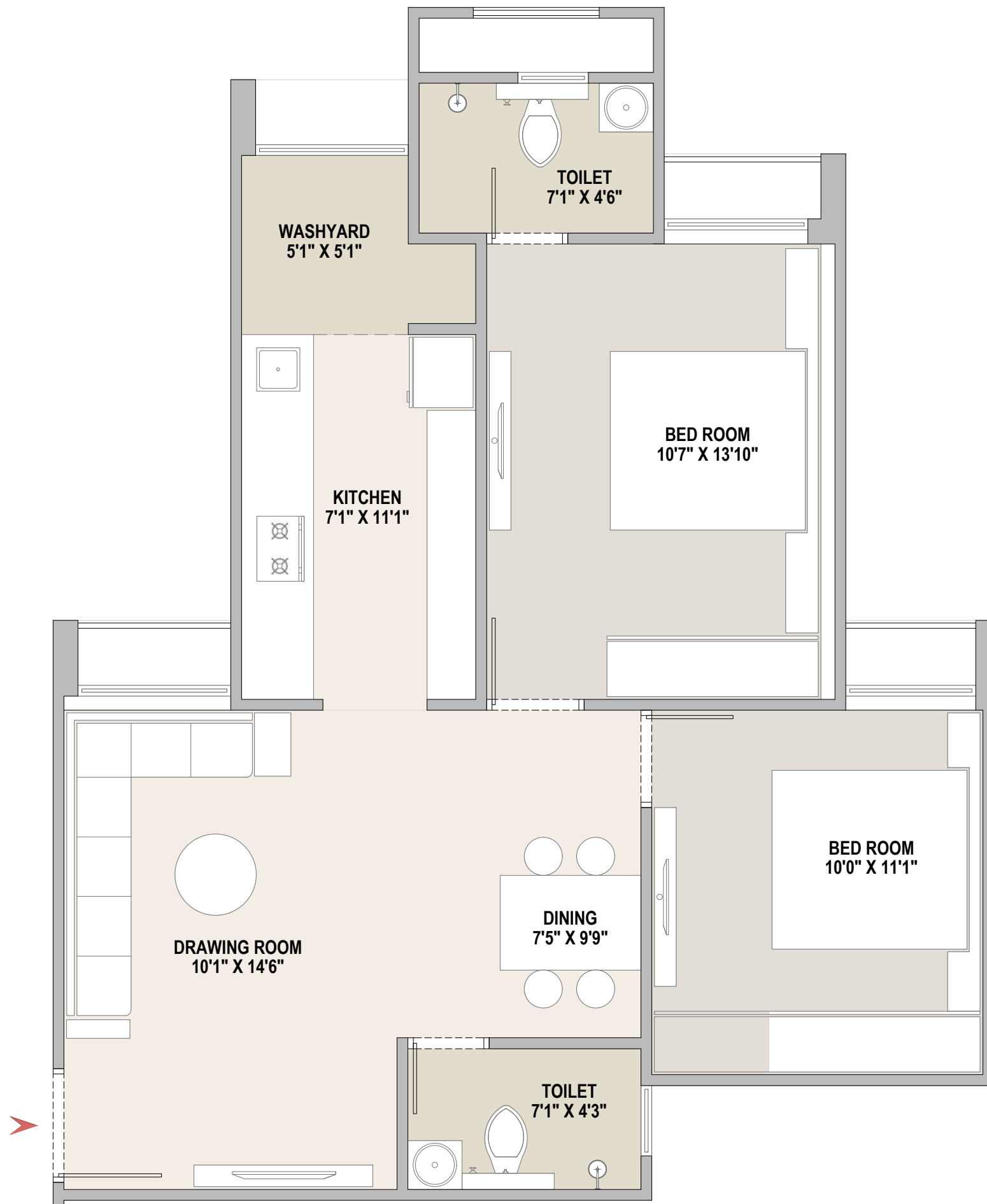
2BHK-D UNIT PLAN PROPOSED APARTMENT SCHEME AT AHMEDABAD
