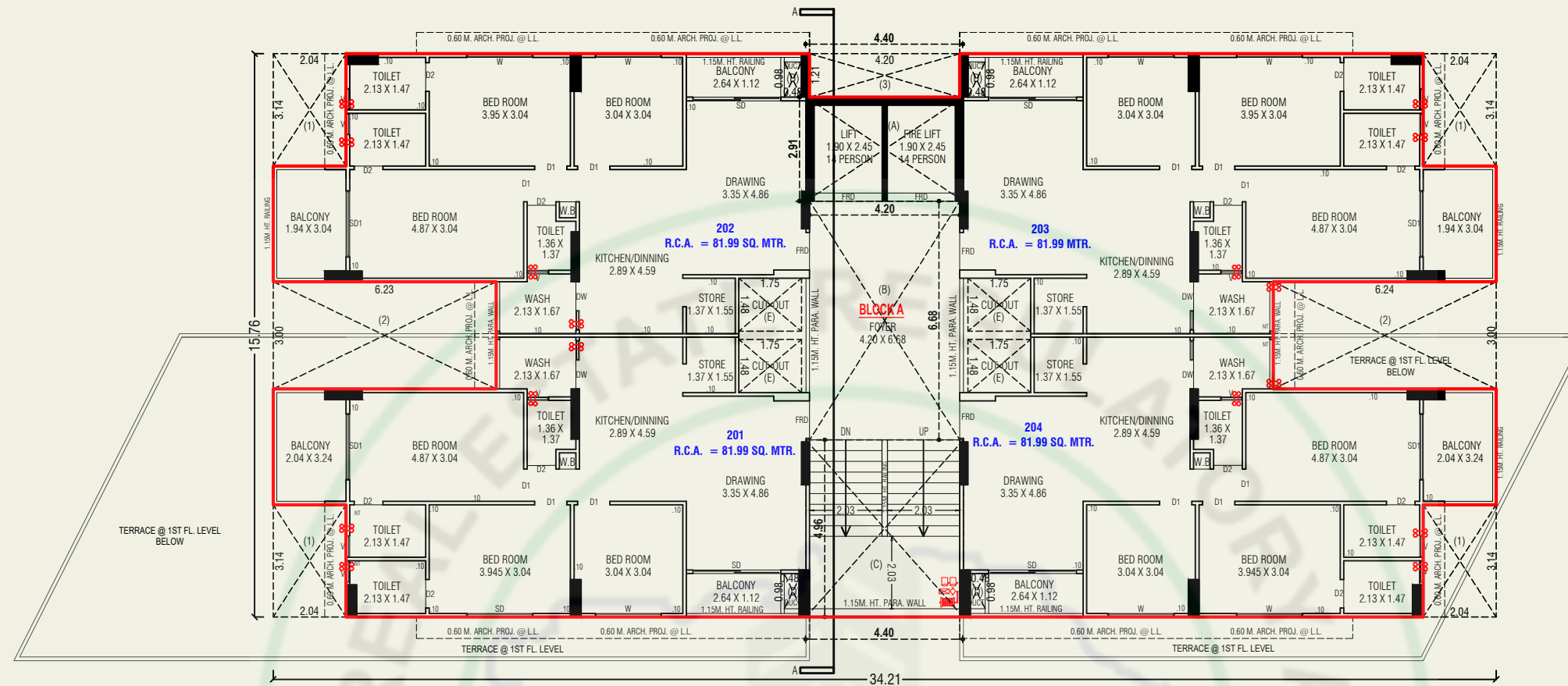
2ND FLOOR PLAN (BLOCK-A)
