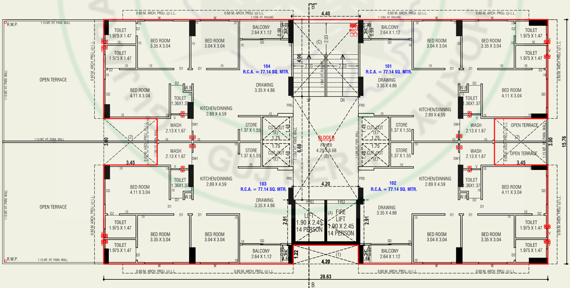
FIRST FLOOR PLAN (BLOCK-B)
