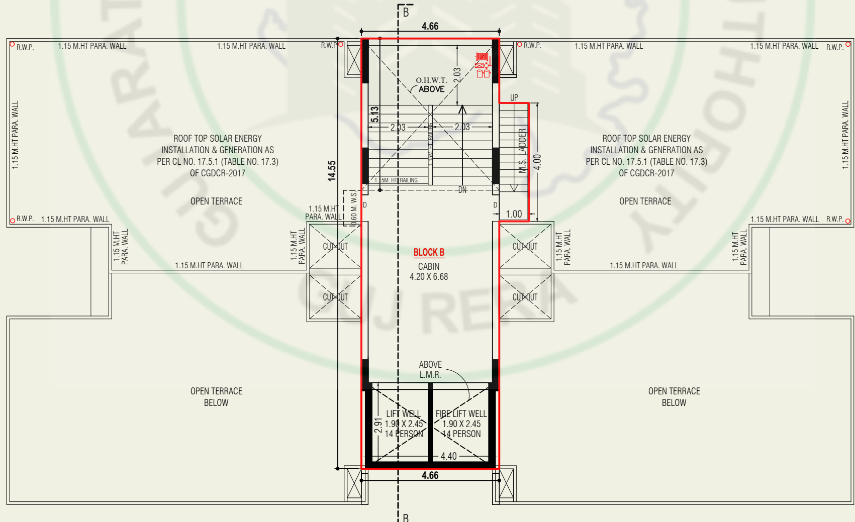
STAIR CABIN & OPEN TERRACE (BLOCK-B)
