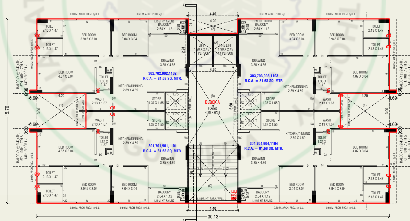
3RD, 7TH, 9TH & 11TH FLOOR PLAN (BLOCK-A)
