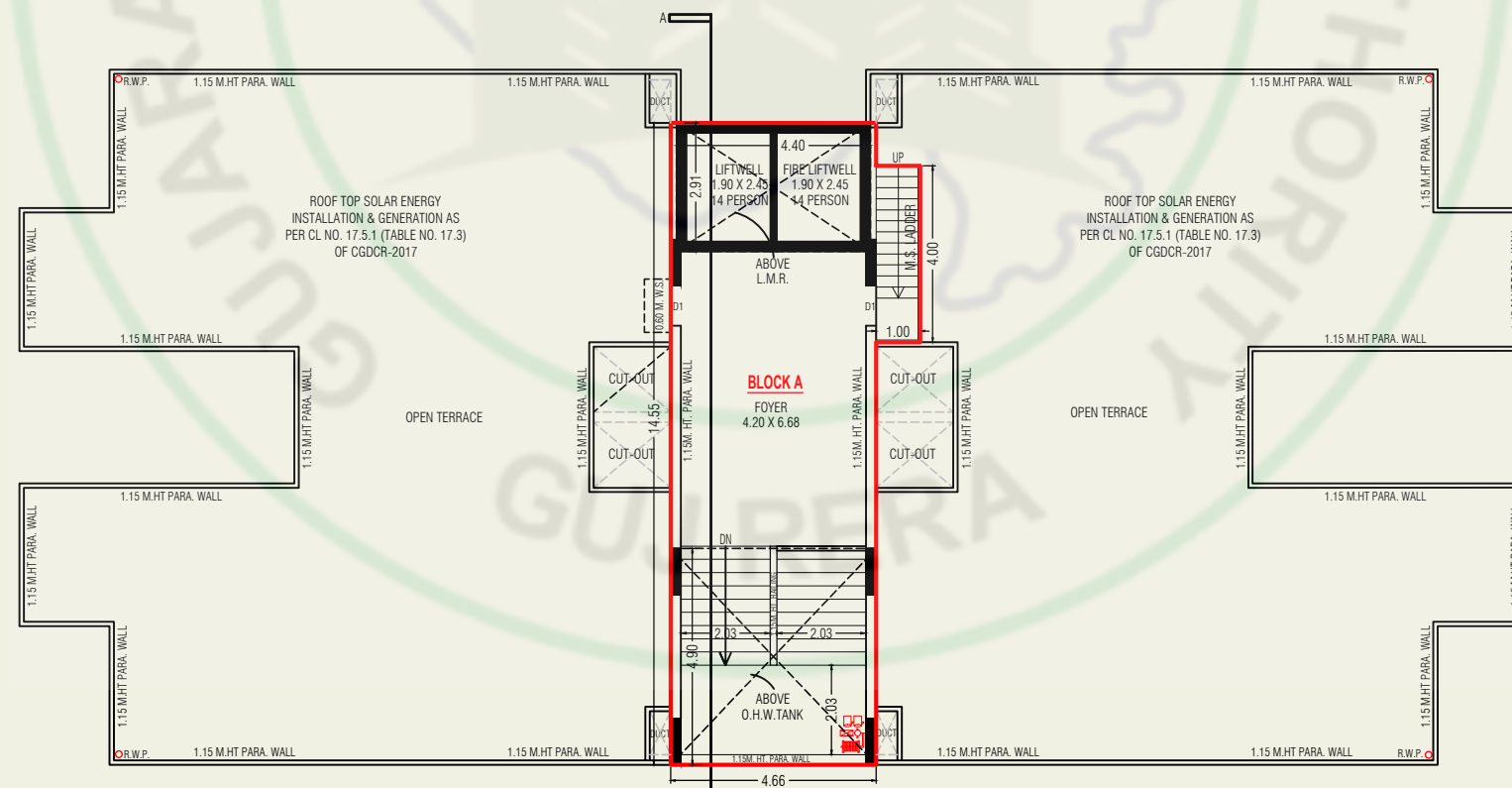
TERRACE FLOOR PLAN (BLOCK-A)
