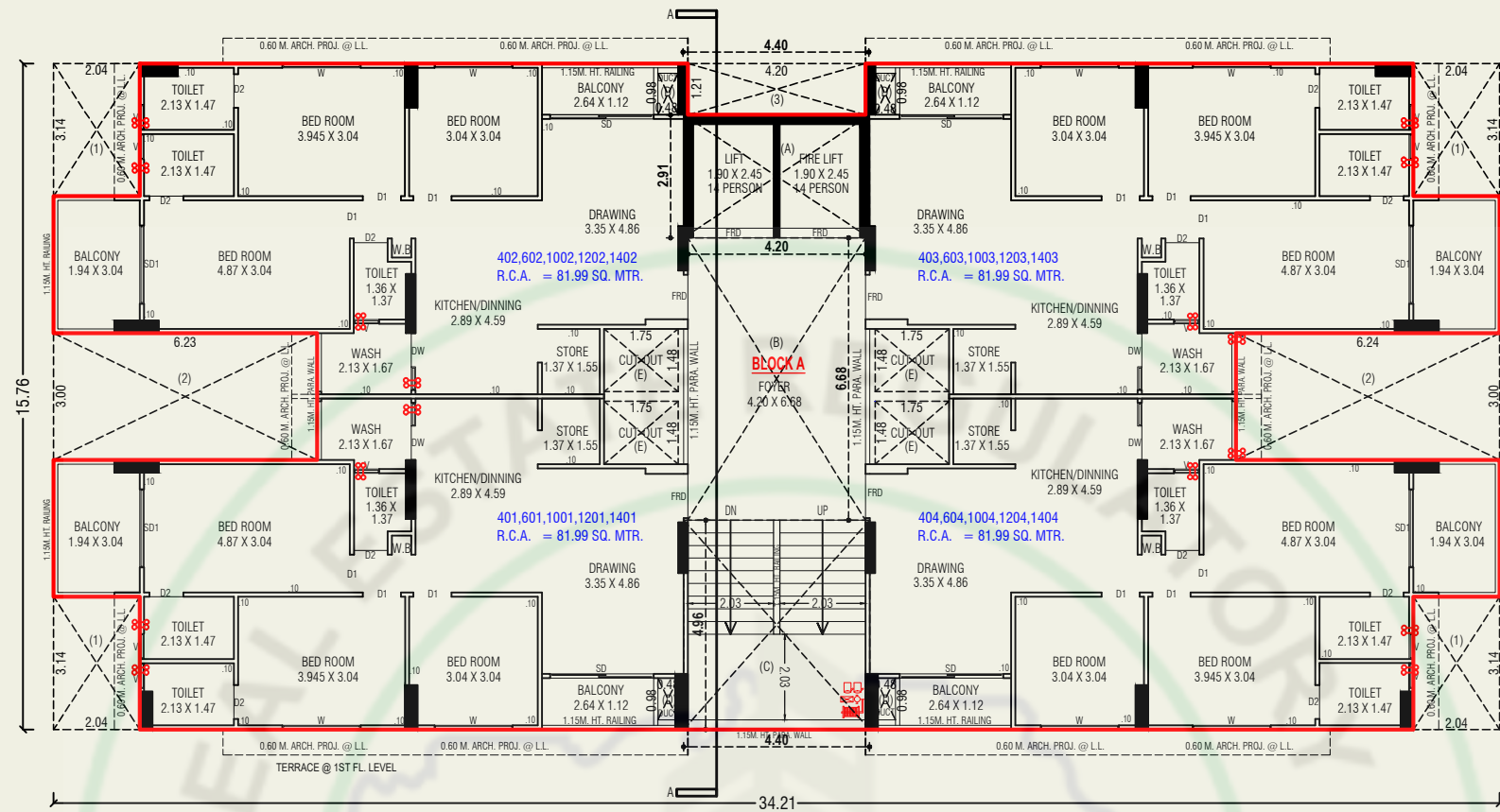
4TH, 6TH, 10TH, 12TH & 14TH FLOOR PLAN (BLOCK-A)
