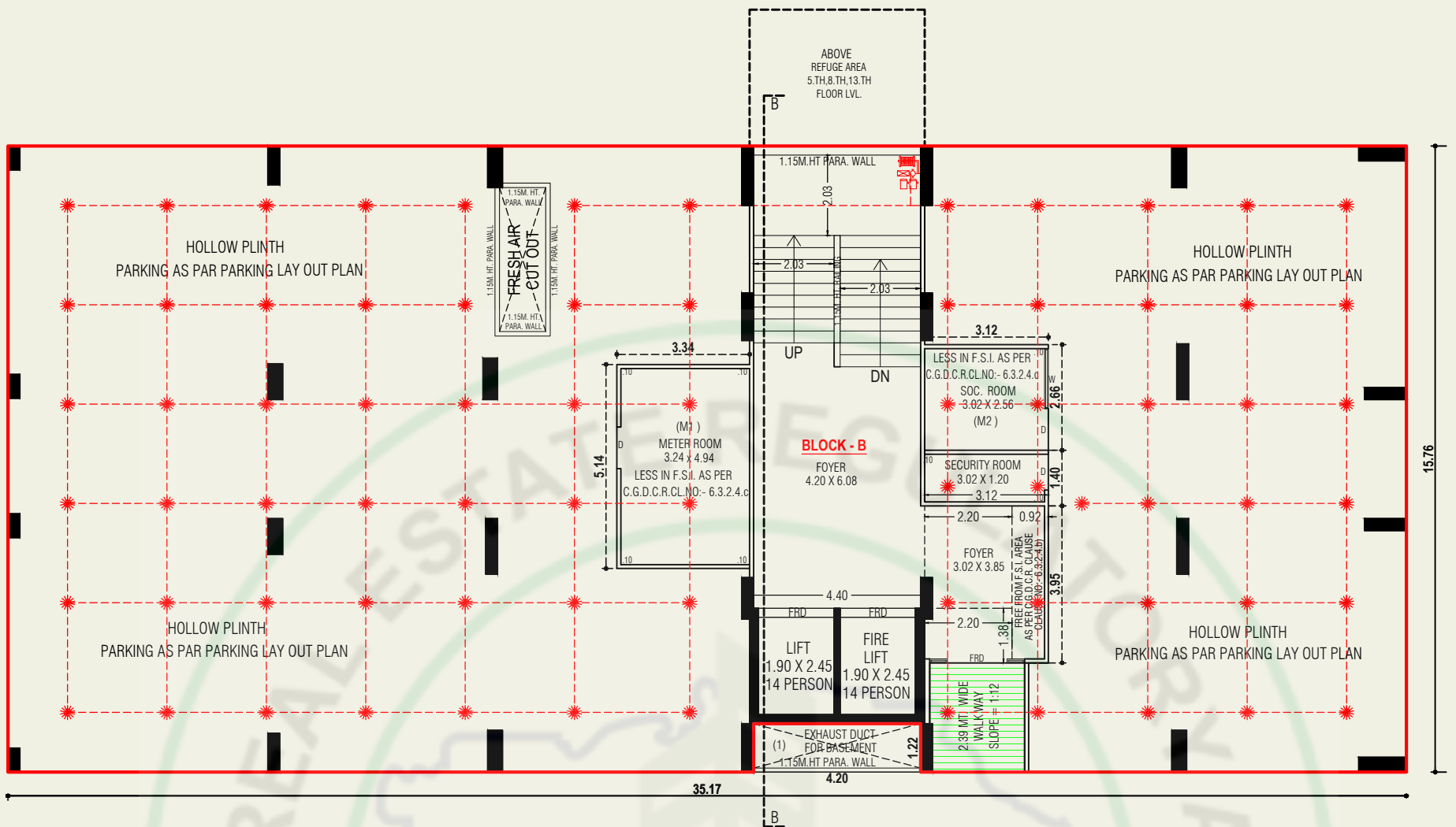
GROUND FLOOR PLAN (HOLLOW PLINTH) (BLOCK-B)
