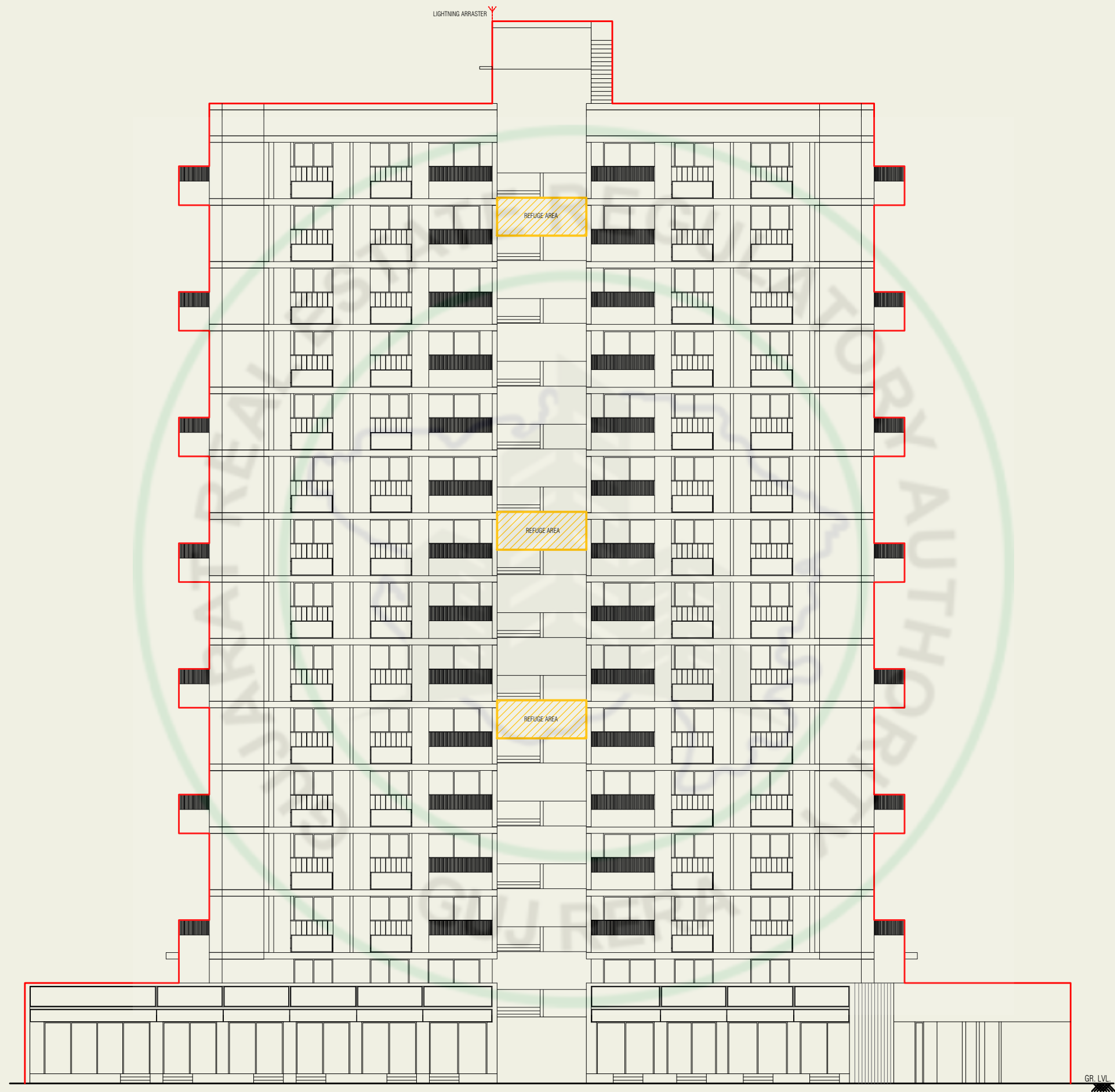
FRONT SIDE ELEVATION (BLOCK-A)
