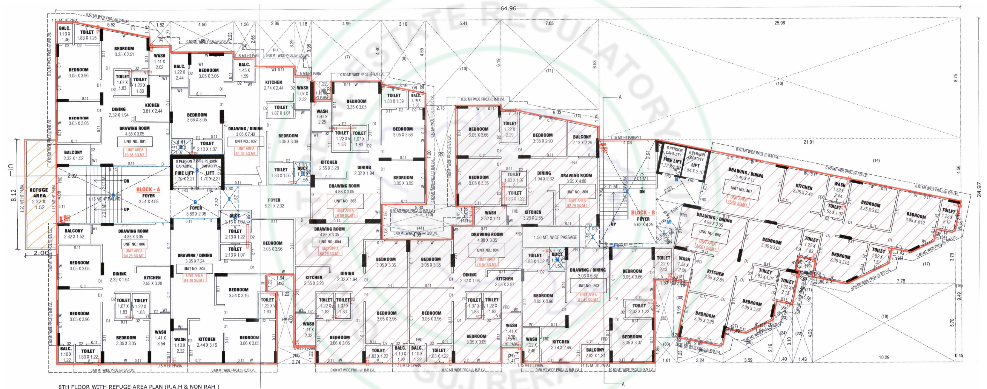
8TH FLOOR WITH REFUGE AREA PLAN (R.A.H & NON RAH)
