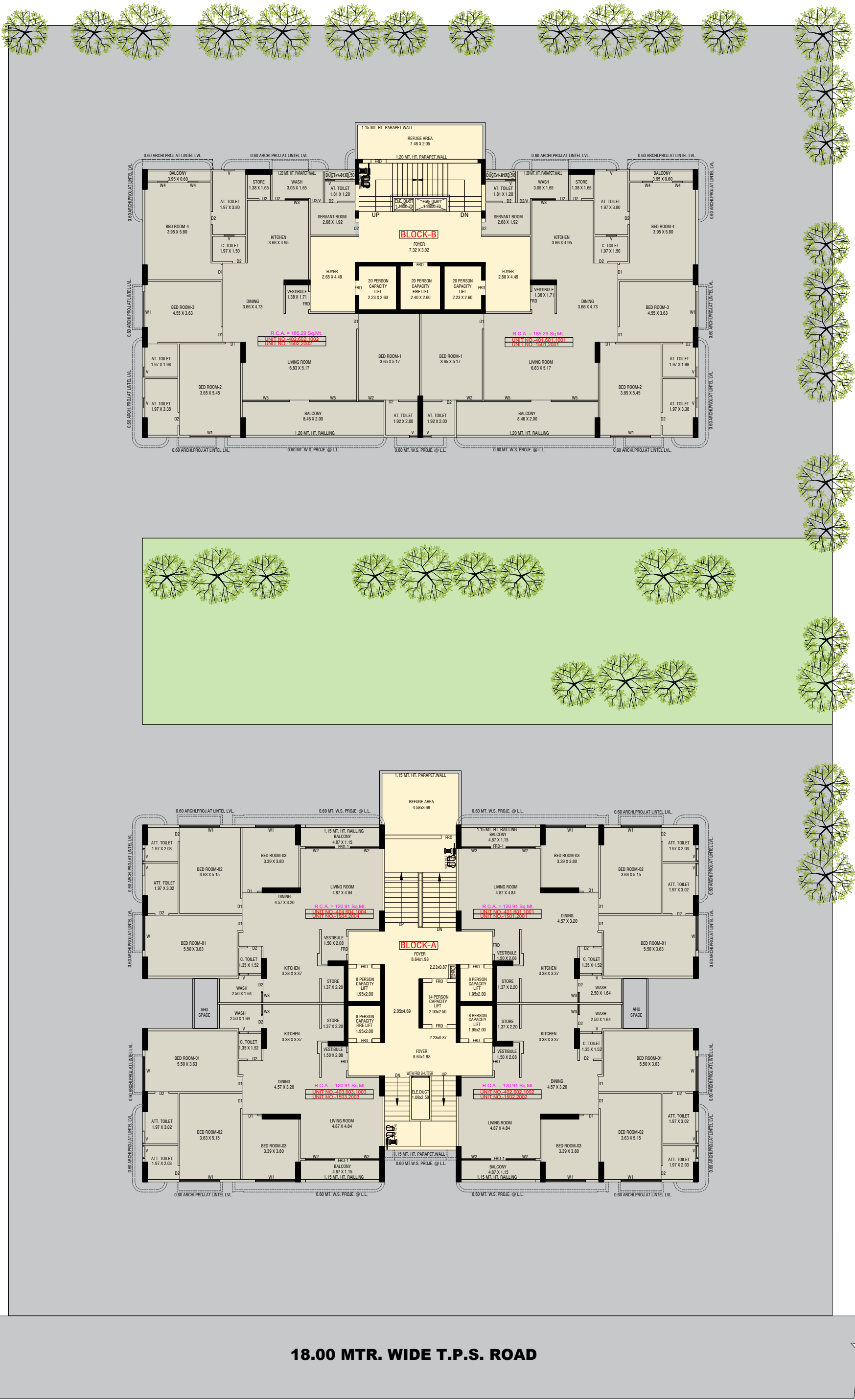
REFUGE FLOOR PLAN (5TH, 7TH, 11TH,16TH & 21ST FLOOR PLAN FLOOR)
