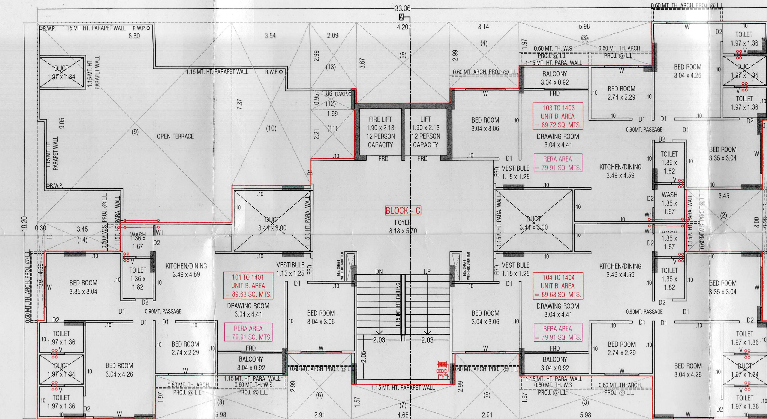
13TH FLOOR PLAN
