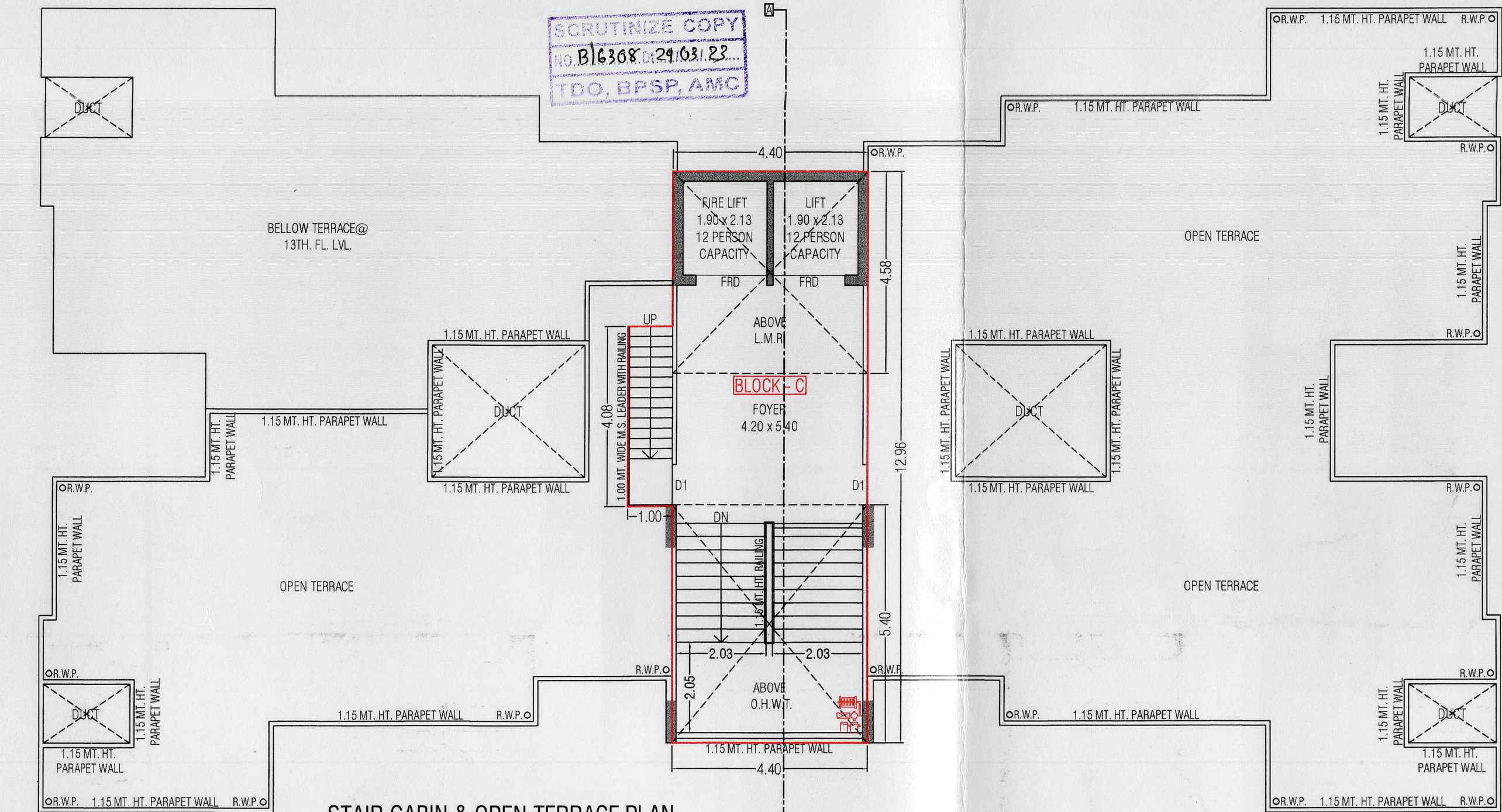
STAIR CABIN & OPEN TERRACE PLAN
