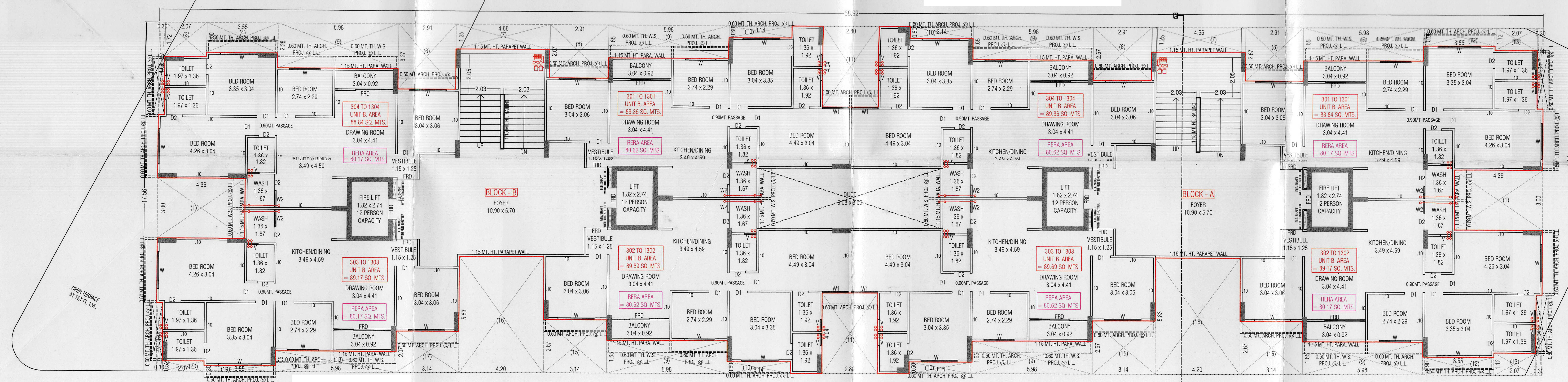
TYPICAL FLOOR PLAN ( 3RD TO 13TH FLOOR PLAN )
