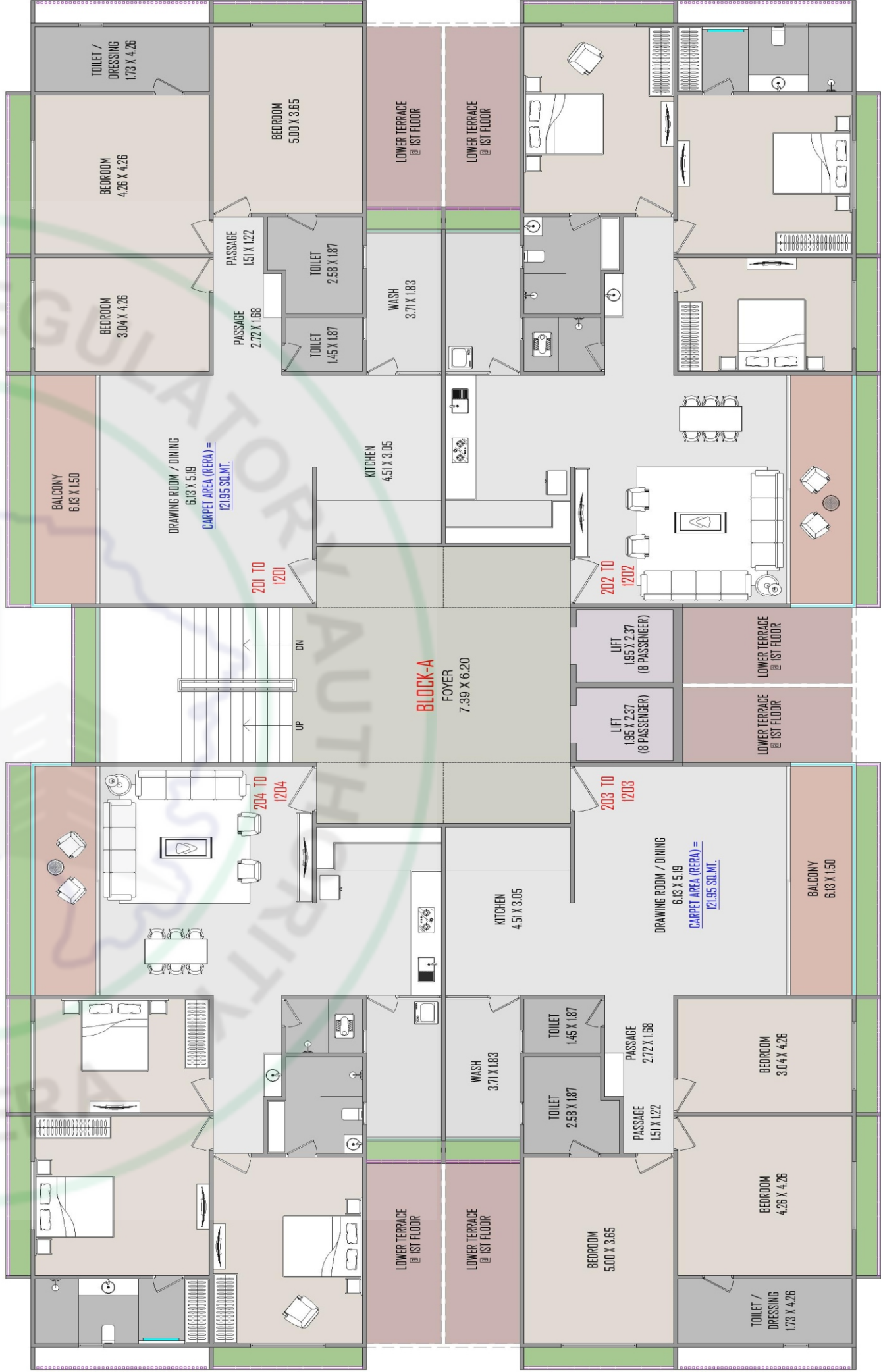
TYPICAL FLOOR PLAN ( 2ND TO 12TH ) :- BLOCK - A , B
