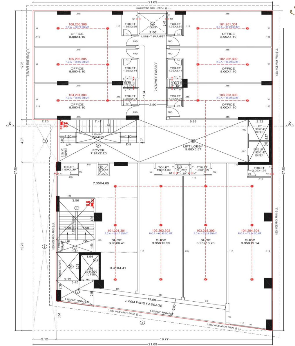
1 ST 2 ND 3 RD FLOOR PLAN
