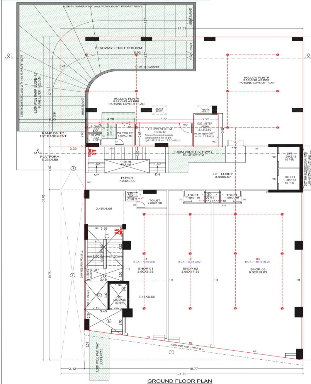
GF FLOOR PLAN
