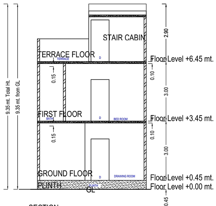
SECTION
