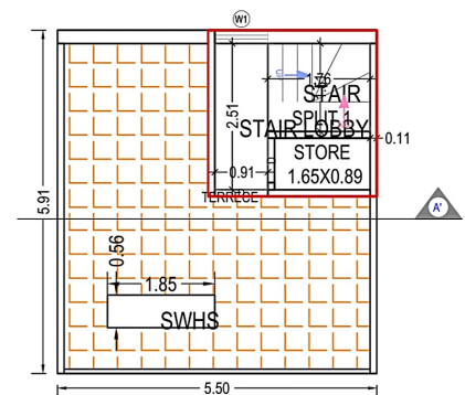
TERRACE FLOOR PLAN (Proposed) (SCALE 1:100)
