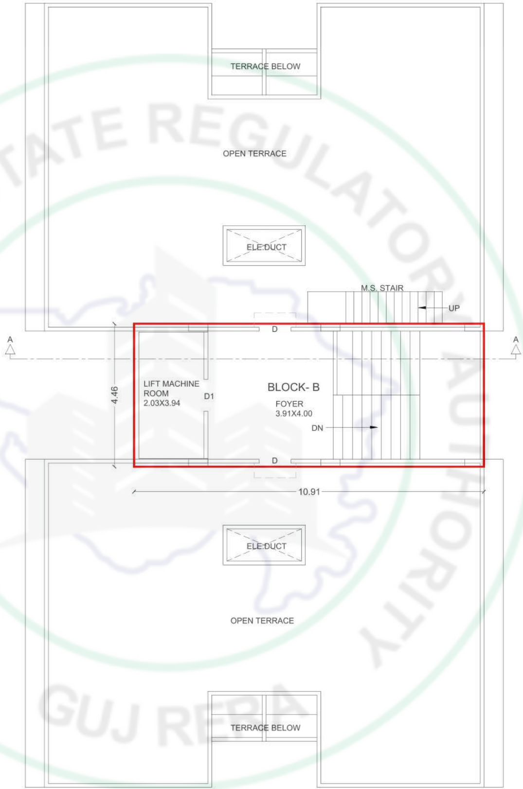
STAIR CABIN PLAN
