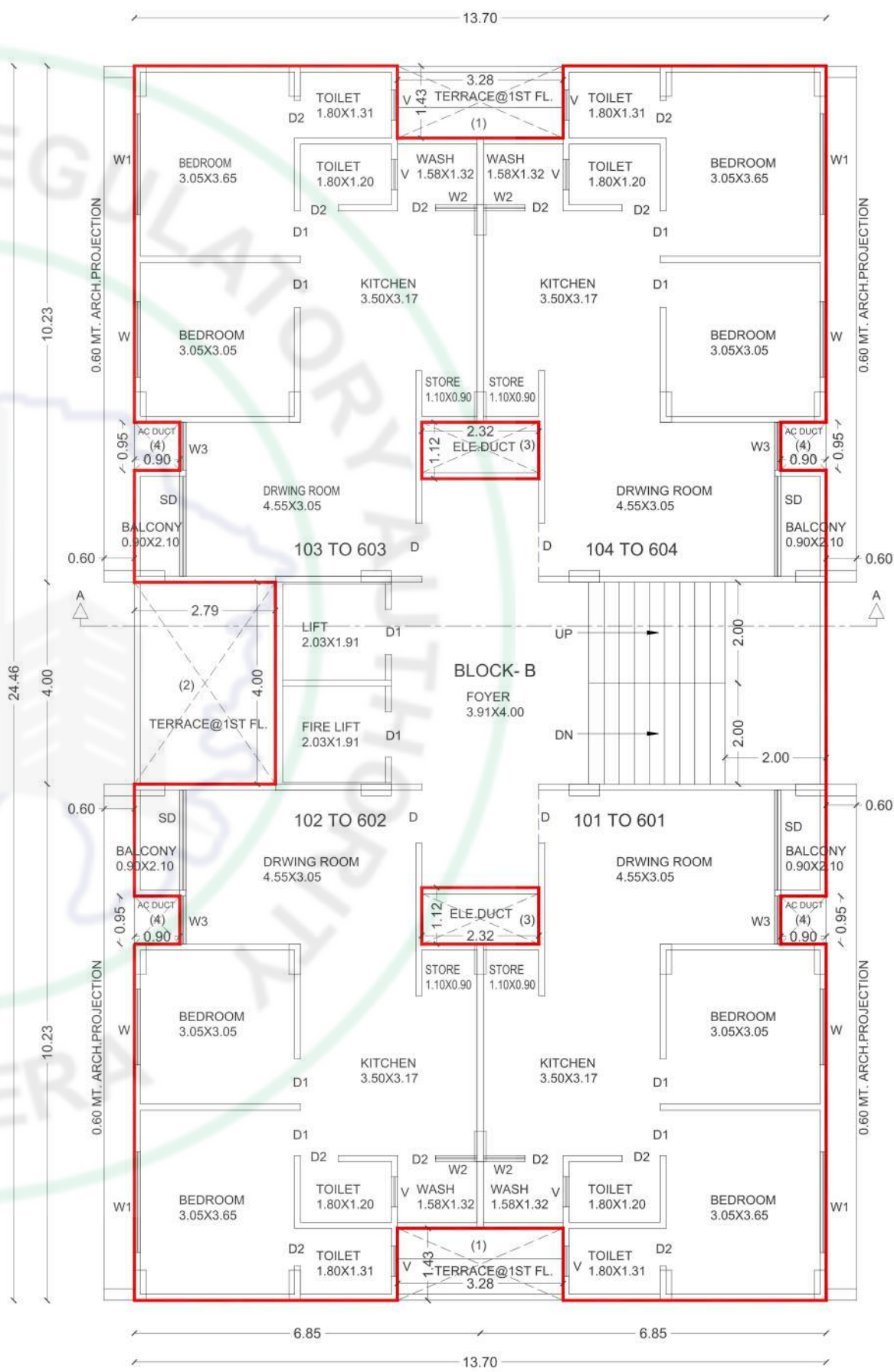
TYPICAL FLOOR PLAN 1ST TO 6TH FLOOR)
