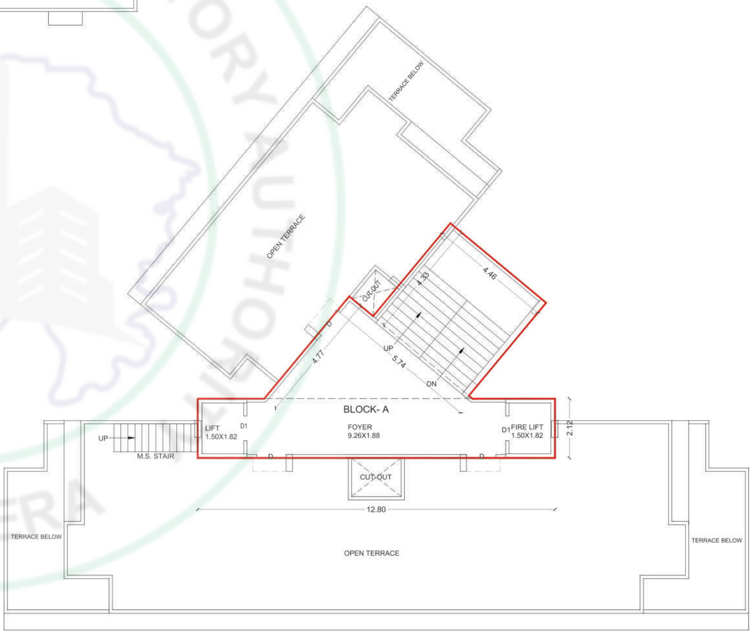
STAIR CABIN PLAN
