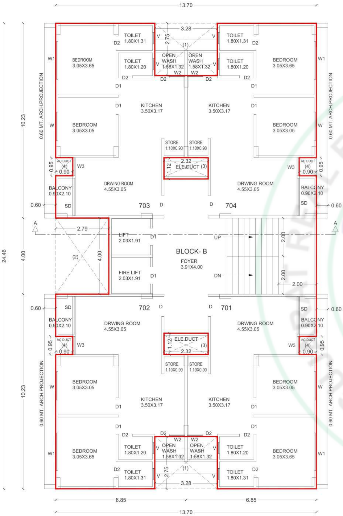
7TH FLOOR PLAN
