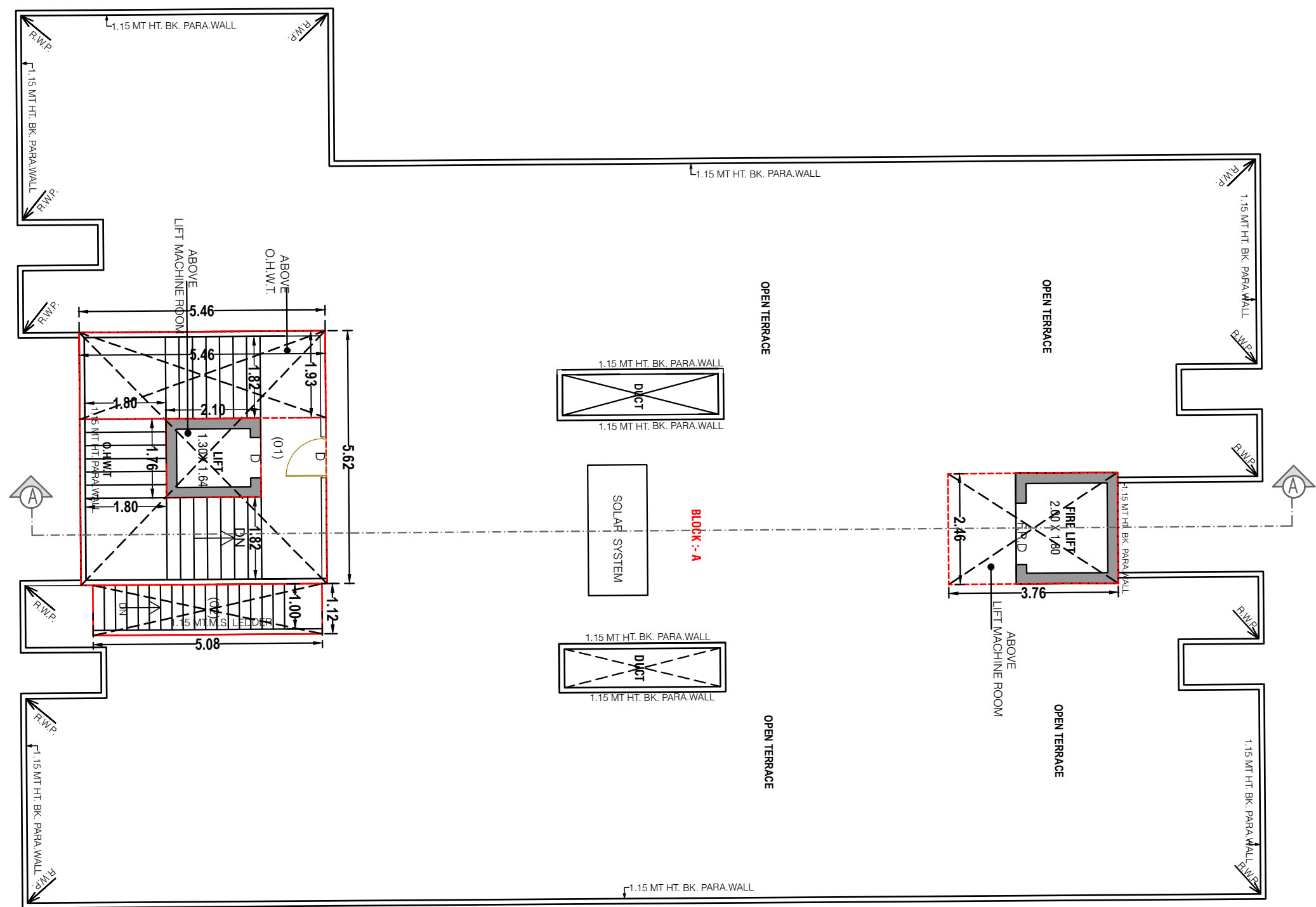
STAIR CABIN, LIFT MACHINE ROOM, O.H.W.T. & OPEN TERRACE PLAN (BLOCK -A)
