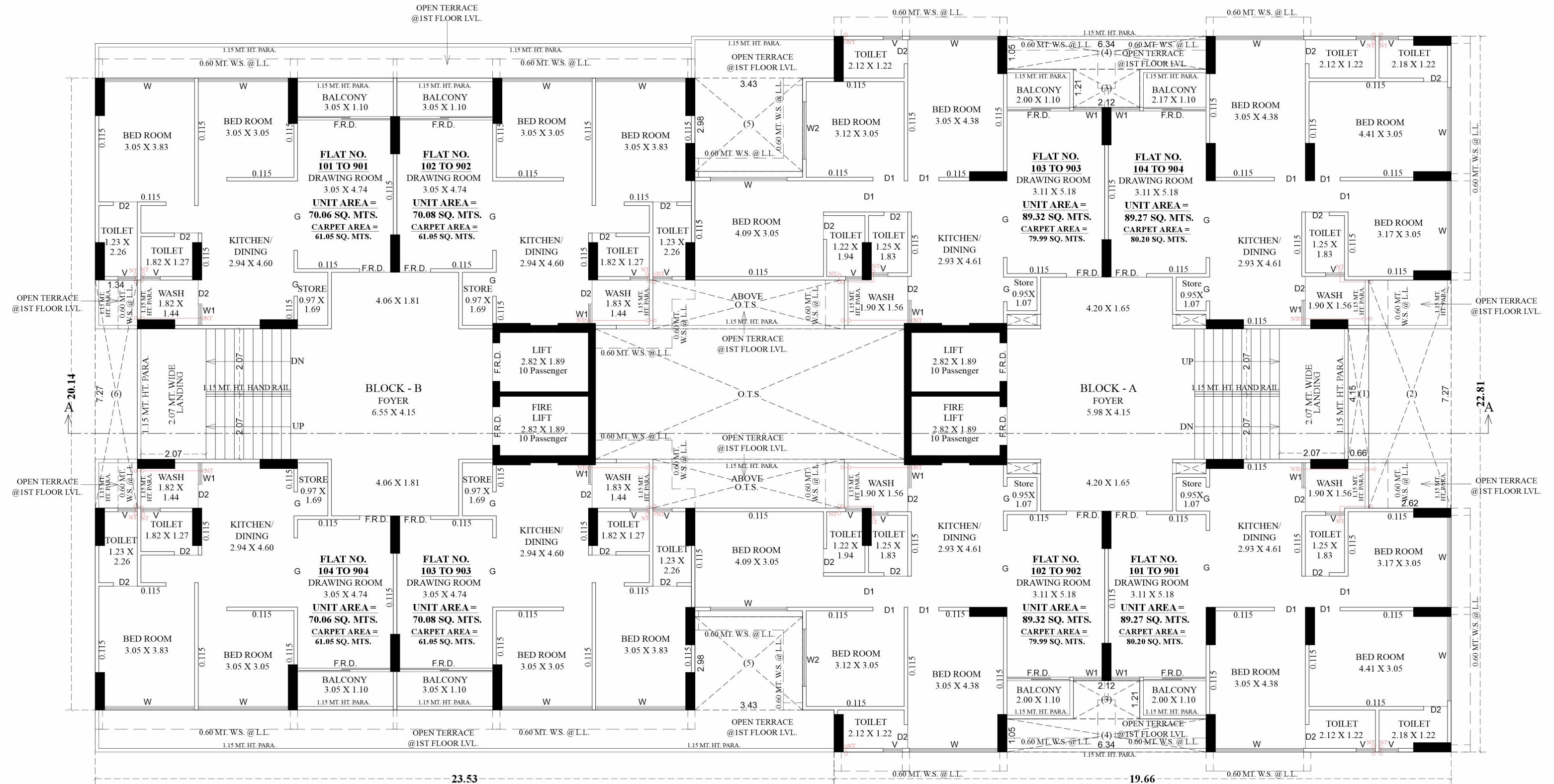
1ST TO 9TH FLOOR PLAN
