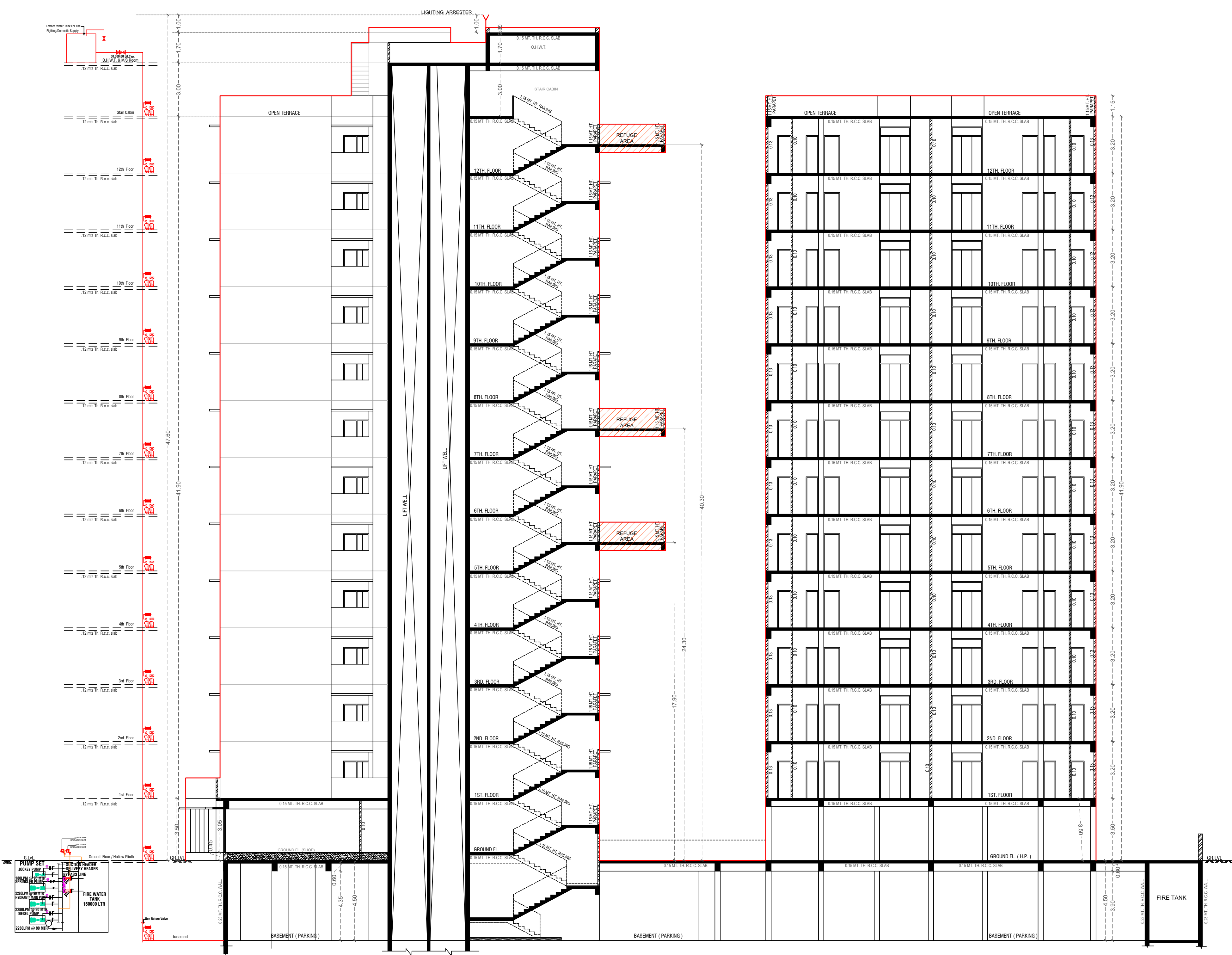
SECTION AT :- A'-B''
