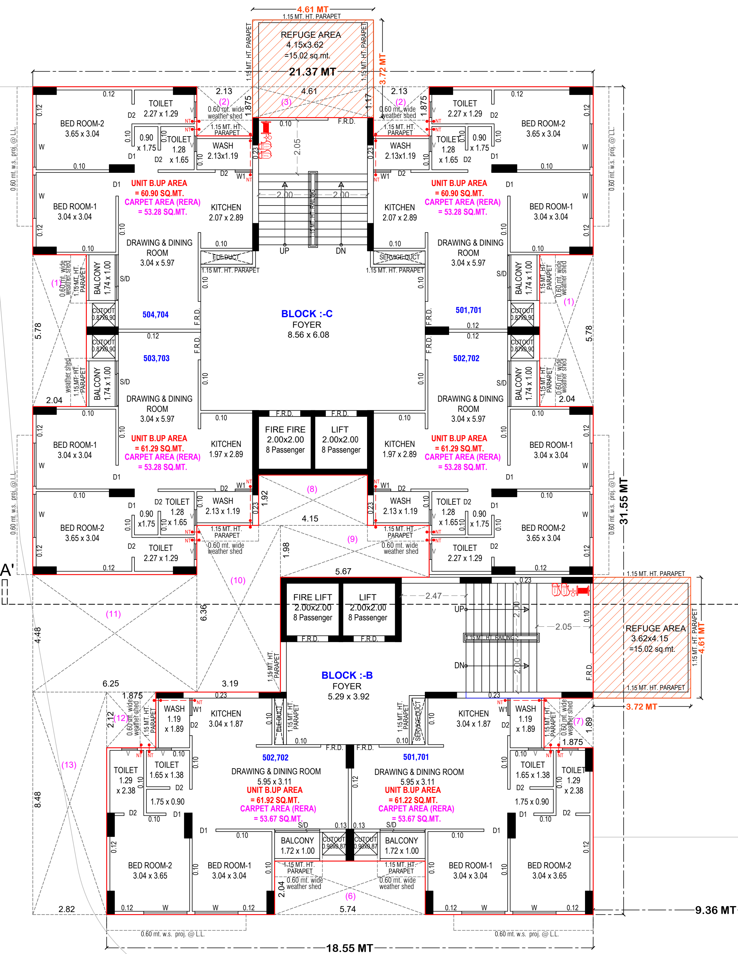
5th. FL. & 7th. FL. (REFUGE FL.) PLAN
