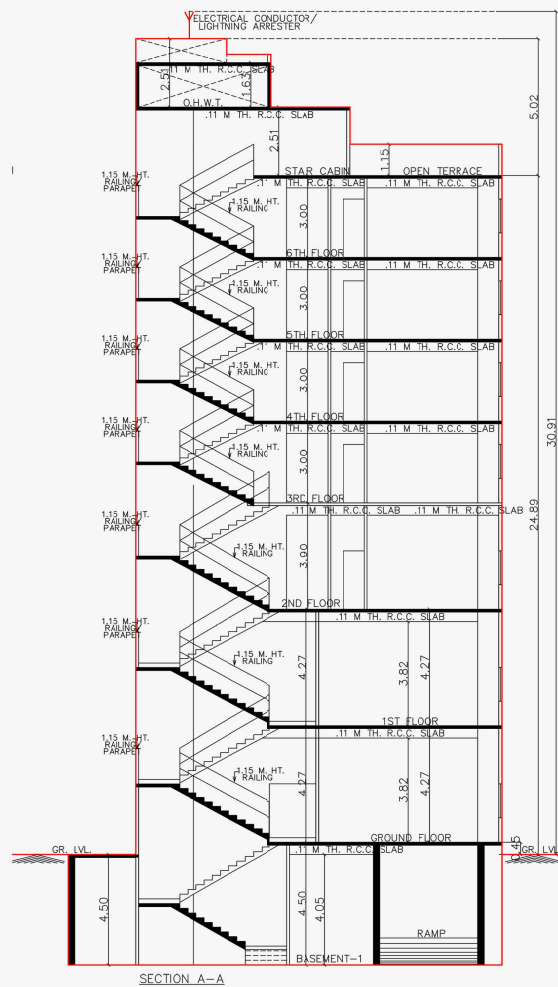
SECTION
