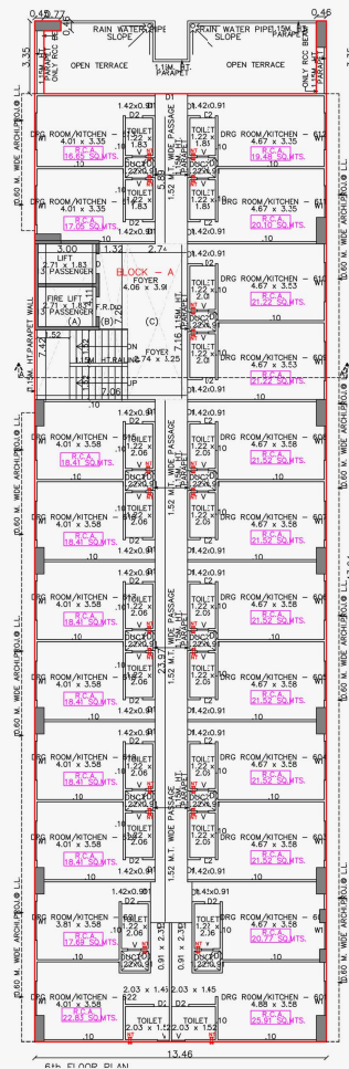
6TH FLOOR PLAN
