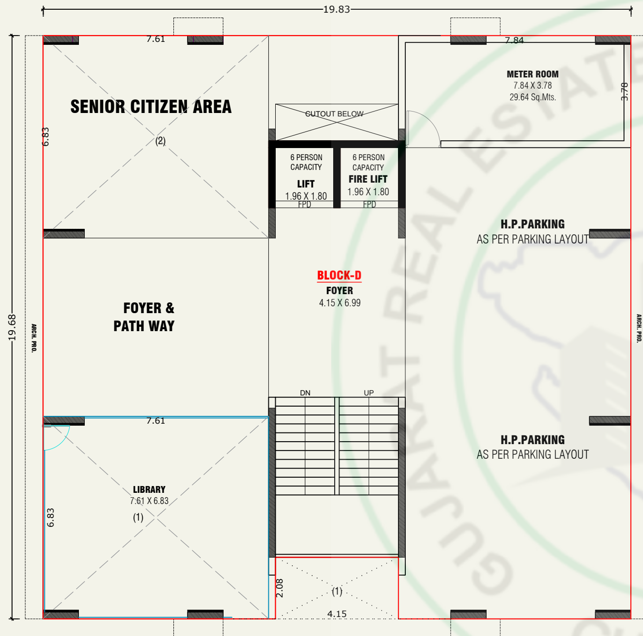
GROUND FLOOR PLAN (BLOCK-D)
