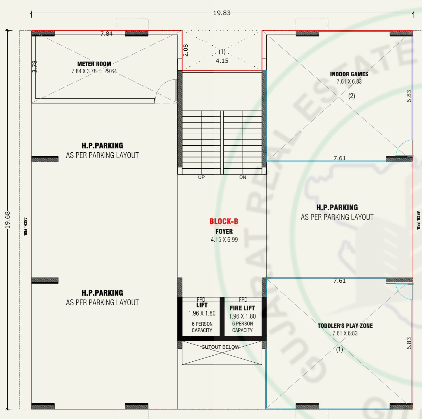
GROUND FLOOR PLAN (BLOCK-B)
