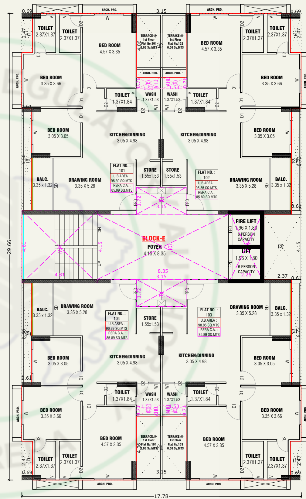
1st FLOOR PLAN (BLOCK-E)
