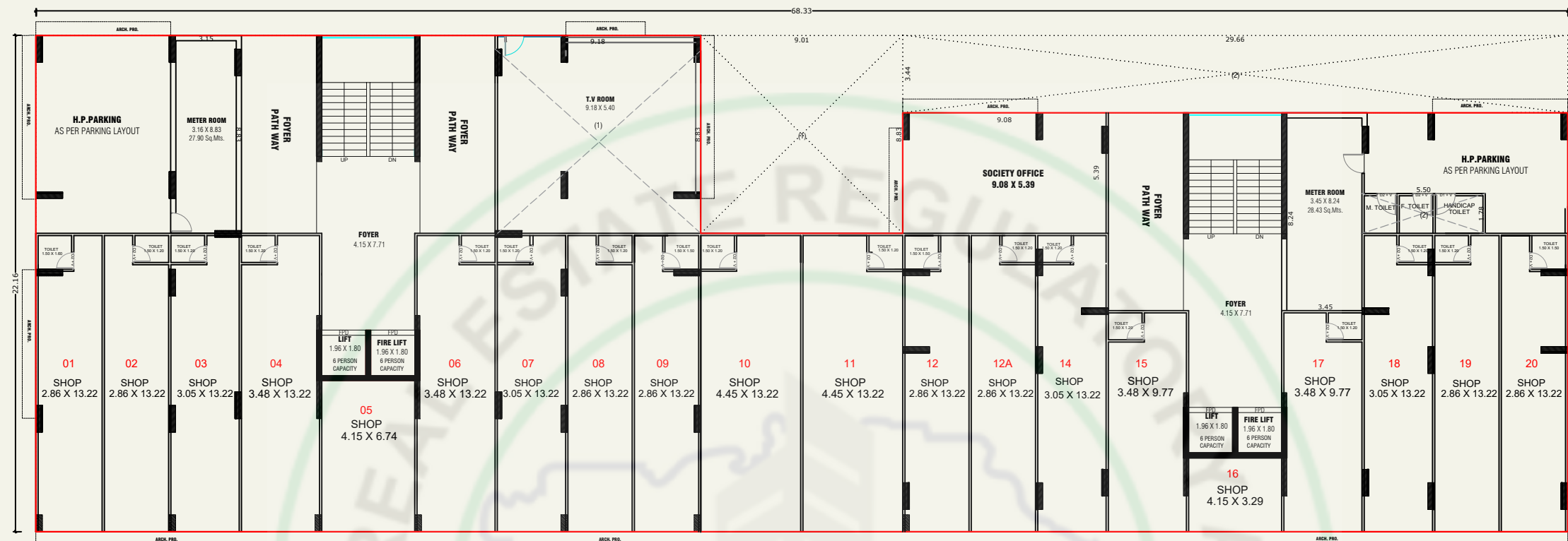
GROUND FLOOR PLAN (S.P.+ H.P.) (BLOCK-A+F)
