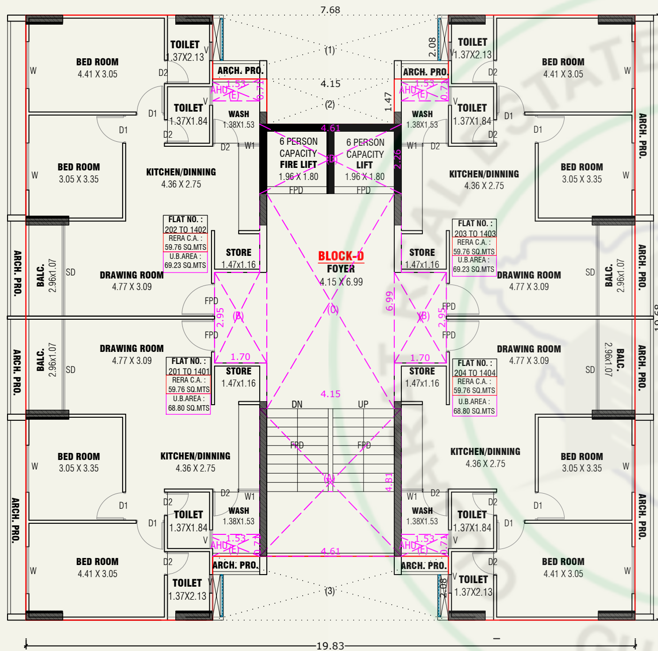
TYPICAL FLOOR PLAN (2nd TO 14th FLOOR PLAN) (BLOCK-D)
