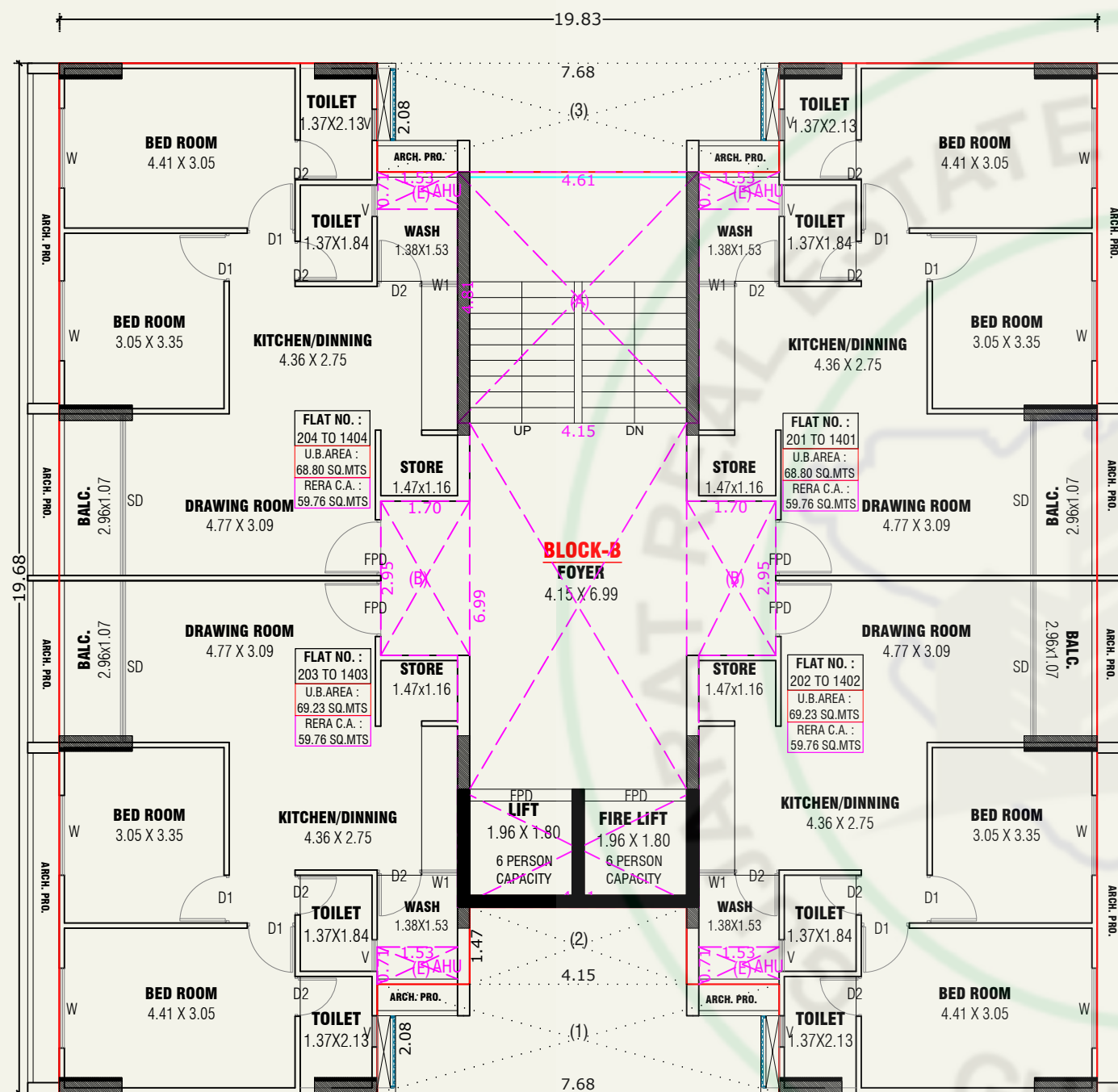
TYPICAL FLOOR PLAN (2nd TO 14th FLOOR PLAN) (BLOCK-B)
