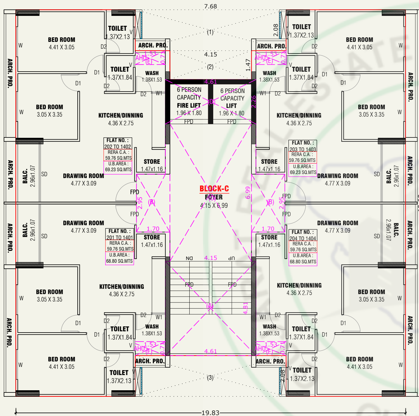
TYPICAL FLOOR PLAN (2nd TO 14th FLOOR PLAN) (BLOCK-C)
