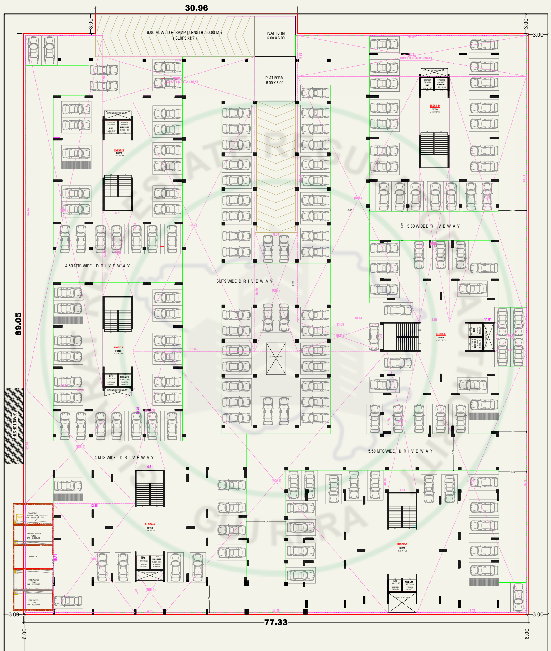
BASEMENT-1 PLAN
