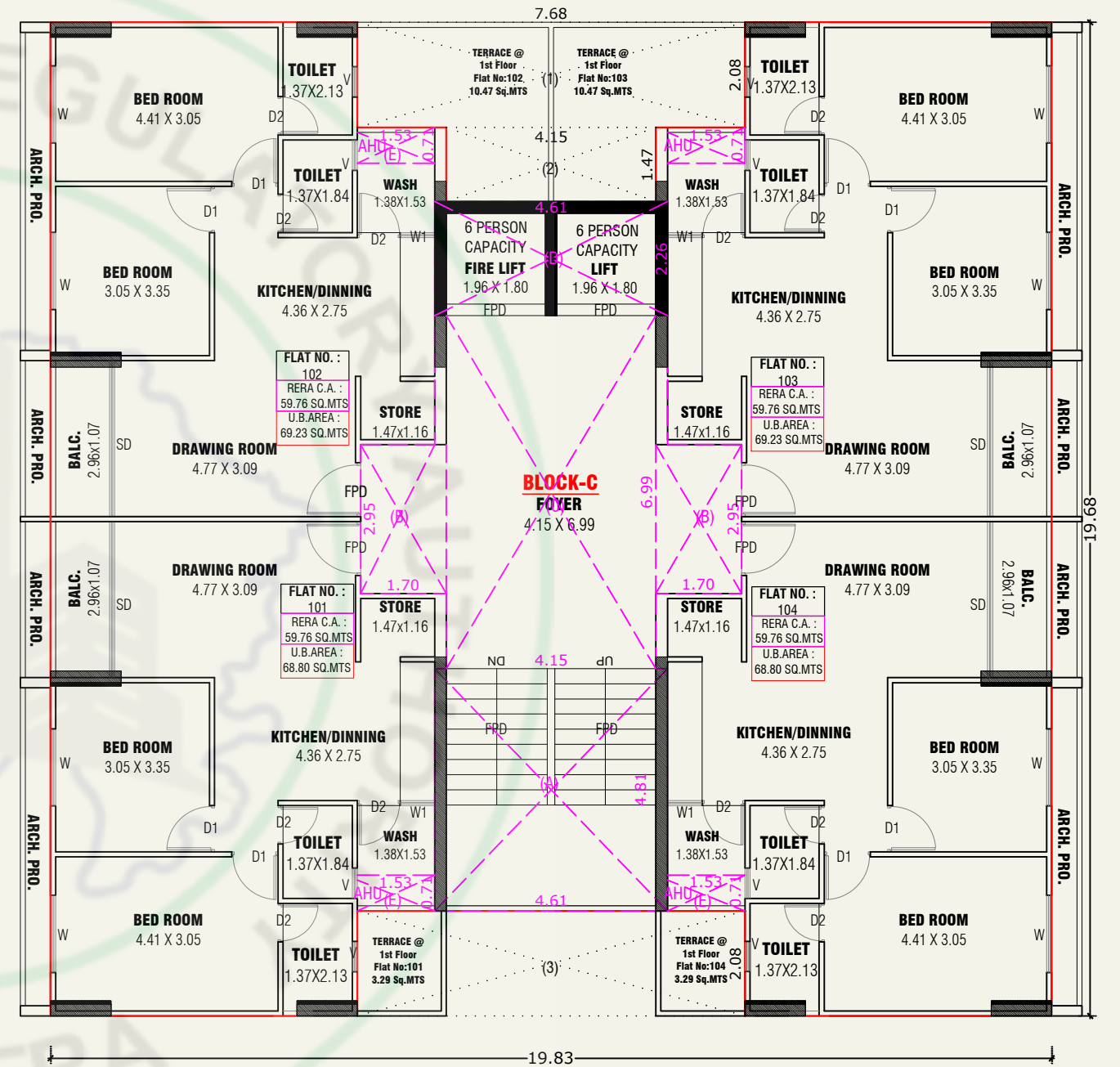
1st FLOOR PLAN (BLOCK-C)
