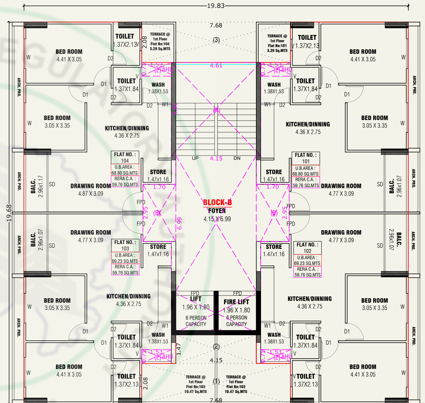
1st FLOOR PLAN (BLOCK-B)
