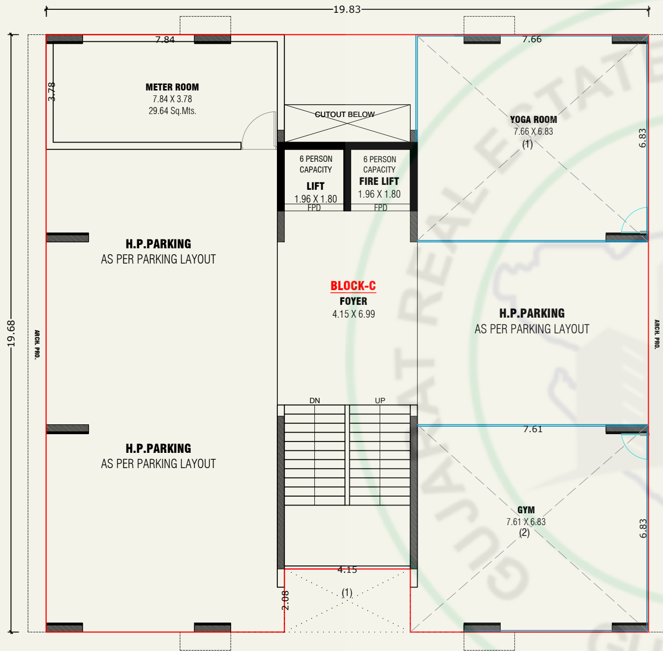
GROUND FLOOR PLAN (BLOCK-C)
