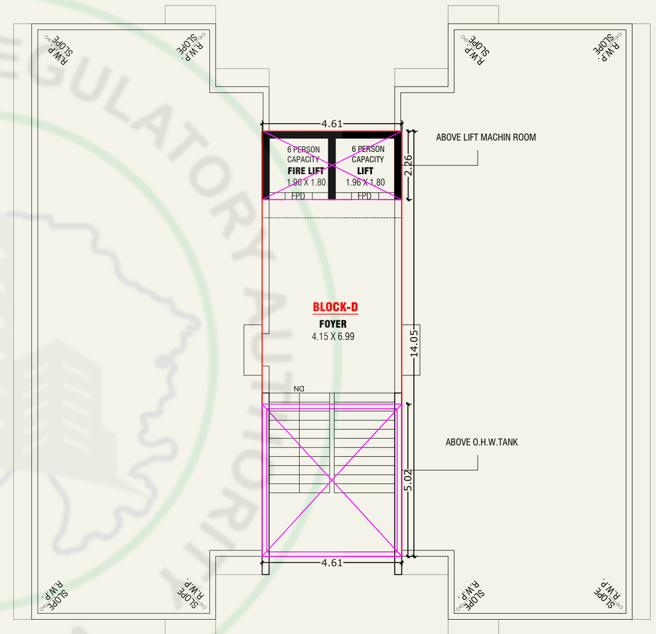
TERRACE + STAIR CABIN PLAN (BLOCK-D)
