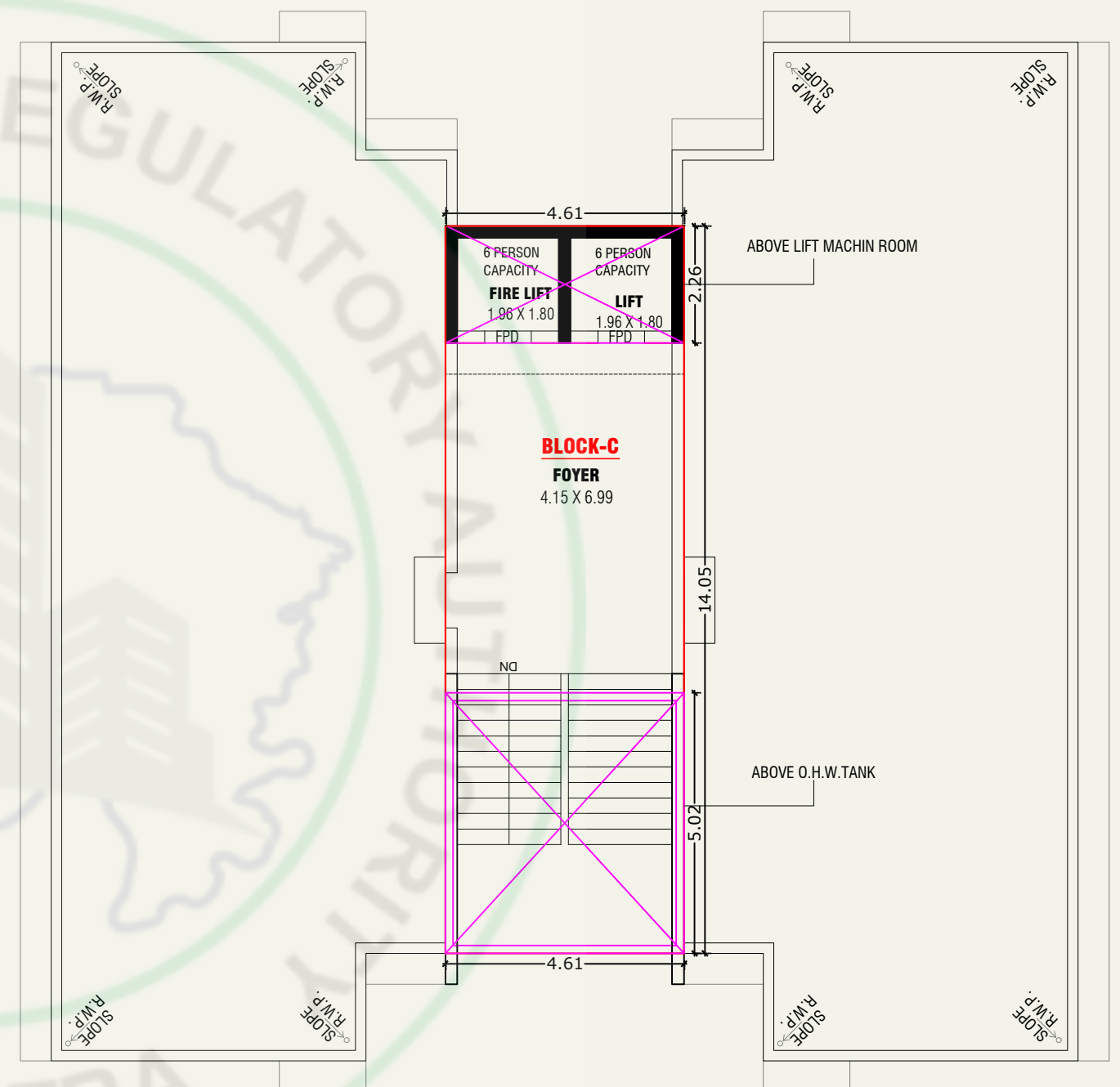
TERRACE + STAIR CABIN PLAN (BLOCK-C)
