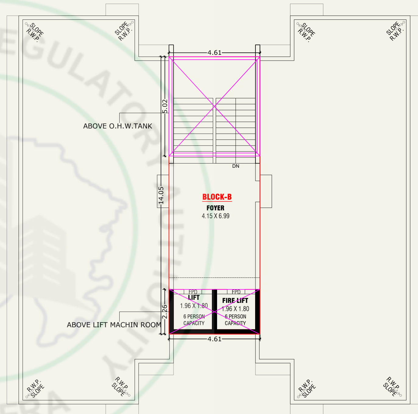
TERRACE + STAIR CABIN PLAN (BLOCK-B)
