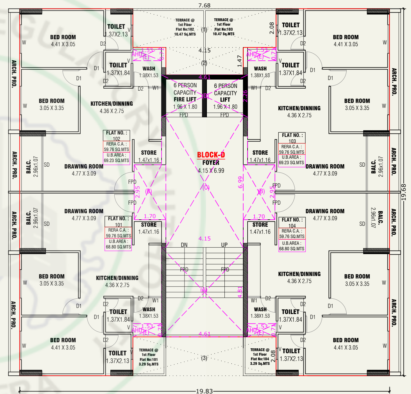
1st FLOOR PLAN (BLOCK-D)
