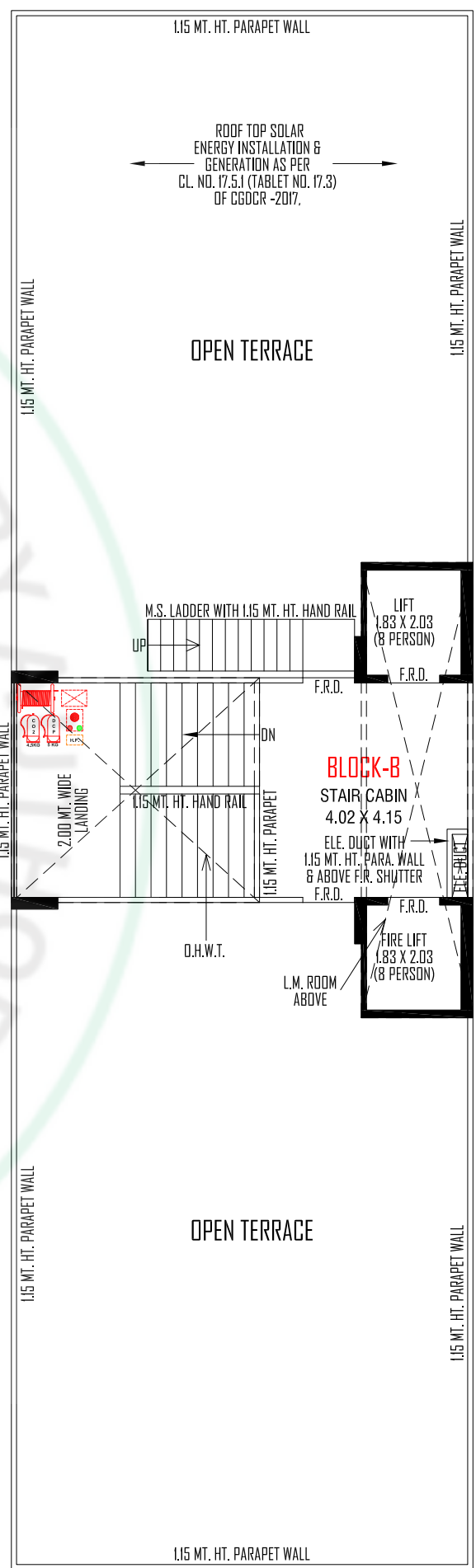
OPEN TERRACE PLAN WITH STAIR CABIN, LIFT MACHINE ROOM & O.H.W.T. ( BLOCK:- B )
