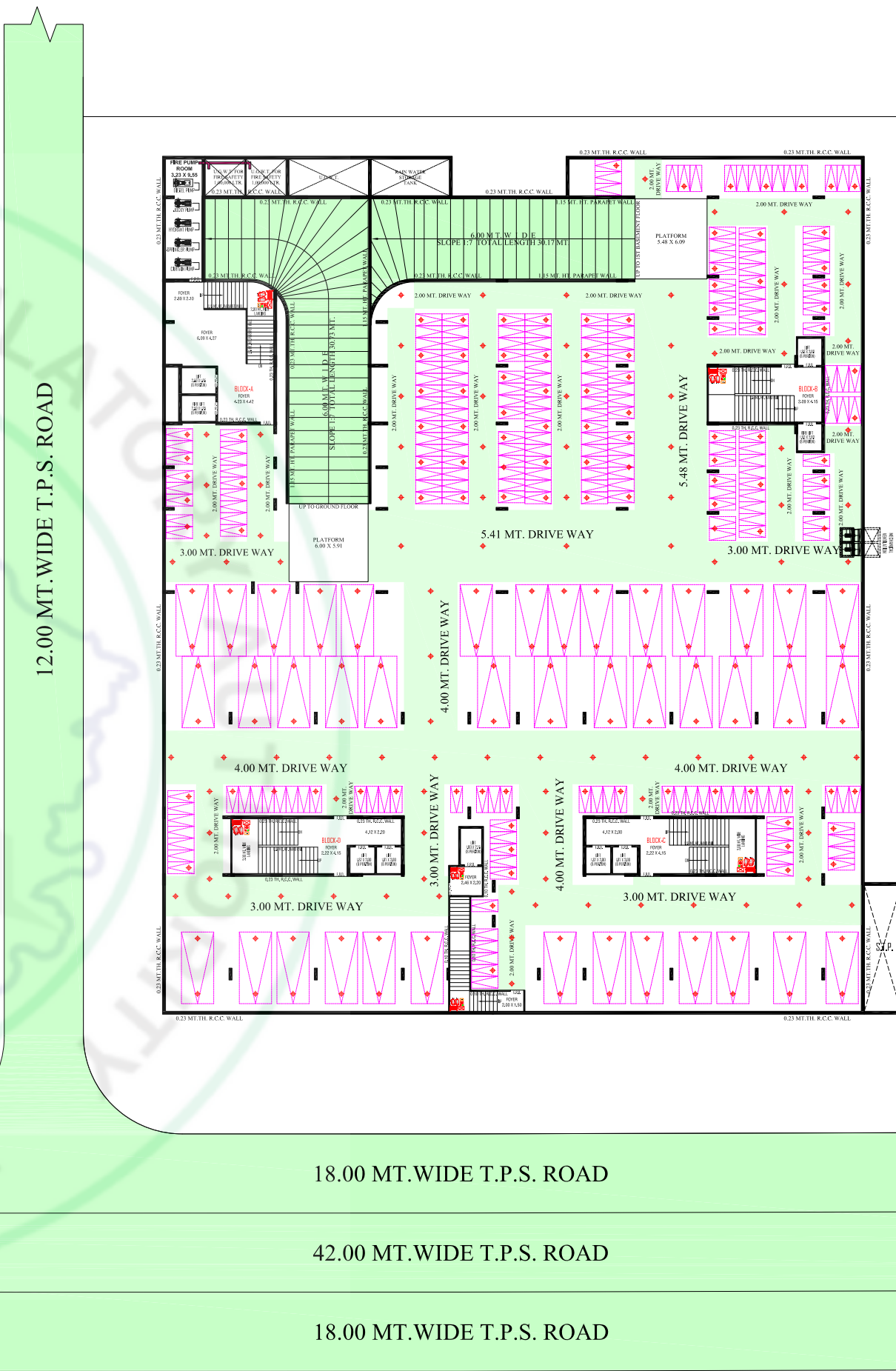
1ST BASEMENT FLOOR PLAN WITH PARKING LAY OUT [SCALE :- 1.00 CM. = 2.00 MT.]
