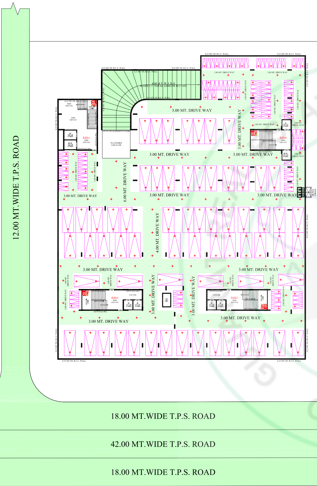
2ND BASEMENT FLOOR PLAN WITH PARKING LAY OUT [SCALE :- 1.00 CM. = 2.00 MT.]
