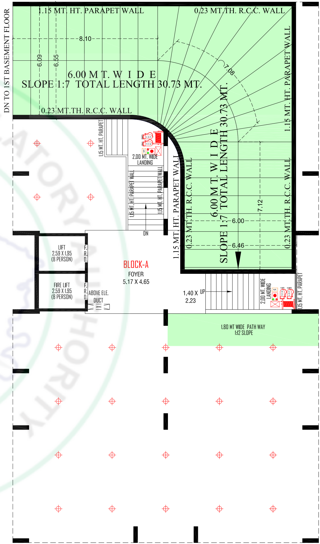
GROUND FLOOR PLAN (HOLLOW PLINTH) BLOCK:- A
