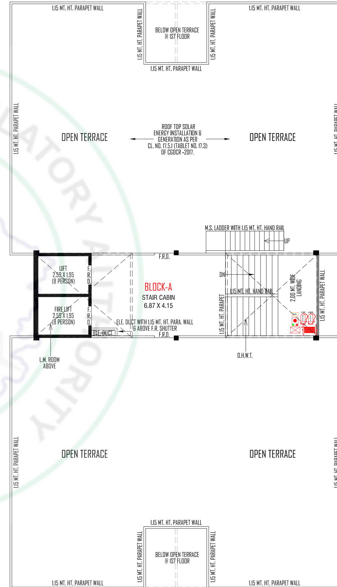
OPEN TERRACE PLAN WITH STAIR CABIN, LIFT MACHINE ROOM & O.H.W.T. ( BLOCK:- A )
