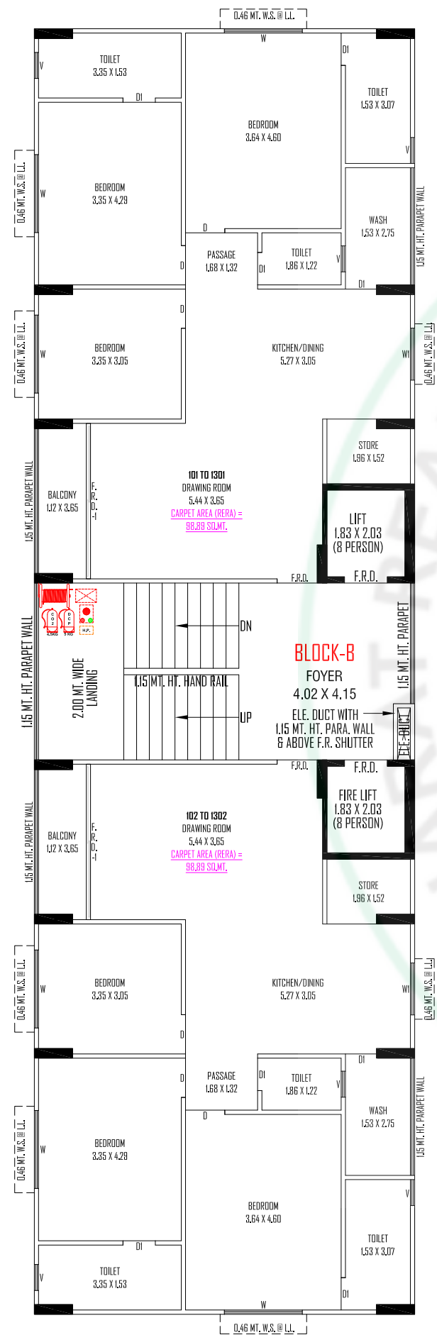
1ST FLOOR TO 13TH FLOOR PLAN ( BLOCK:- B )
