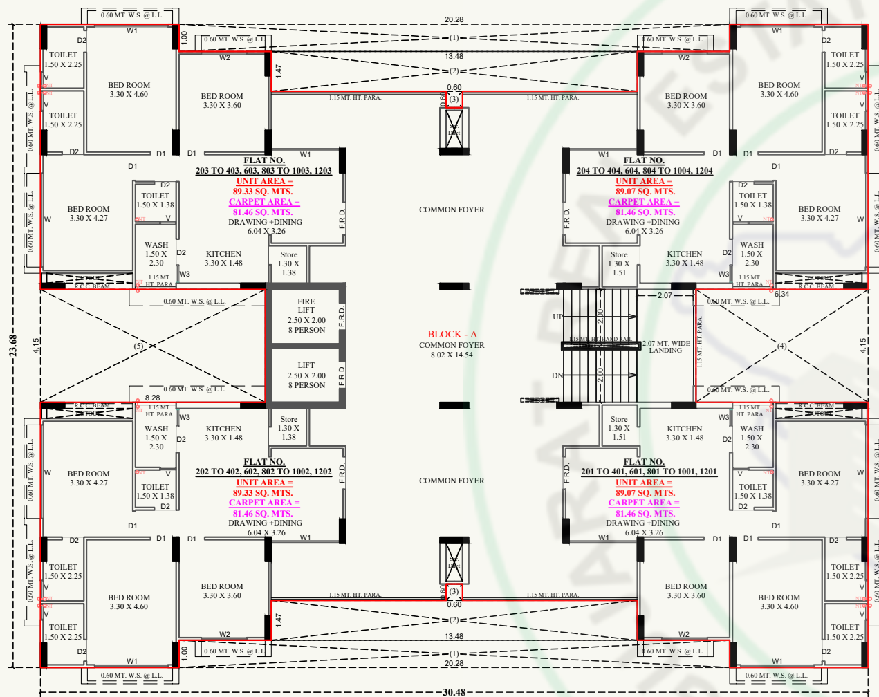
2ND TO 4TH, 6TH, 8TH TO 10TH, 12TH FLOOR PLAN
