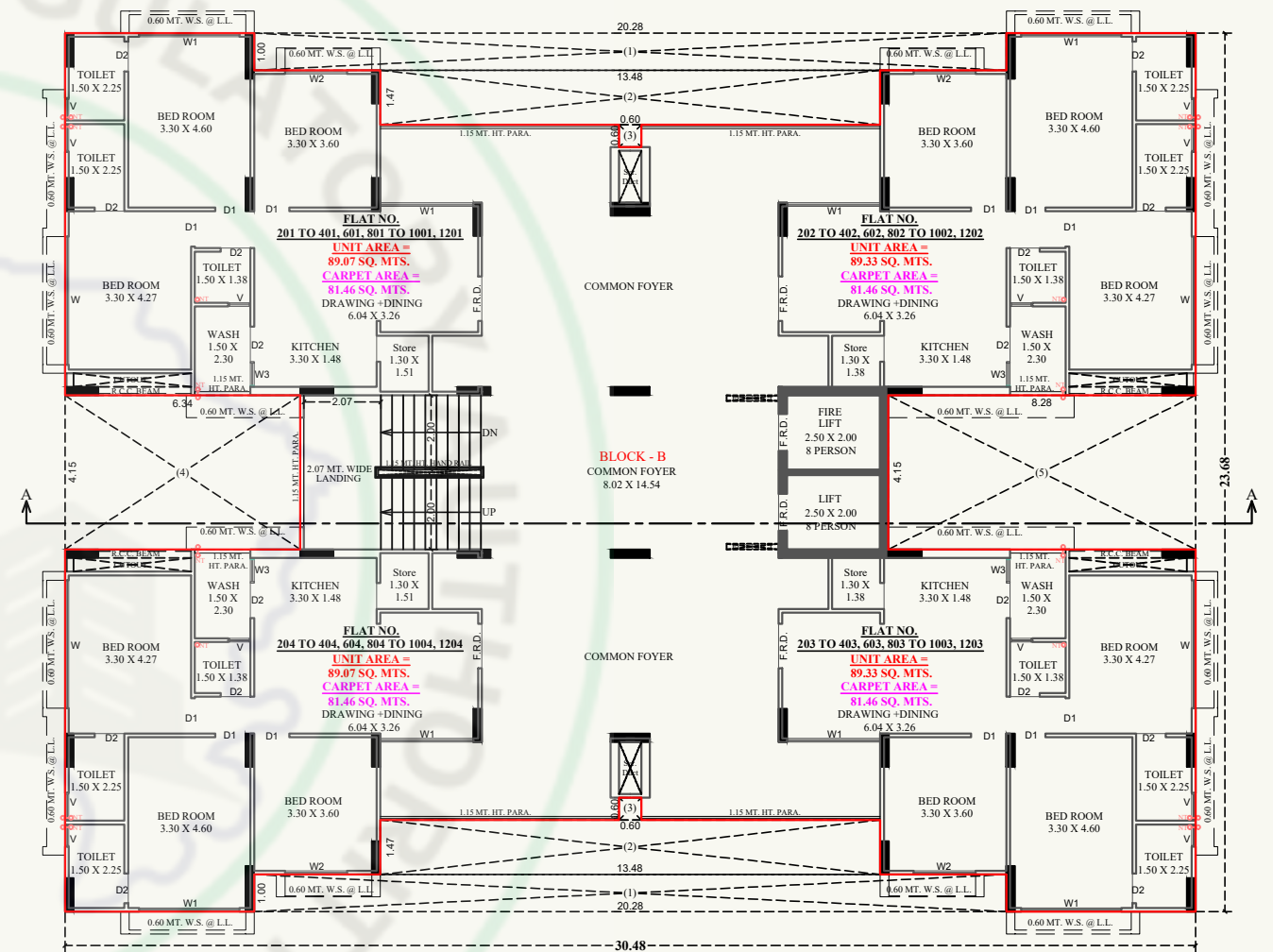
2ND TO 4TH, 6TH, 8TH TO 10TH, 12TH FLOOR PLAN
