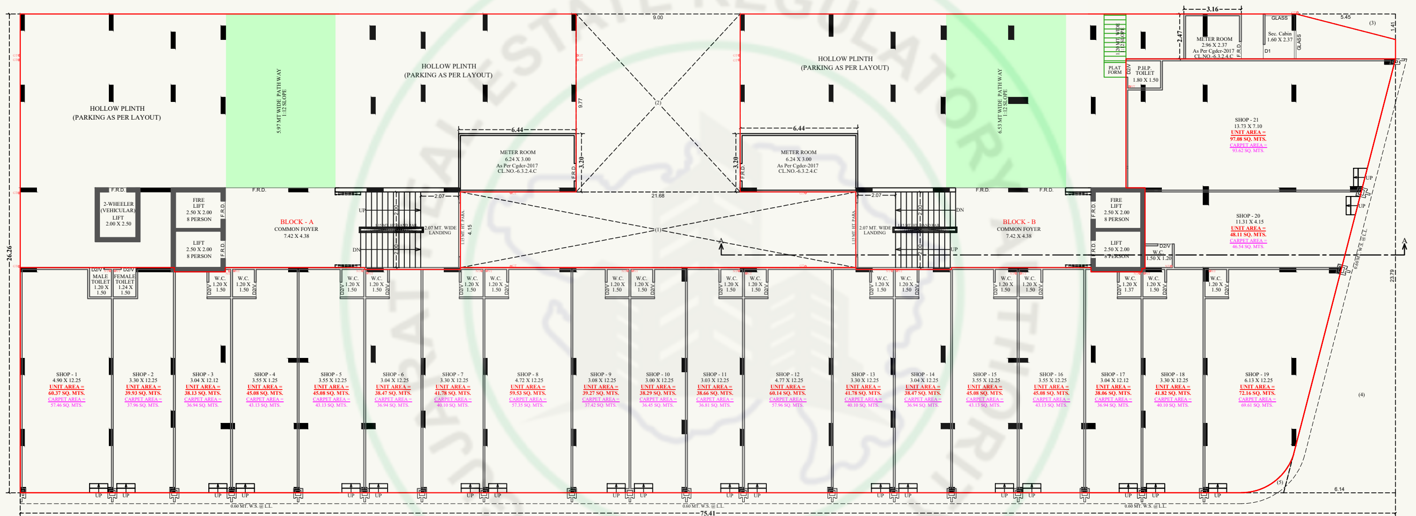
GROUND FLOOR PLAN (HOLLOW PLINTH+SOLID PLINTH)
