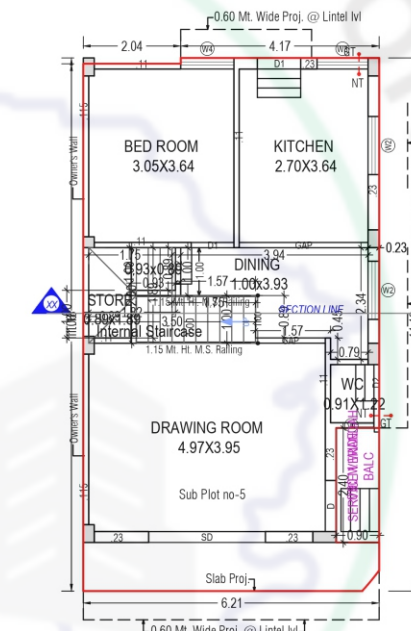
GROUND FLOOR PLAN (Proposed) (SCALE 1:100)
