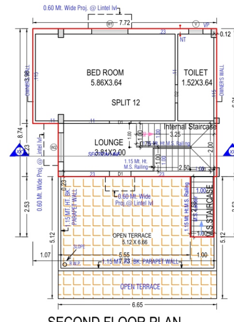
SECOND FLOOR PLAN (Proposed) (SCALE 1:100)
