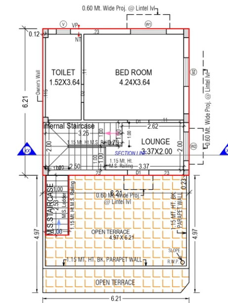
SECOND FLOOR PLAN (Proposed) (SCALE 1:100)
