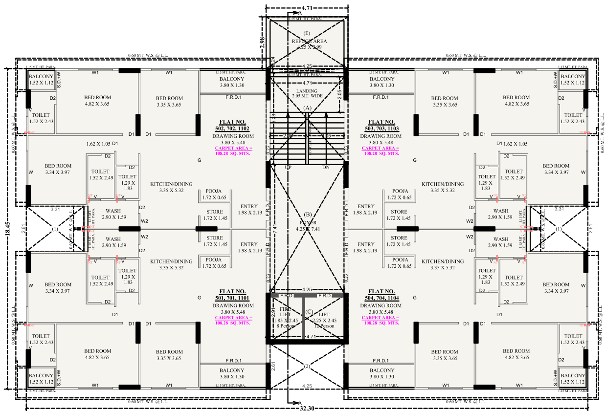
5TH, 7TH & 11TH FLOOR PLAN
