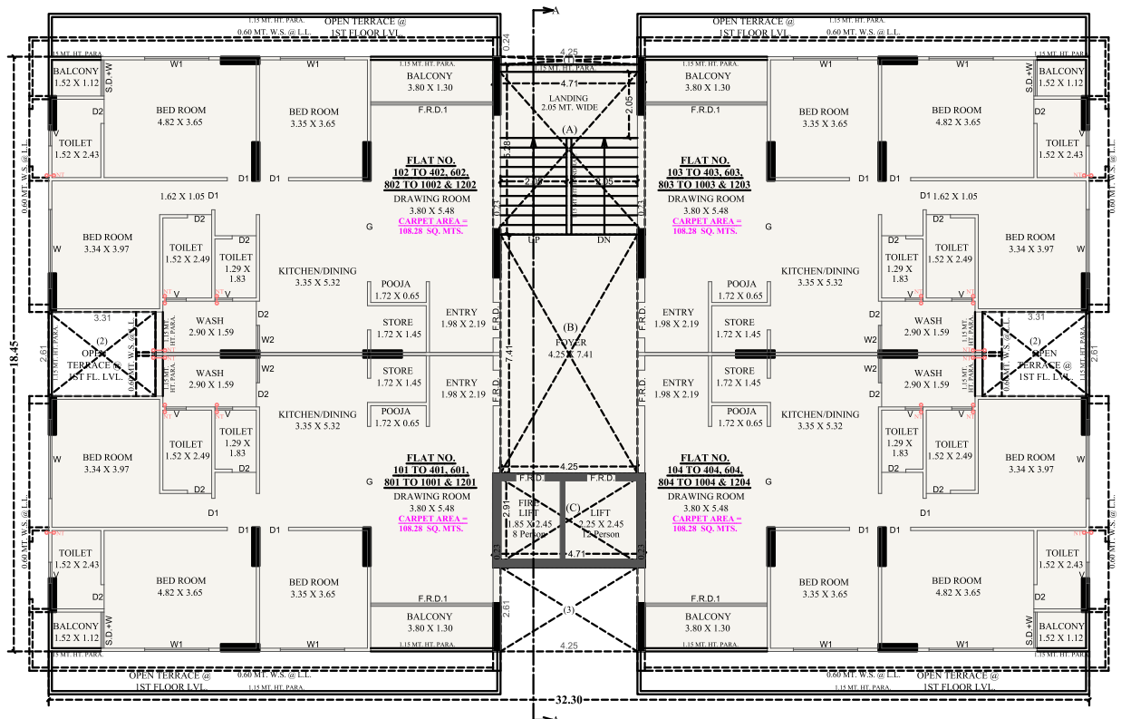
1ST TO 4TH, 6TH, 8TH TO 10TH & 12TH FLOOR PLAN
