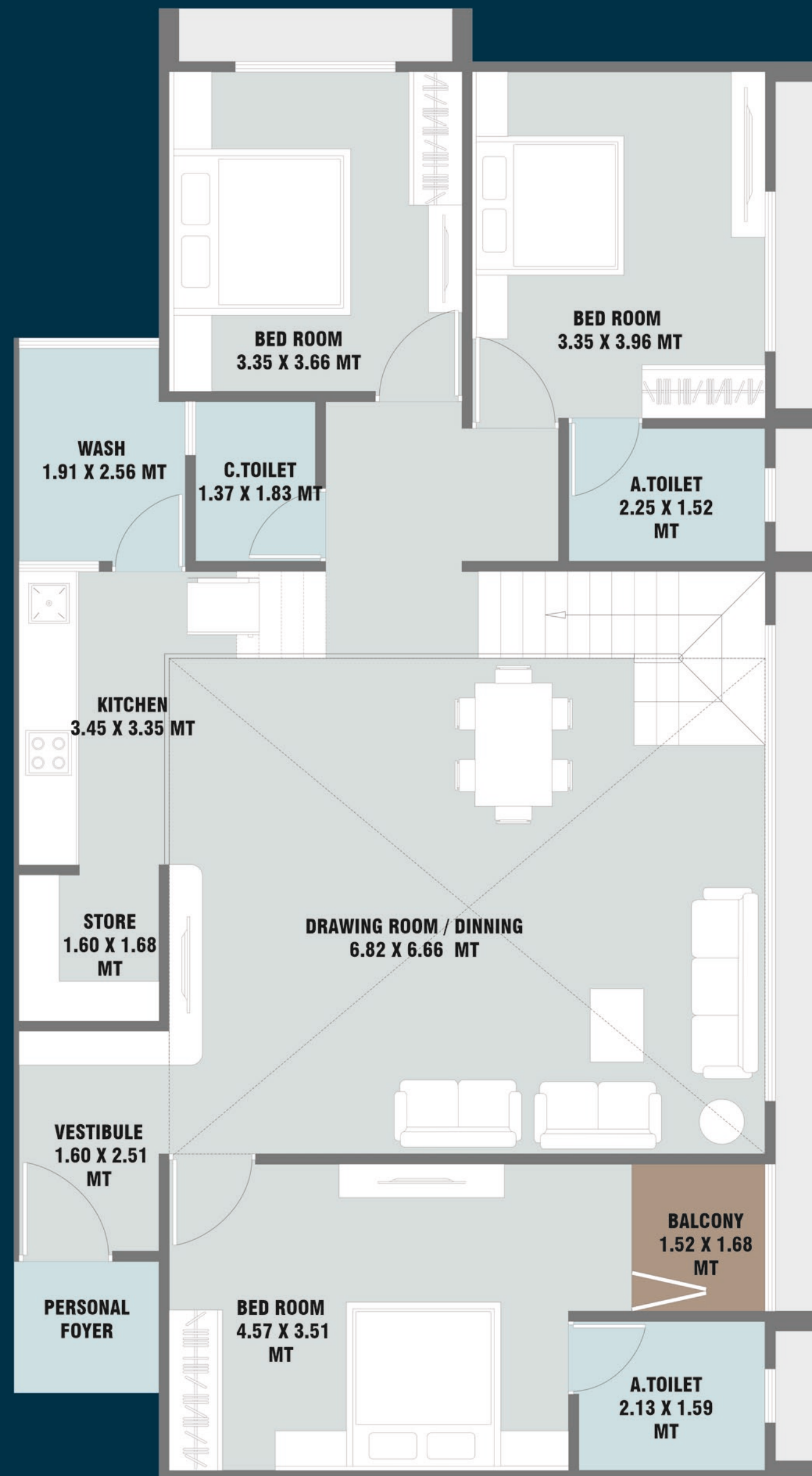
Lower Level Plan
