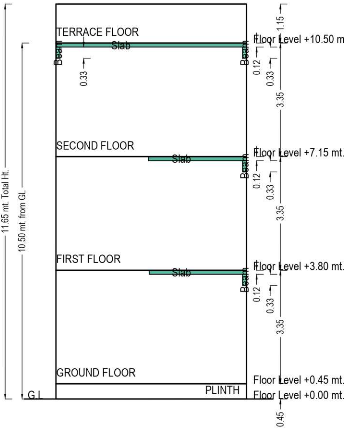
Sectional Diagram
