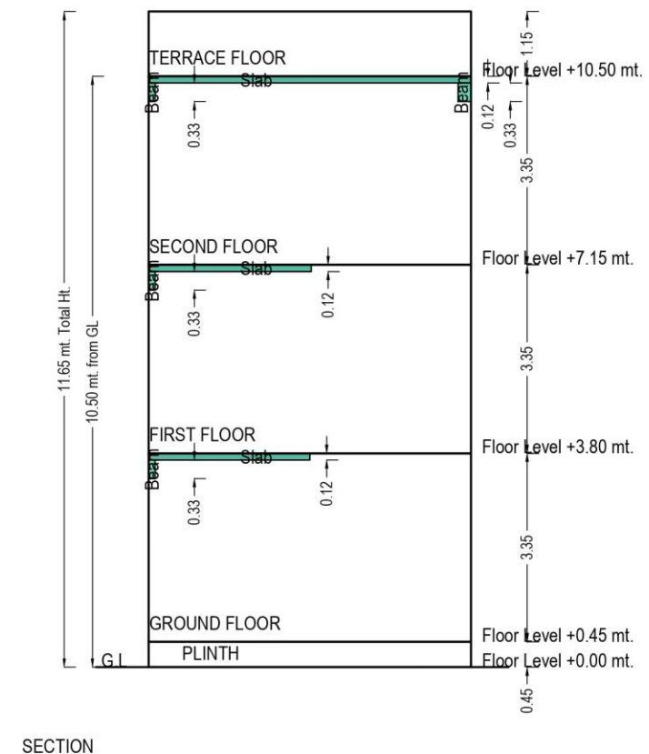
Sectional Diagram
