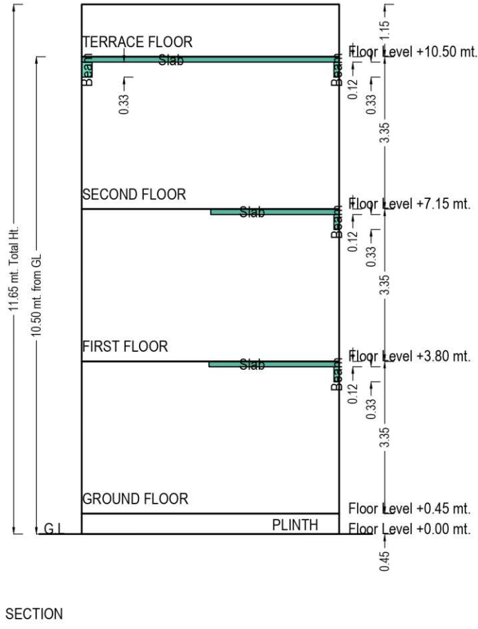
Sectional Diagram
