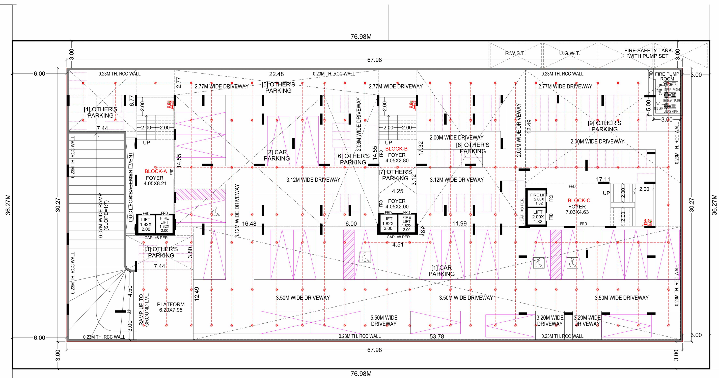
BASEMENT PLAN SCALE:- 1.0 CM = 2.0 MT.
