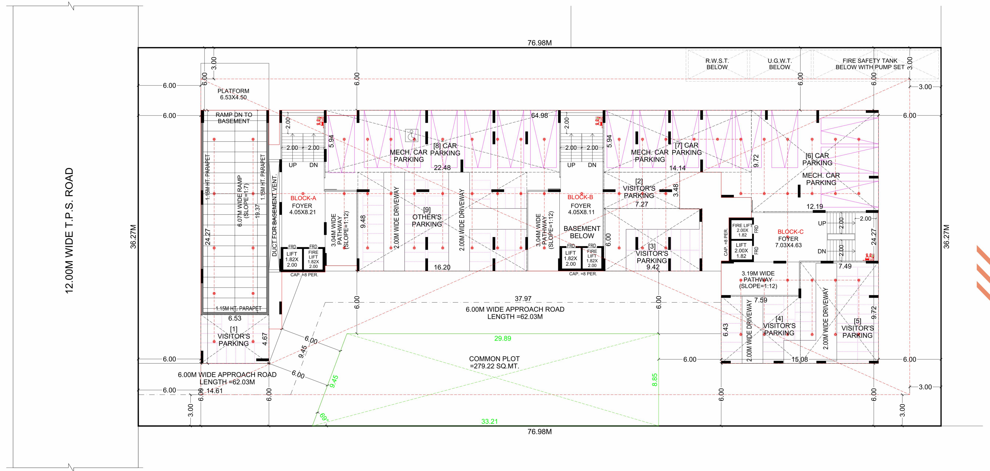
GROUND FLOOR PARKING LAYOUT PLAN SCALE:- 1.0 CM = 2.0 MT.
