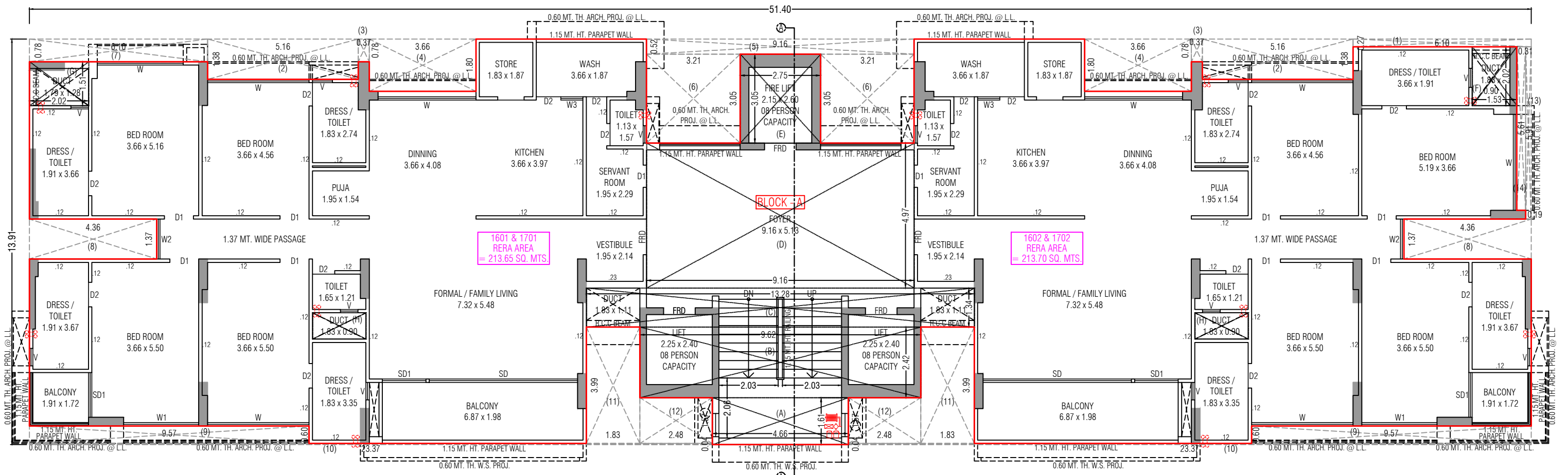
TYPICAL FLOOR PLAN ( 16TH TO 17TH FLOOR )
