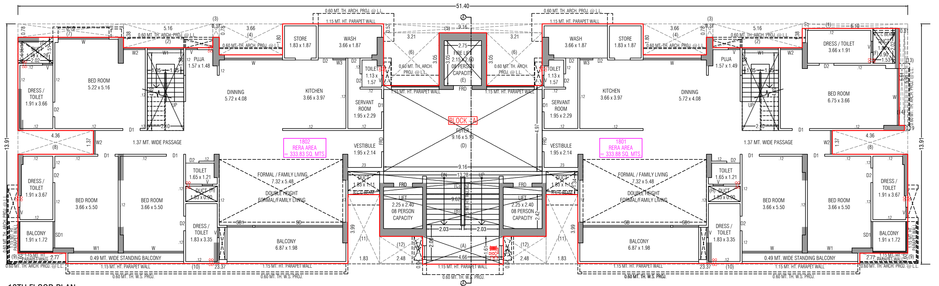
18TH FLOOR PLAN
