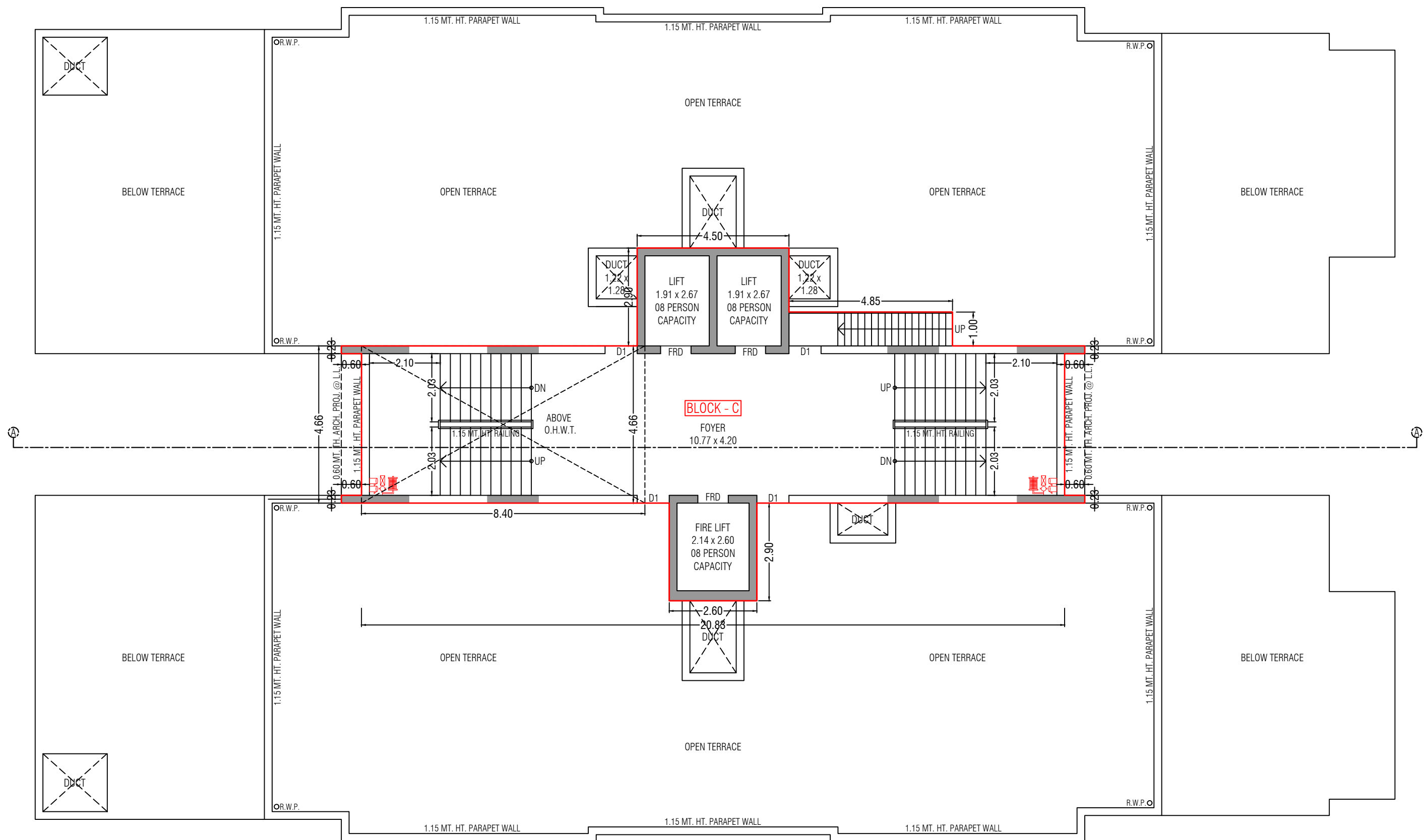
OPEN TERRACE & STAIR CABIN PLAN
