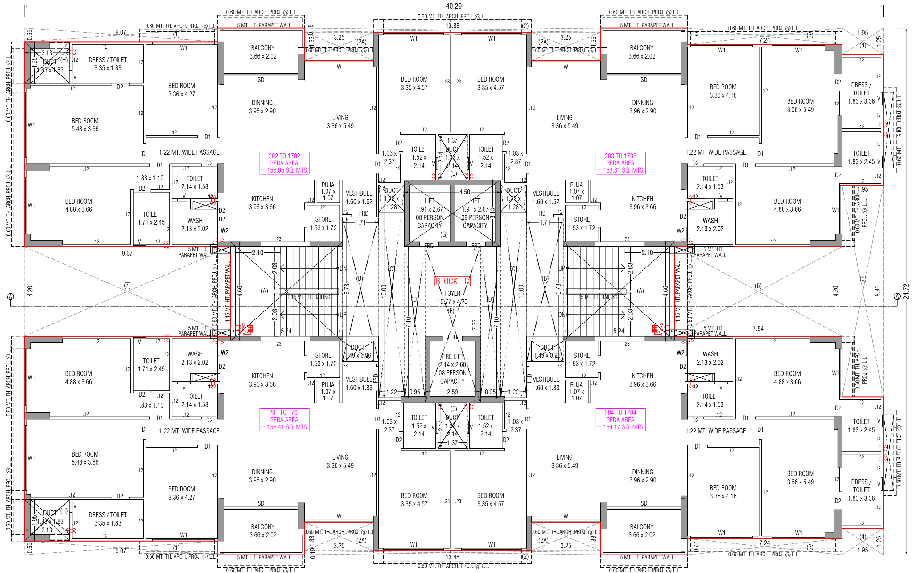
TYPICAL FLOOR PLAN ( 2ND TO 17TH FLOOR )
