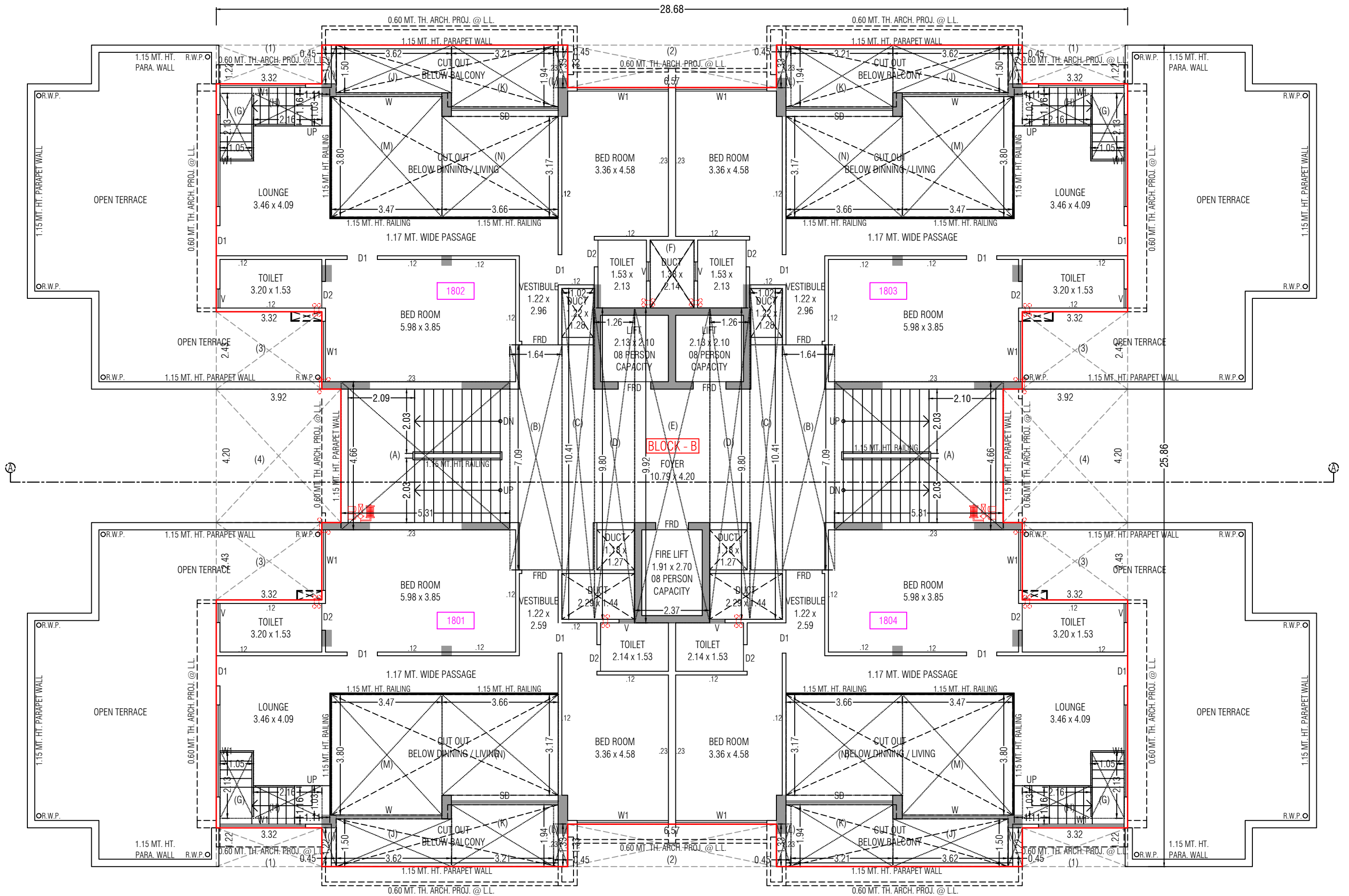
19TH FLOOR PLAN
