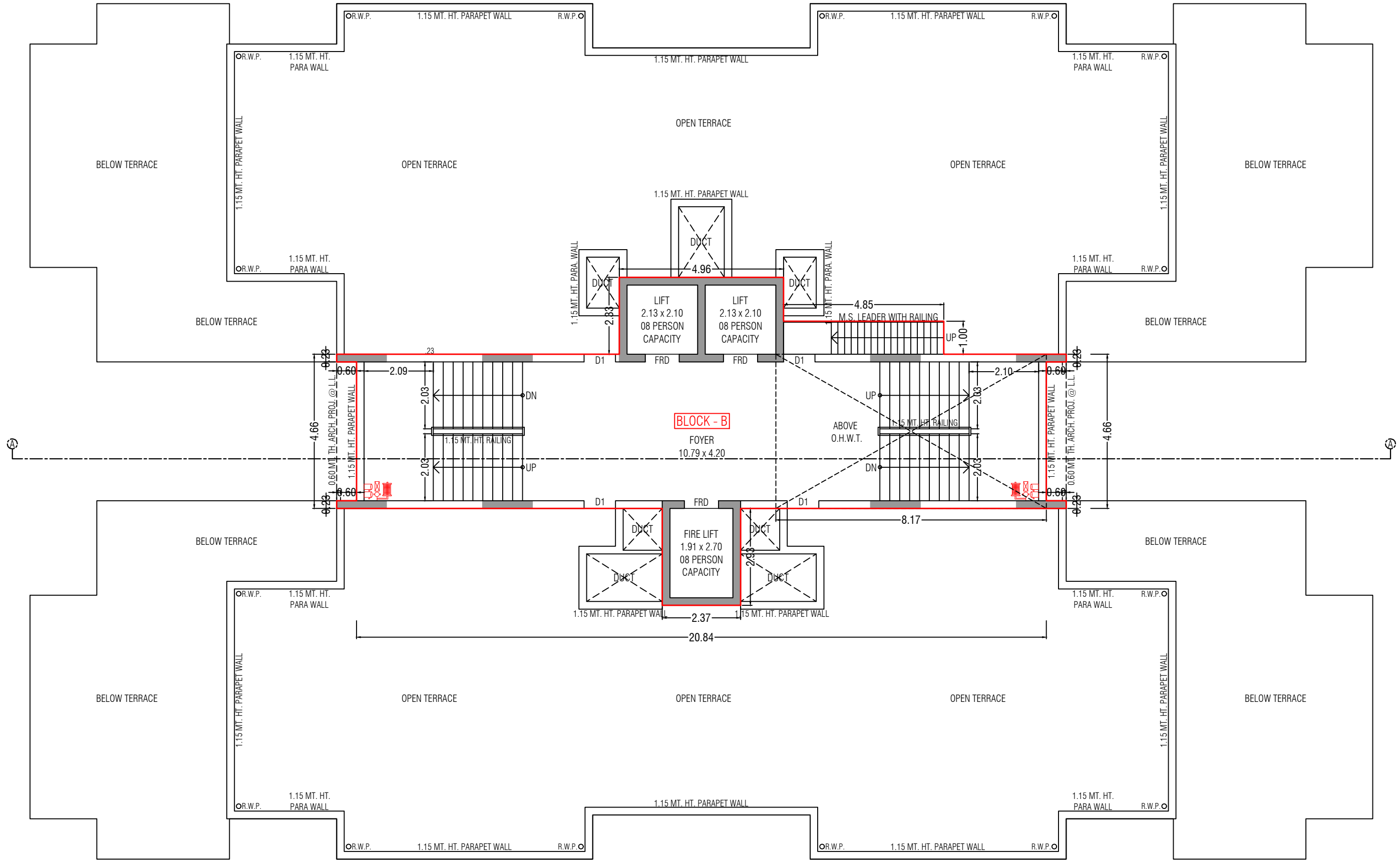
OPEN TERRACE & STAIR CABIN PLAN
