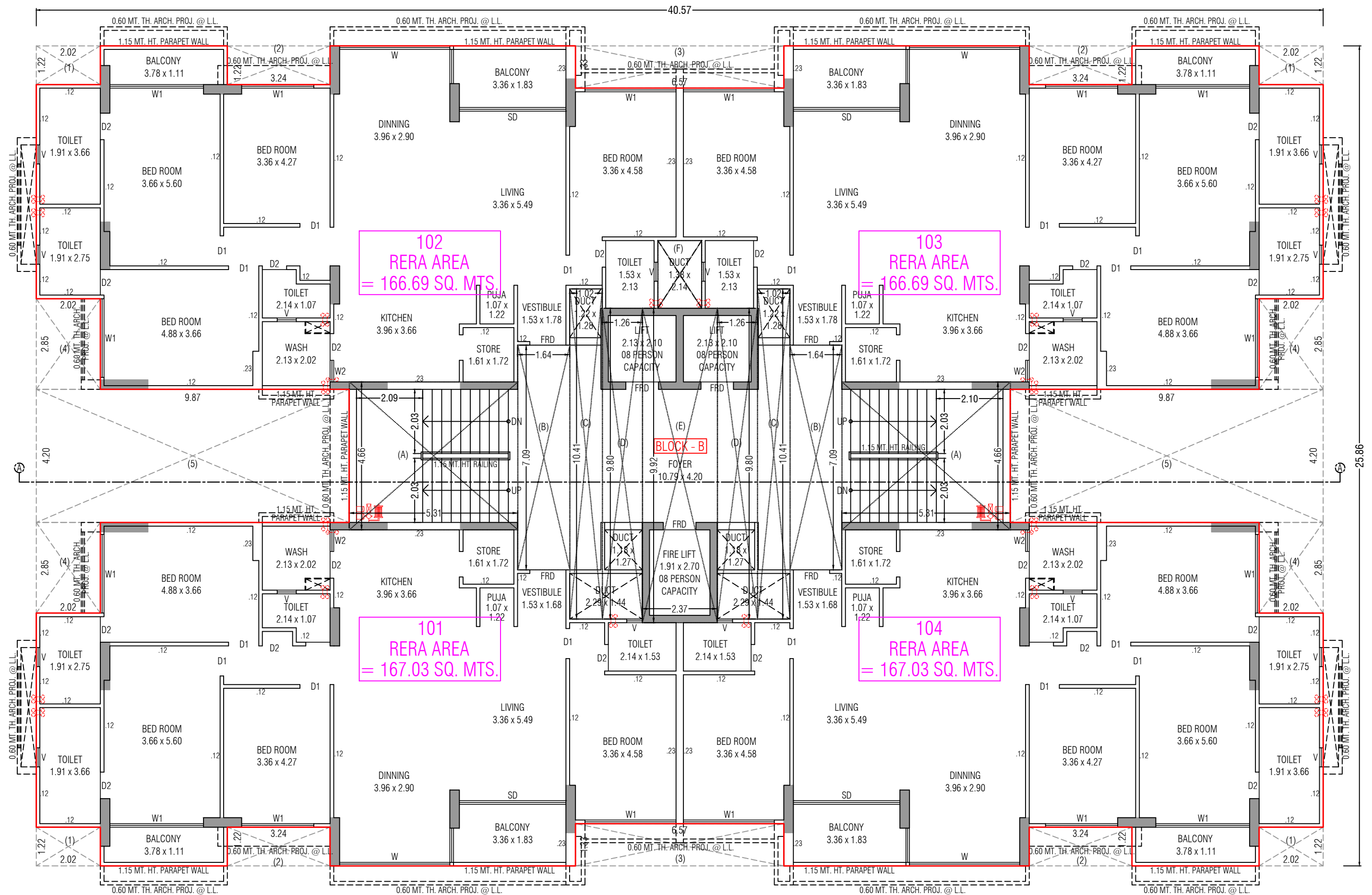
TYPICAL FLOOR PLAN ( 2ND TO 17TH FLOOR )
