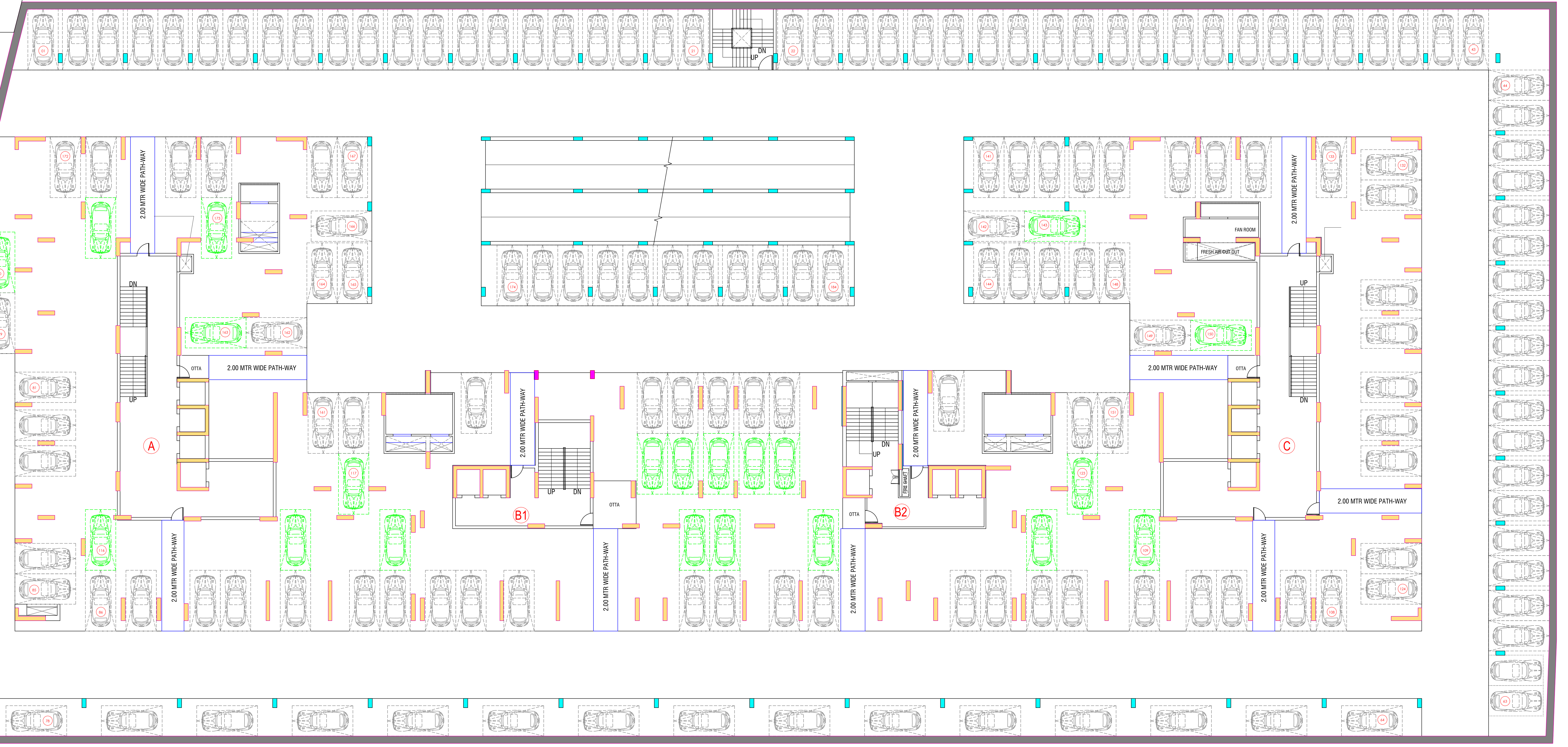
3rd BASEMENT PLAN
