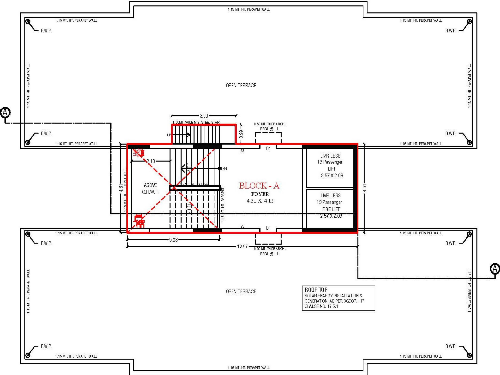
OPEN TERRACE WITH O.H.W.T. PLAN (BLOCK-A)
