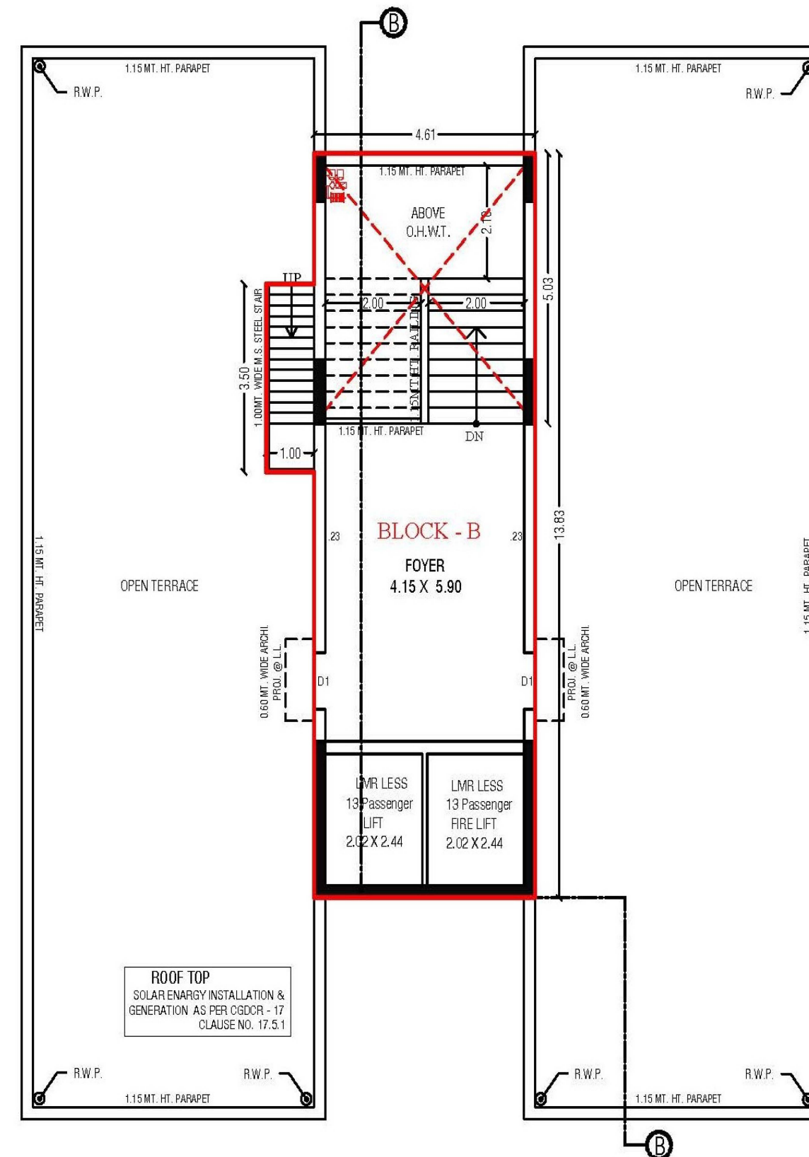
OPEN TERRACE WITH O.H.W.T. PLAN (BLOCK-B)
