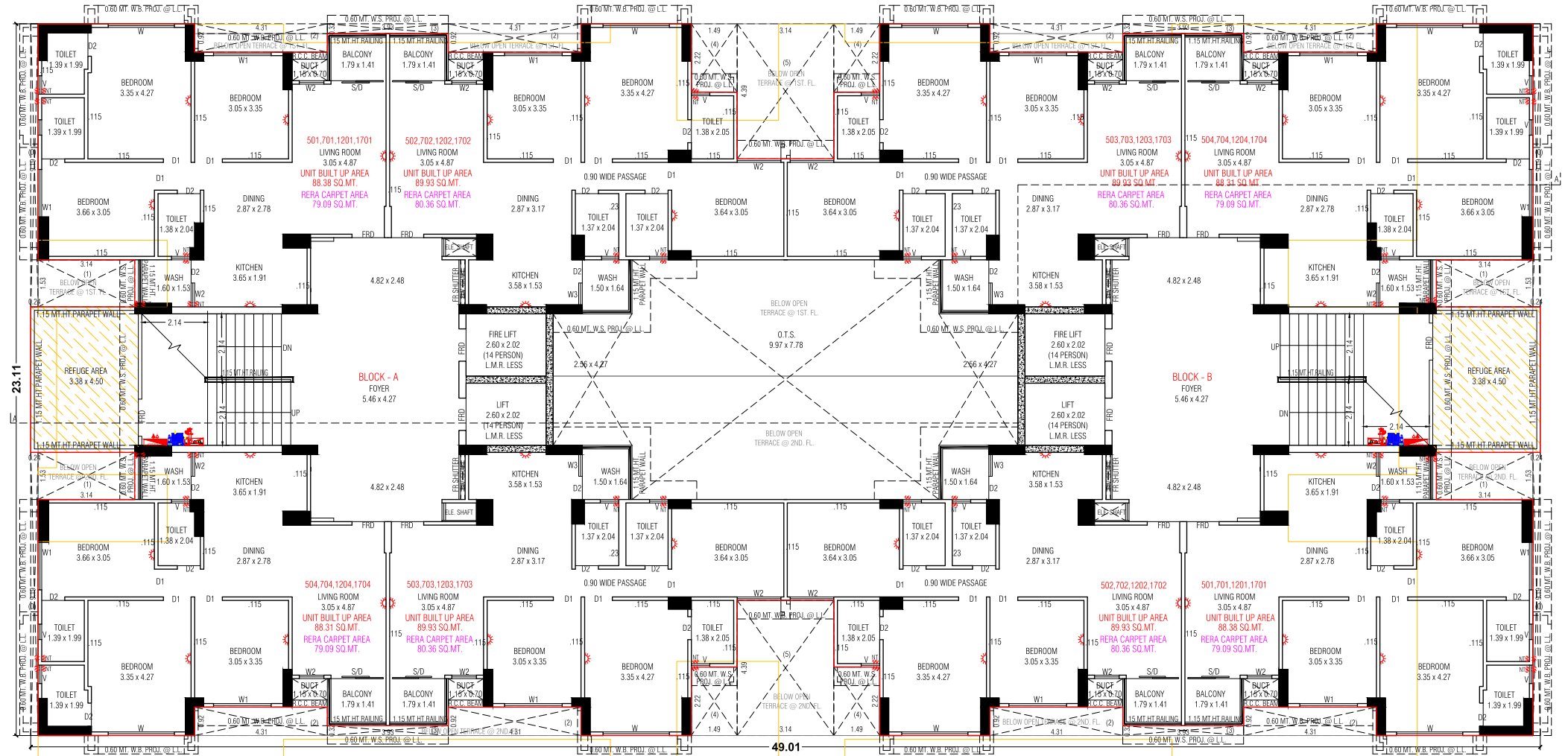
5TH, 7TH, 12TH & 17TH FLOOR PLAN (WITH REFUGE AREA)
