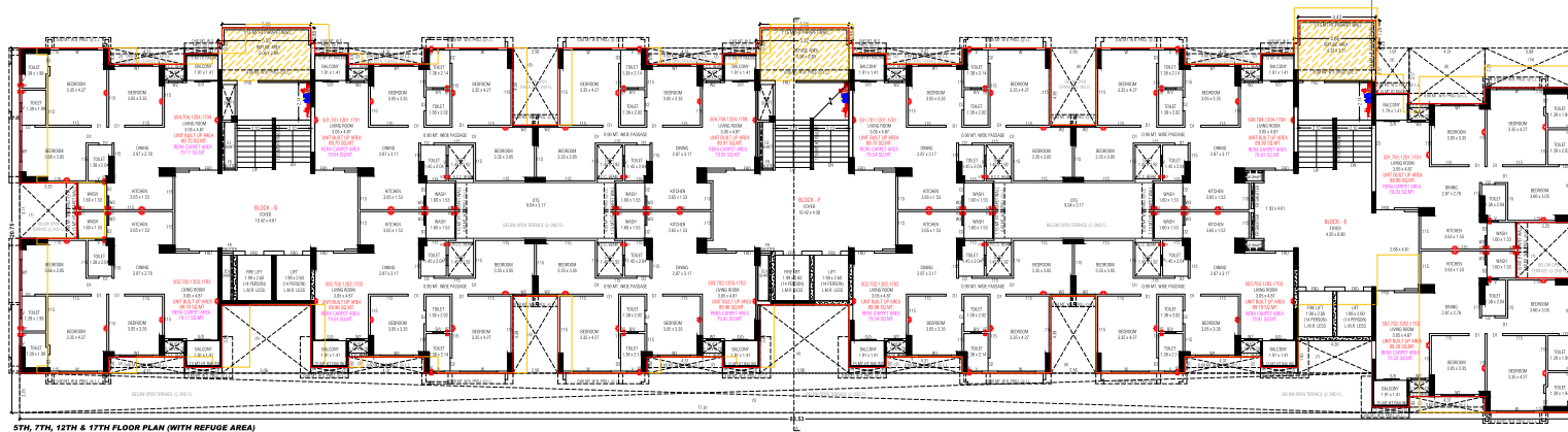
5TH, 7TH, 12TH & 17TH FLOOR PLAN (WITH REFUGE AREA)
