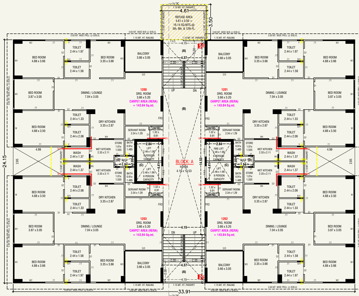
12th FL. PLAN (BLOCK-A)
