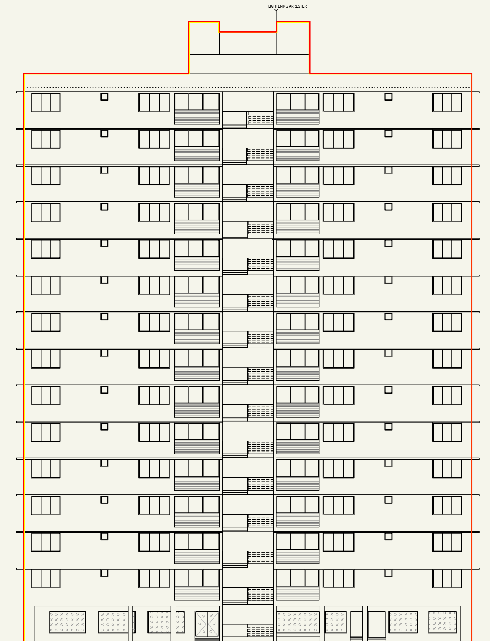
ELEVATION (BLOCK-B)
