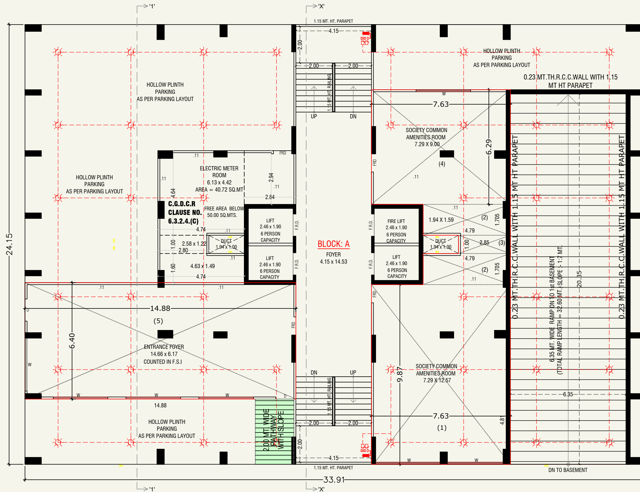
GROUND FLOOR PLAN (BLOCK-A)
