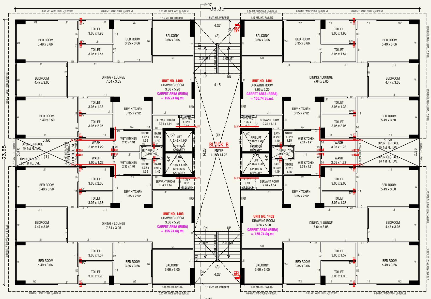
14th FLOOR PLAN (BLOCK-B)
