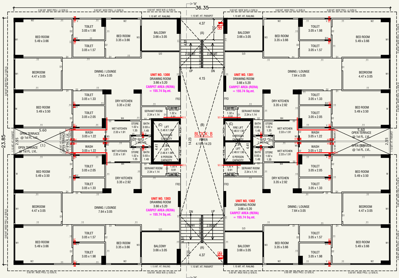
13th FLOOR PLAN (BLOCK-B)
