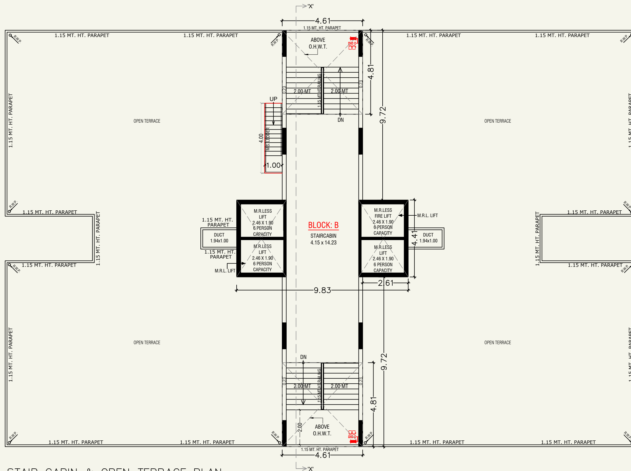
STAIR CABIN & OPEN TERRACE PLAN O.H.W.T., LIFT MACHINE ROOM, (BLOCK-B)
