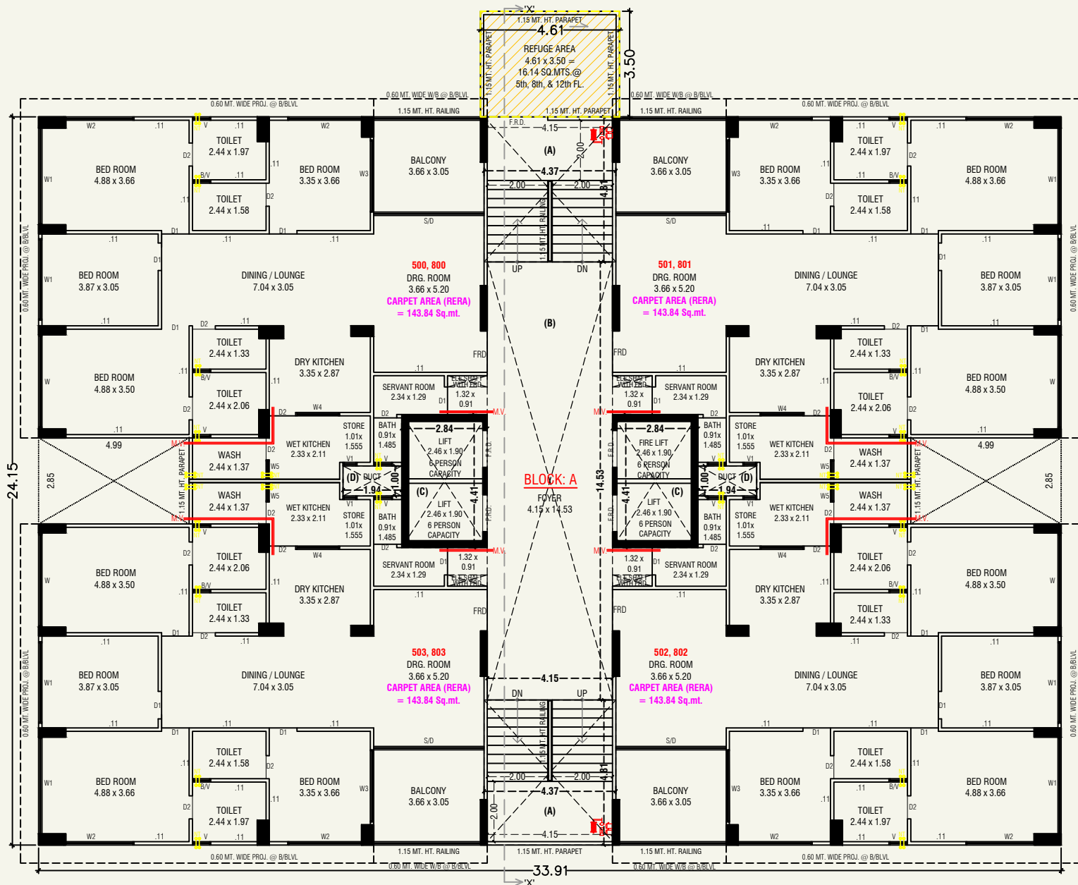
5th FL. & 8th FL. PLAN (BLOCK-A)
