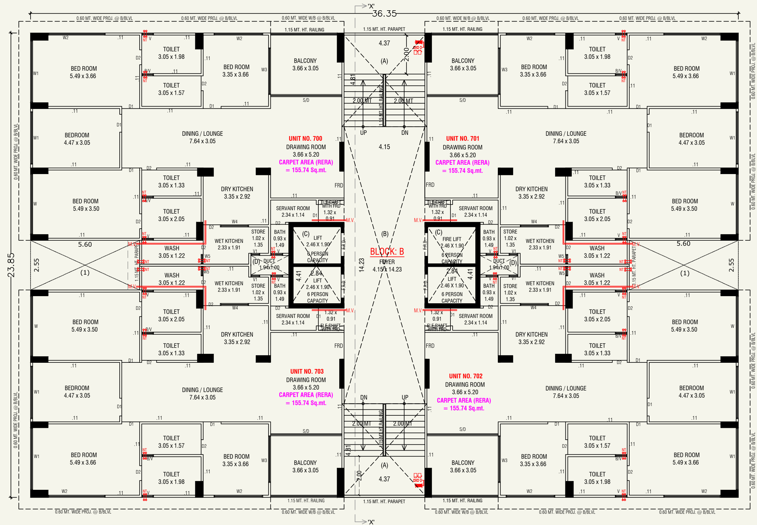
7th FLOOR PLAN (BLOCK-B)
