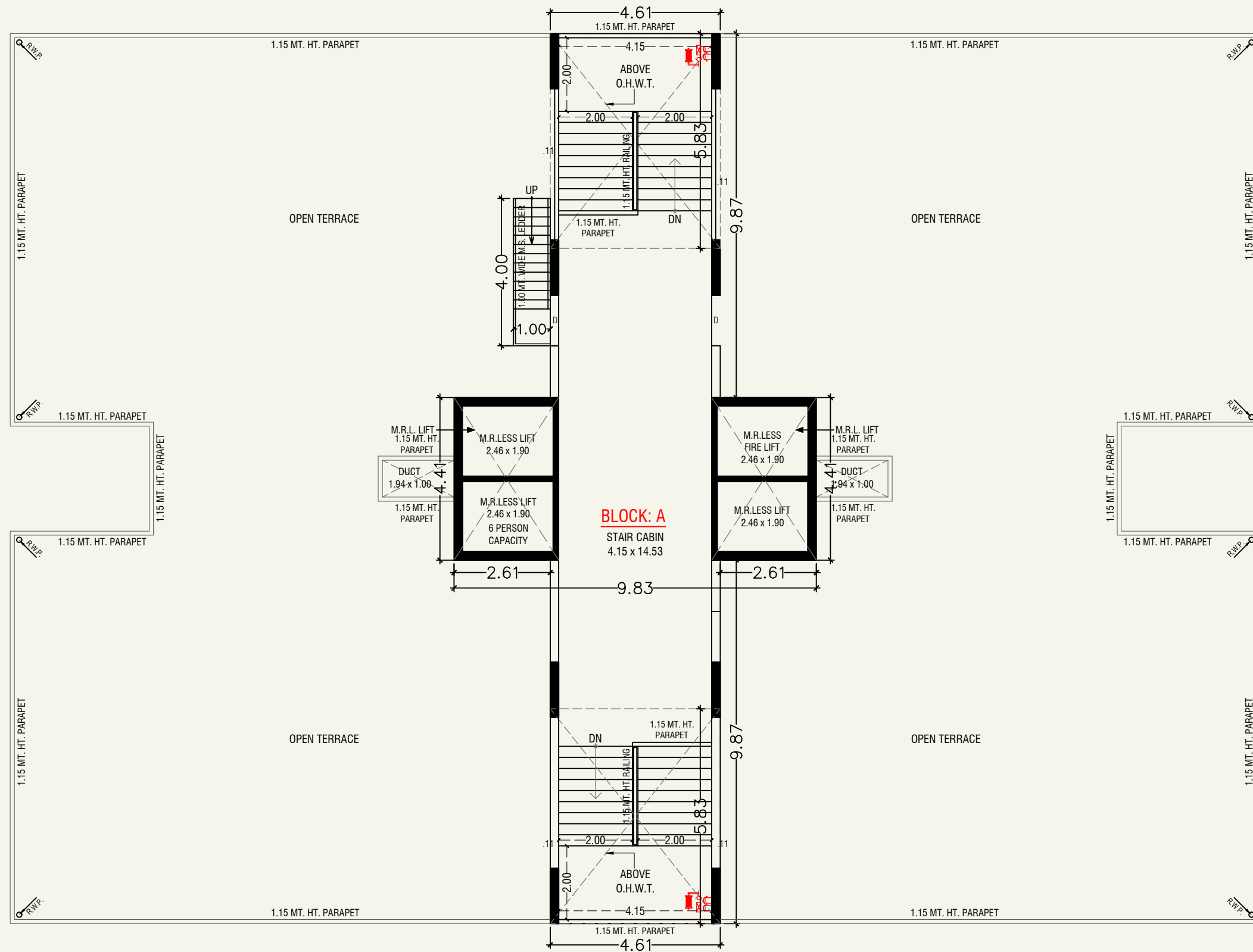
STAIR CABIN & OPEN TERRACE PLAN O.H.W.T., LIFT MACHINE ROOM, (BLOCK-A)
