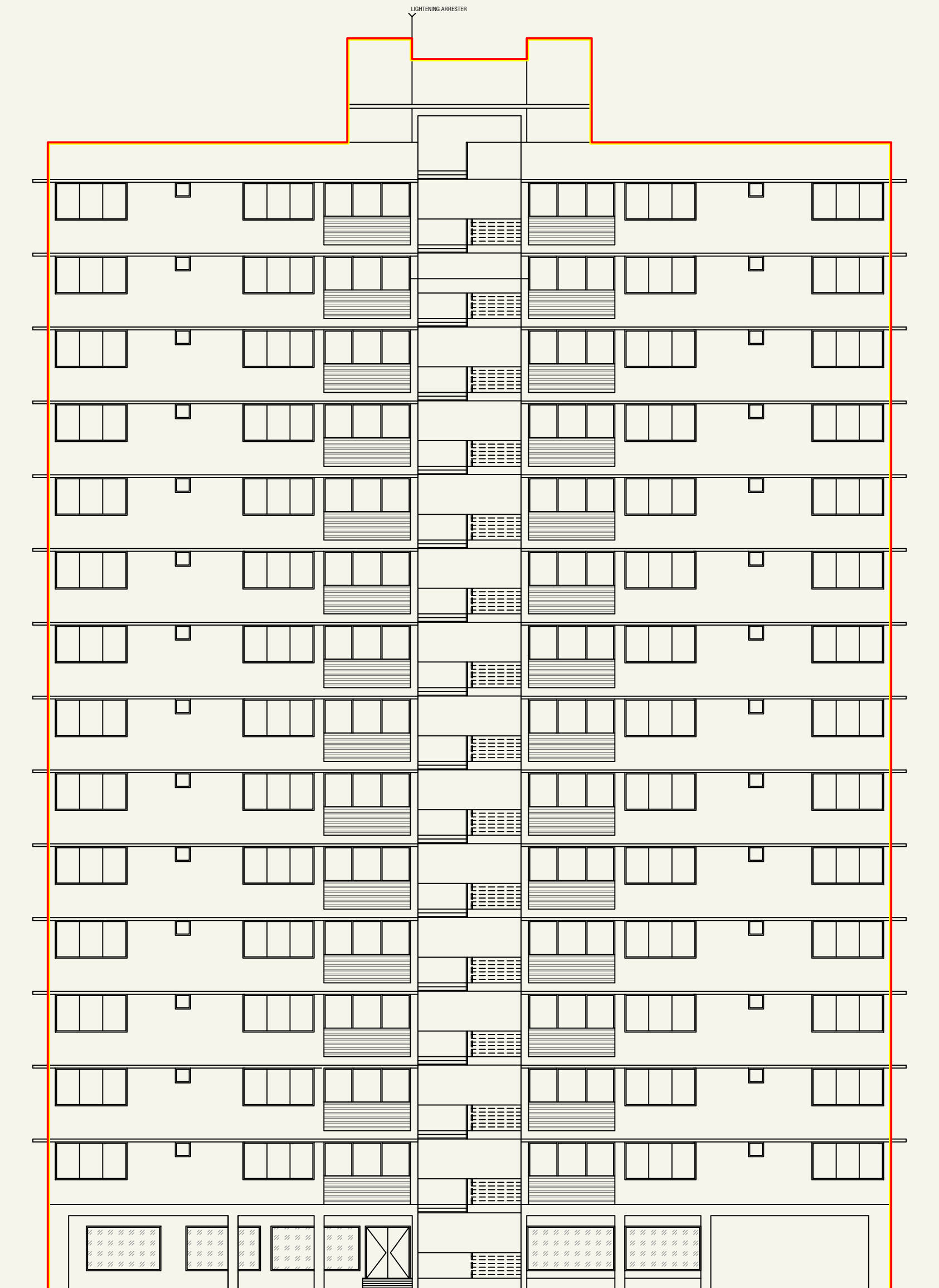
ELEVATION (BLOCK-A)
