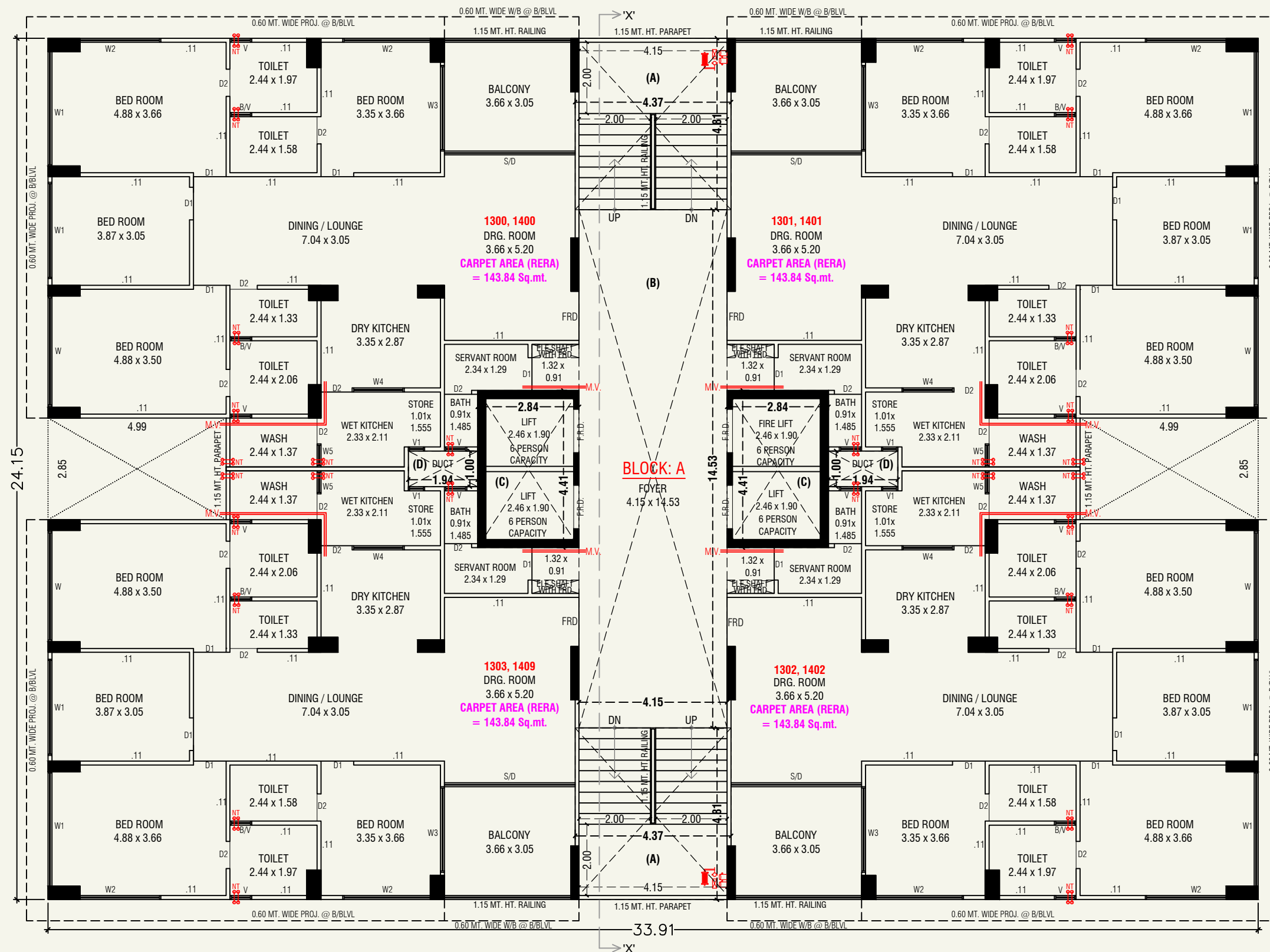
13th & 14th FL. PLAN (BLOCK-A)
