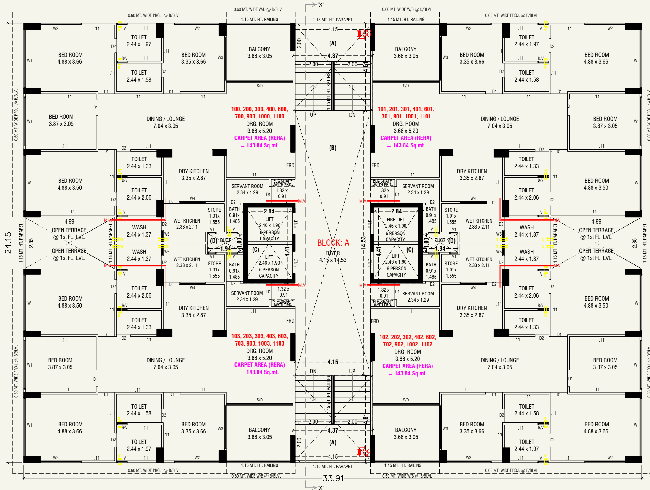
1st. to 4th, 6th, 7th, 9th to 11th FL. PLAN (BLOCK-A)
