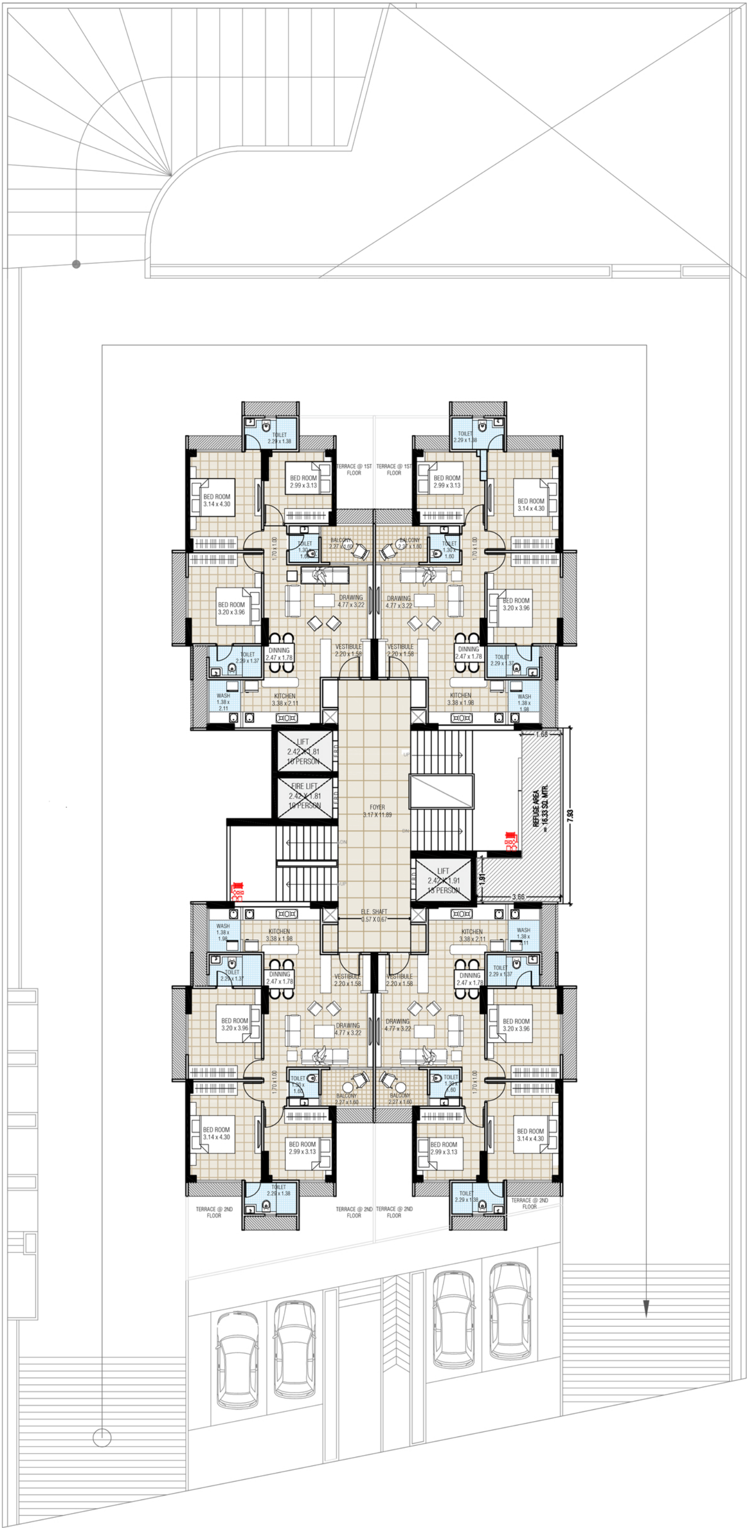
TYPICAL FLOOR WITH REFUGE |
