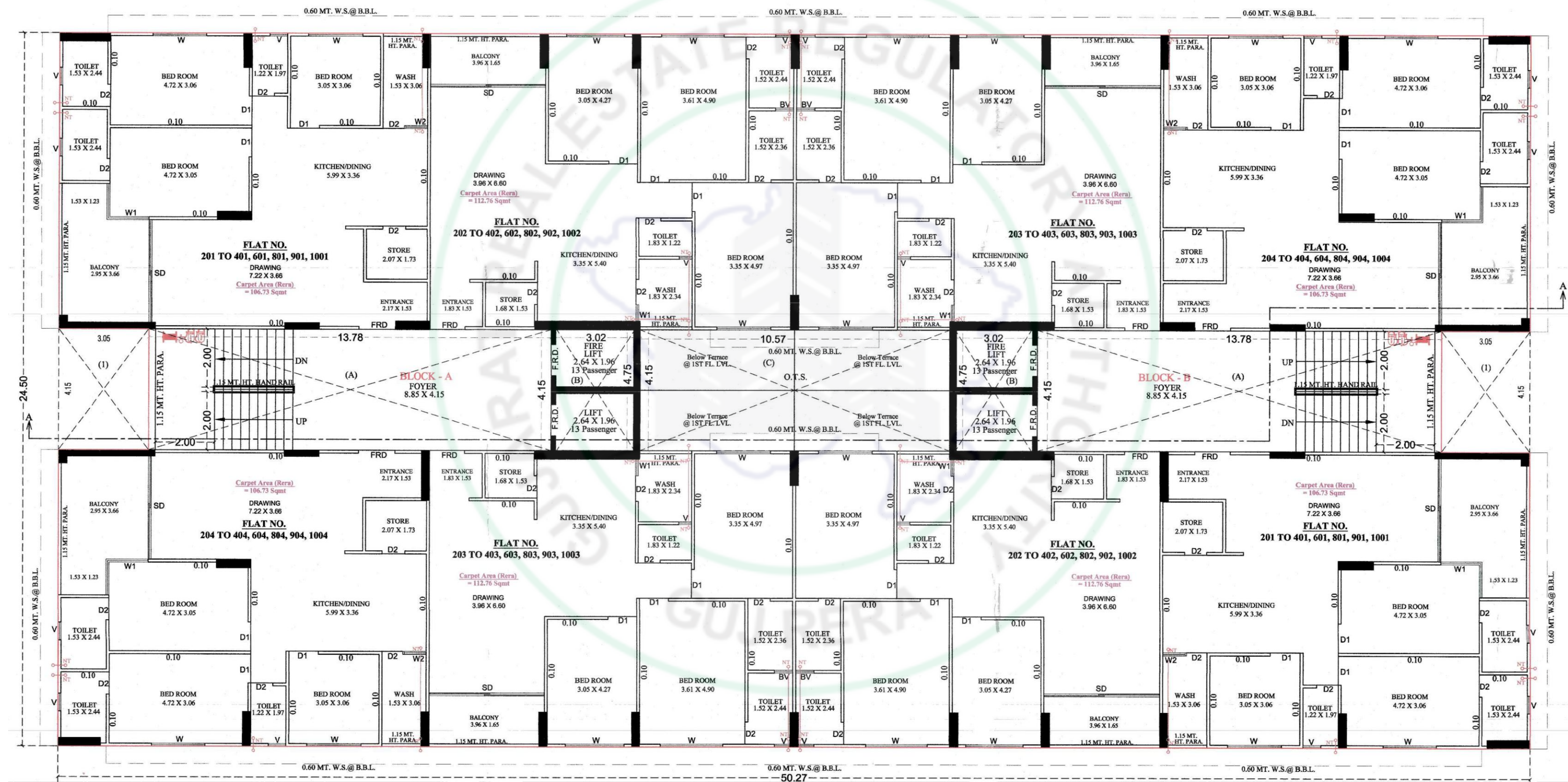
2ND TO 4TH, 6TH, 8TH, 9TH, 10TH FLOOR PLAN NOTE :- ALL OUTER & INTERNAL WALL ARE OF 0.10 MT. TH. B/W WALL
