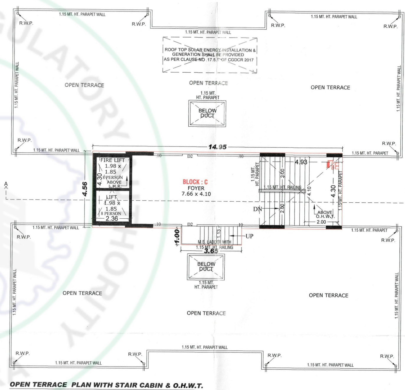
OPEN TERRACE PLAN WITH STAIR CABIN & O.H.W.T.
