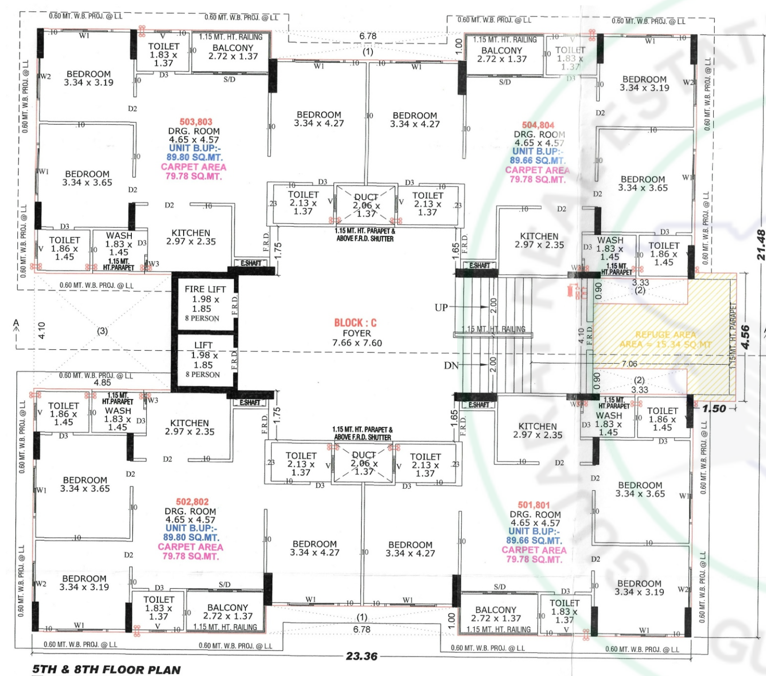
5TH & 8TH FLOOR PLAN
