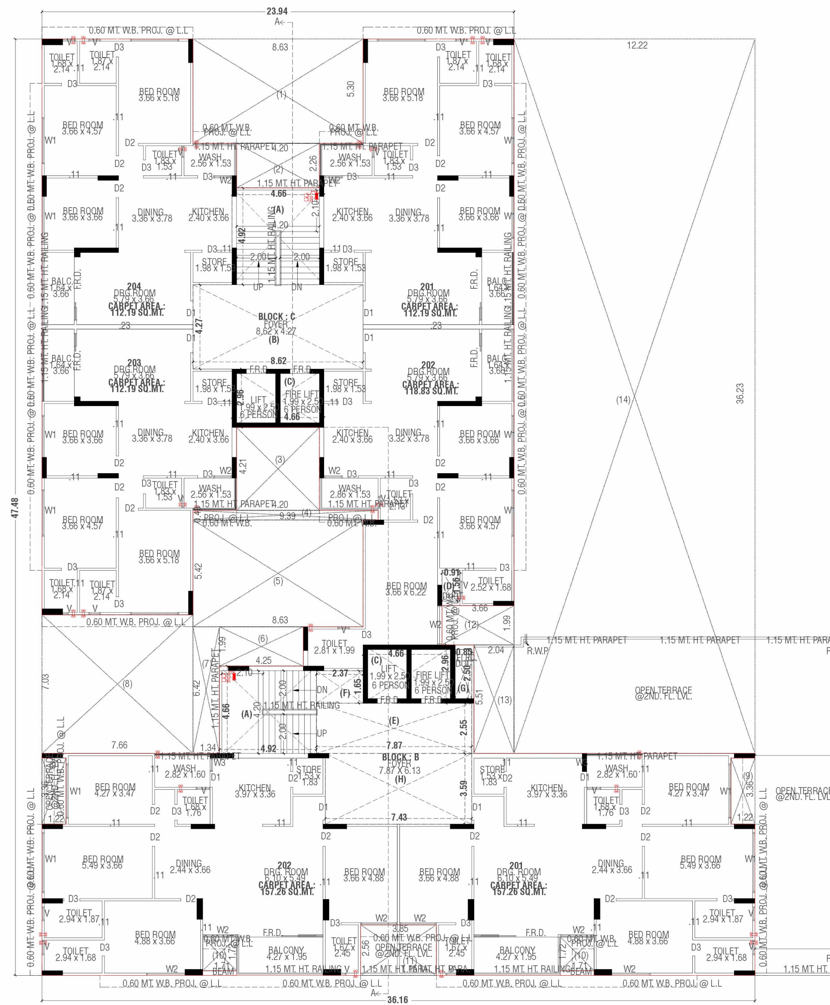
2ND. FL. PLAN
