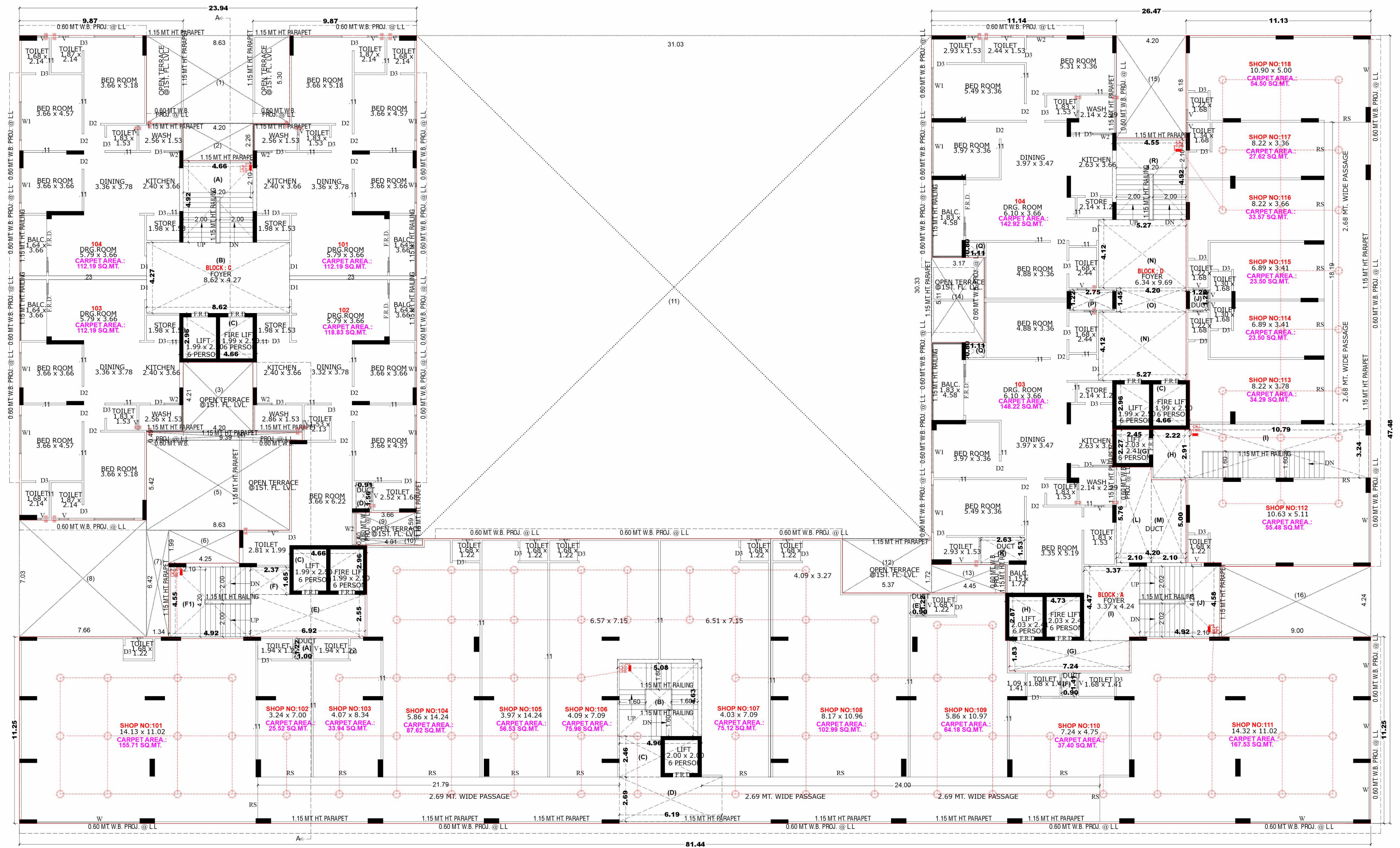
1ST. FL. PLAN
