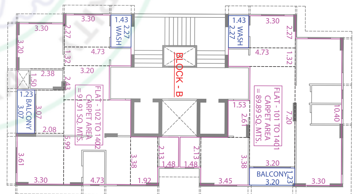
Rera Area Typical Floor Plan ( 1st To 14th Floor Plan )
