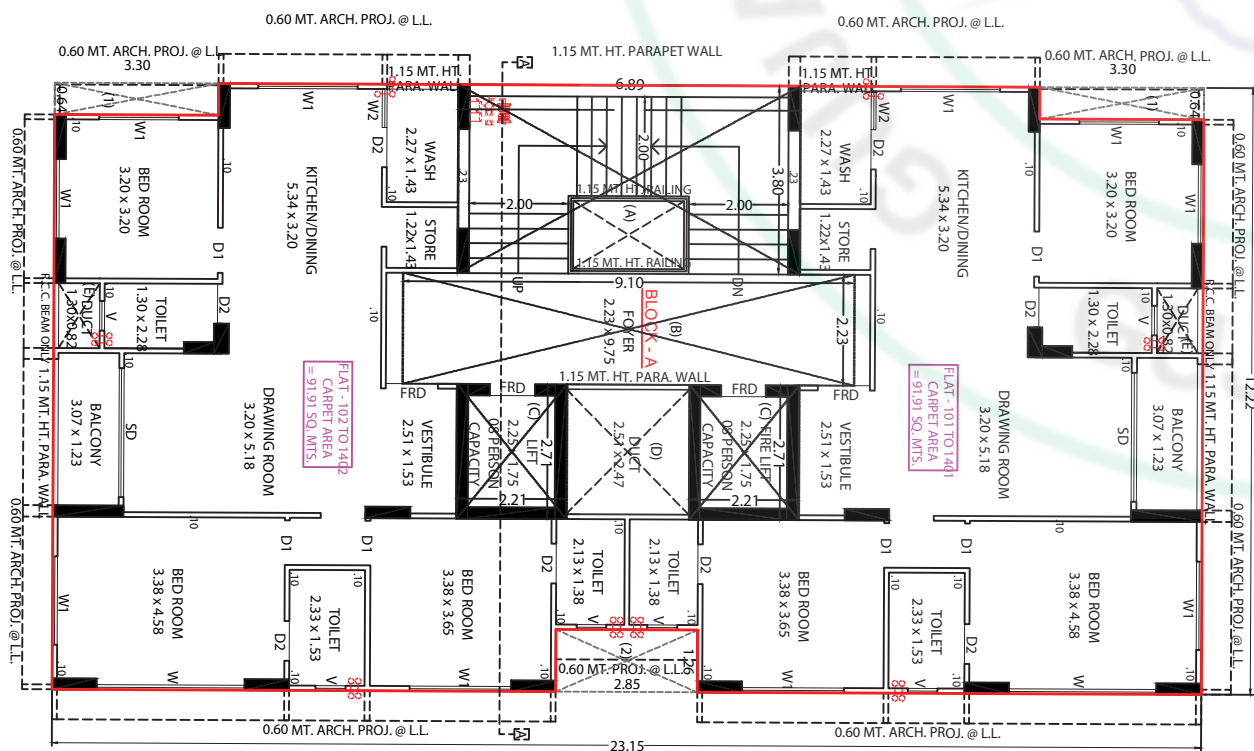
Typical Floor Plan (1st To 14th Floor Plan)
