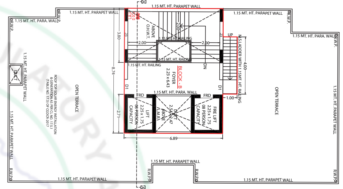
Open Terrace & Stair Cabin Plan
