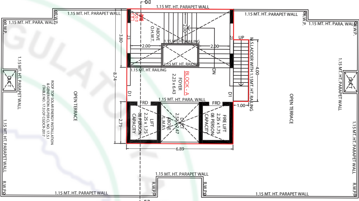
Open Terrace & Stair Cabin Plan
