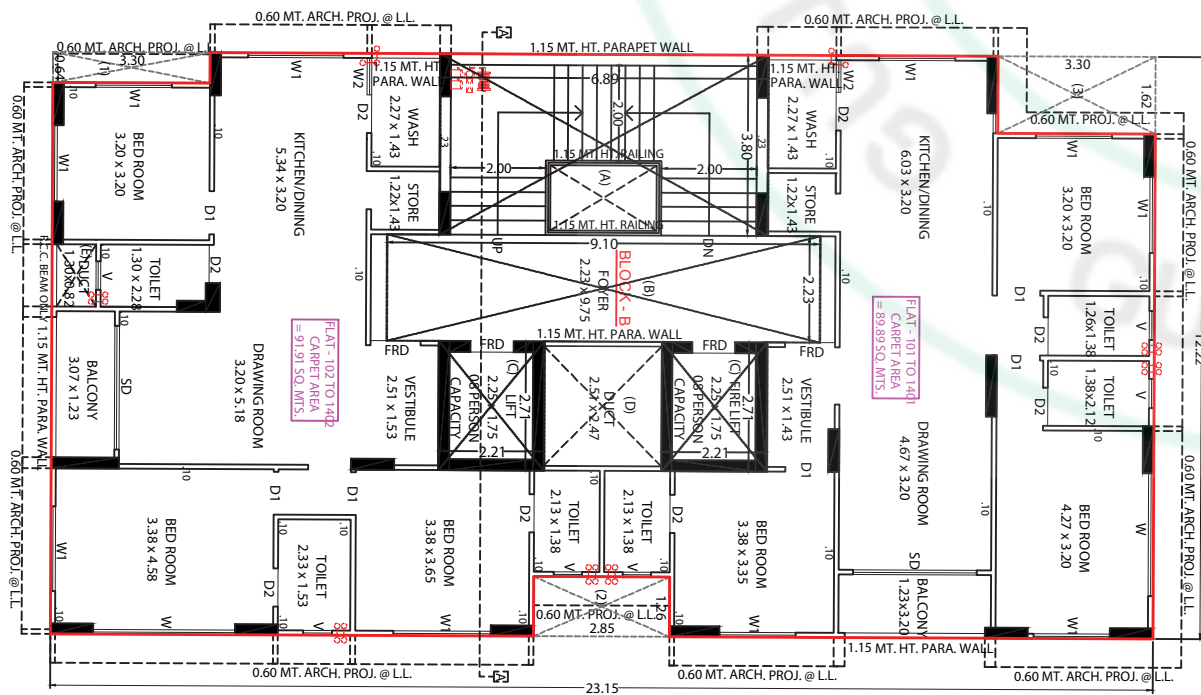
Typical Floor Plan ( 1st To 14th Floor Plan )
