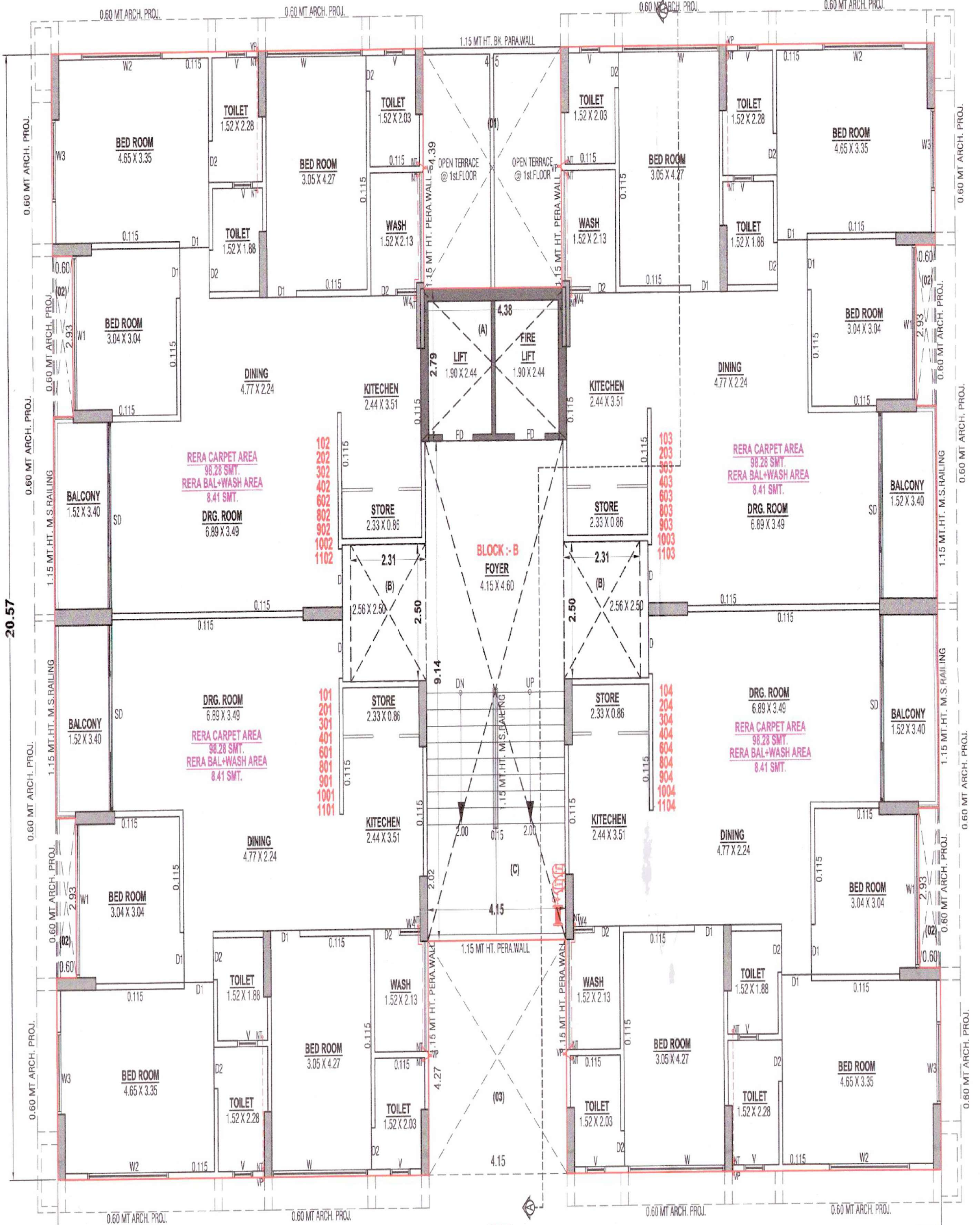
1st. to 4th., 6th., 8th., to 11th., FLOOR PLAN
