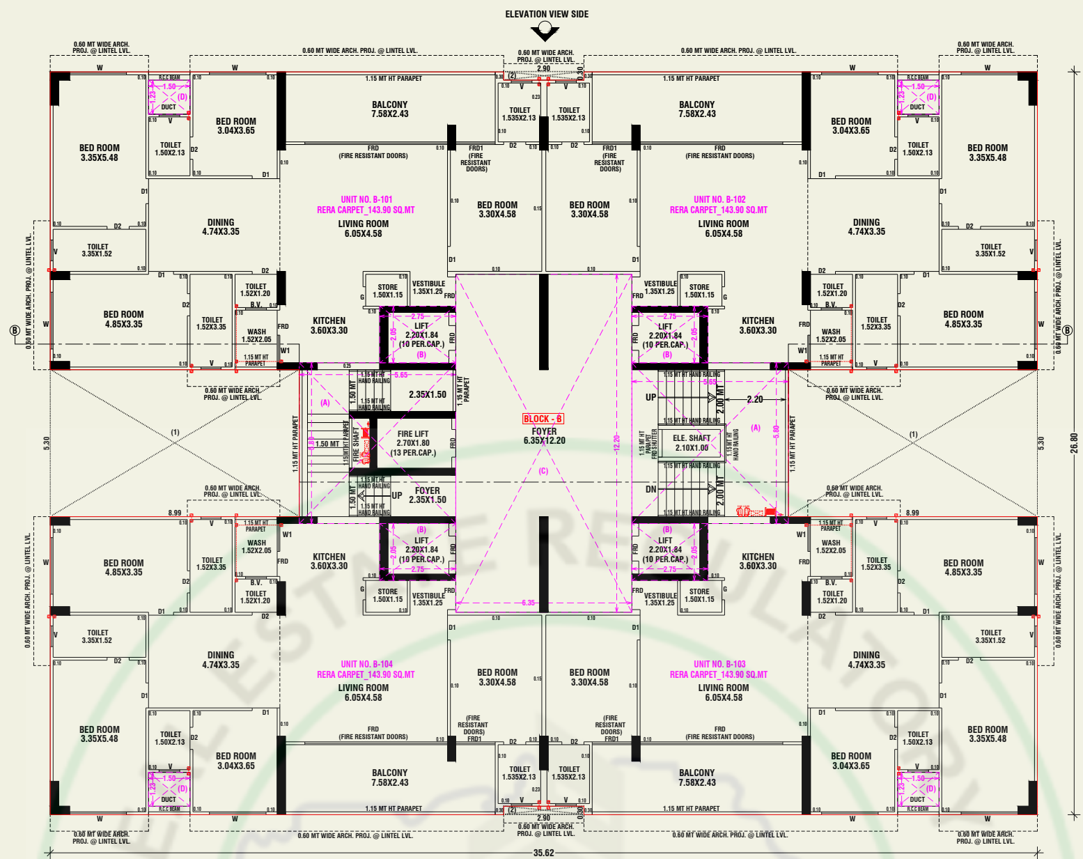
1st FLOOR PLAN (BLOCK-B)
