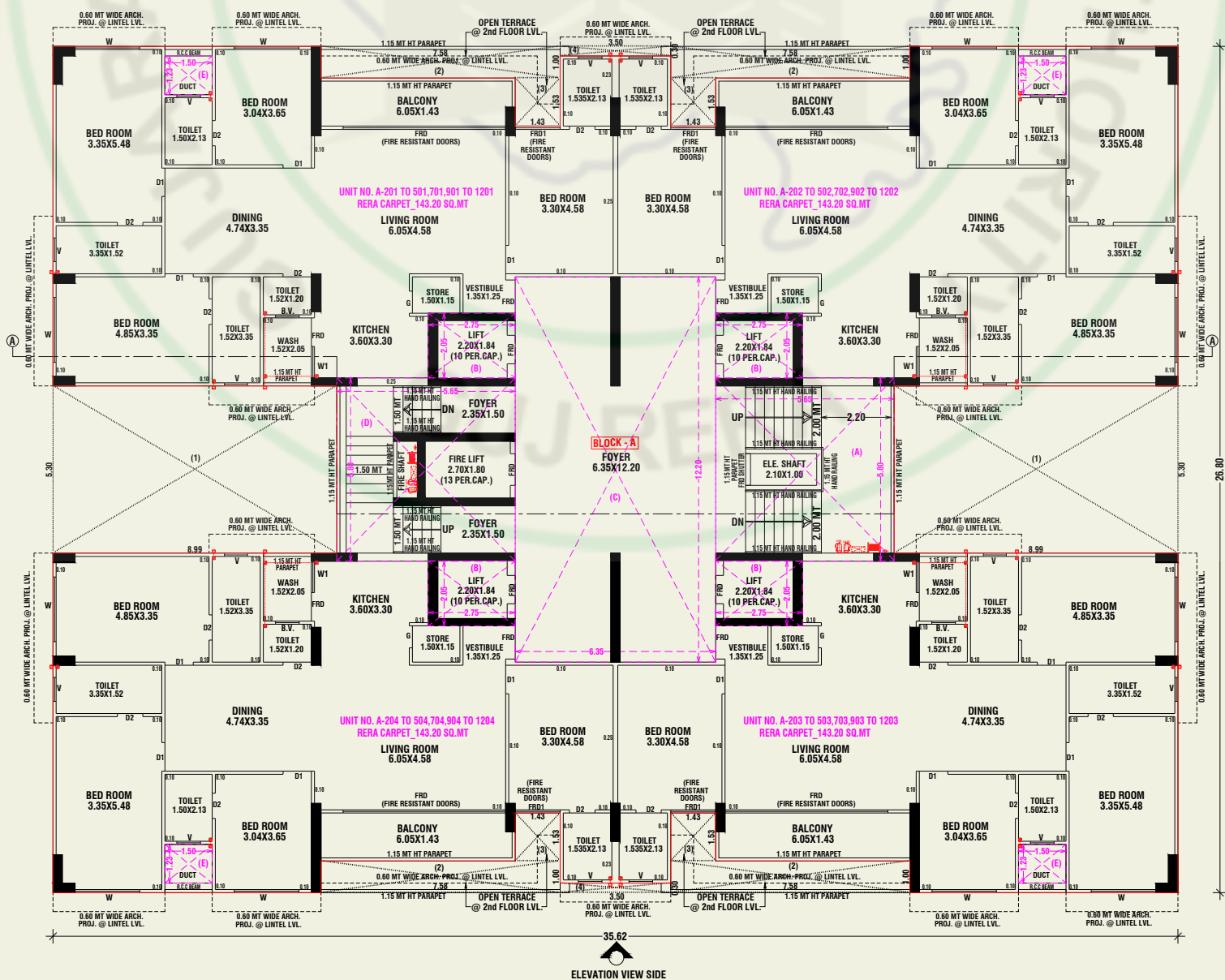
TYPICAL FLOOR PLAN (2nd TO 13th FLOOR) (BLOCK-A)
