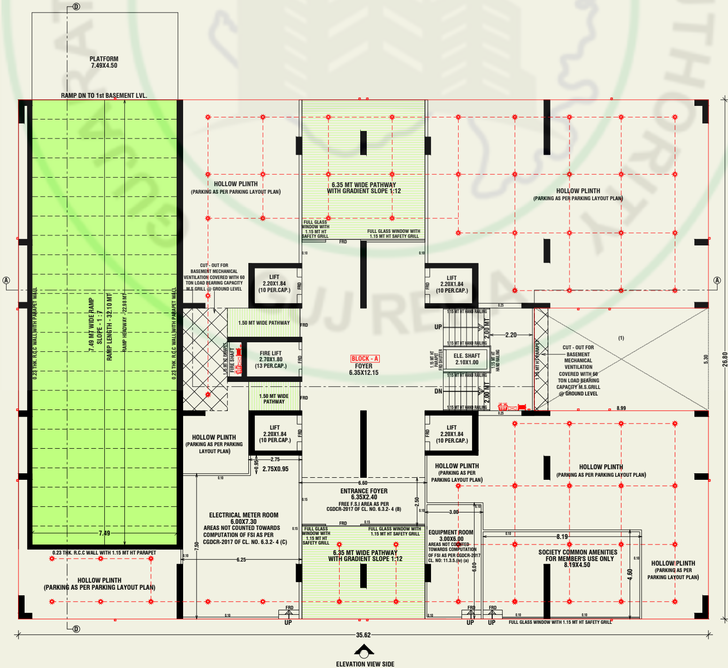
GROUND FLOOR PLAN (BLOCK-A)
