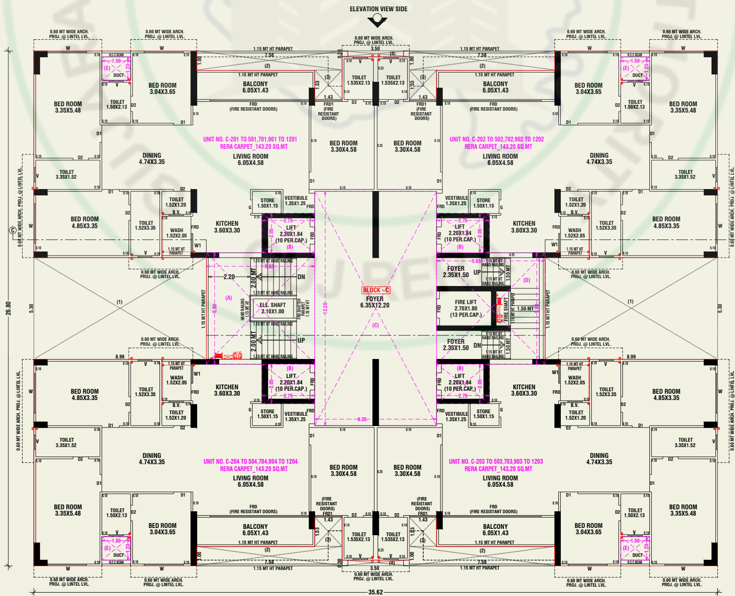
TYPICAL FLOOR PLAN (2nd TO 13th FLOOR) (BLOCK-C)
