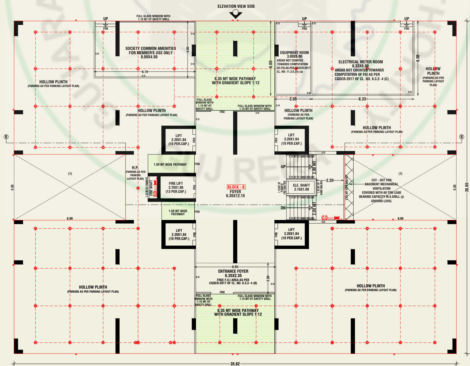
GROUND FLOOR PLAN (BLOCK-B)
