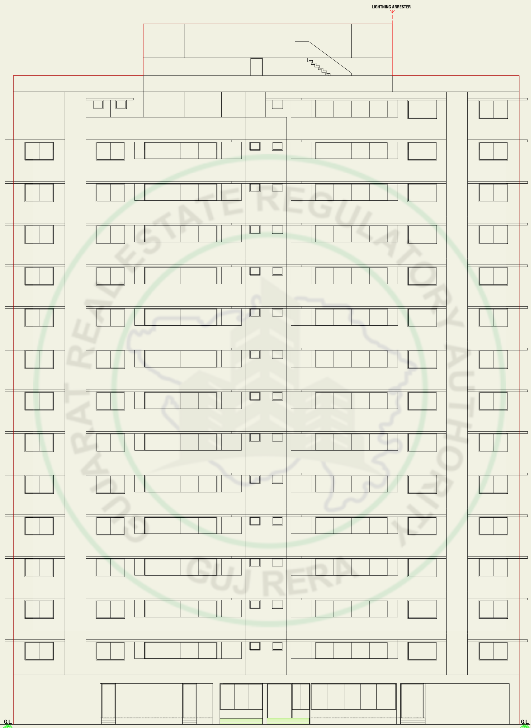
FRONT ELEVATION (BLOCK-C)
