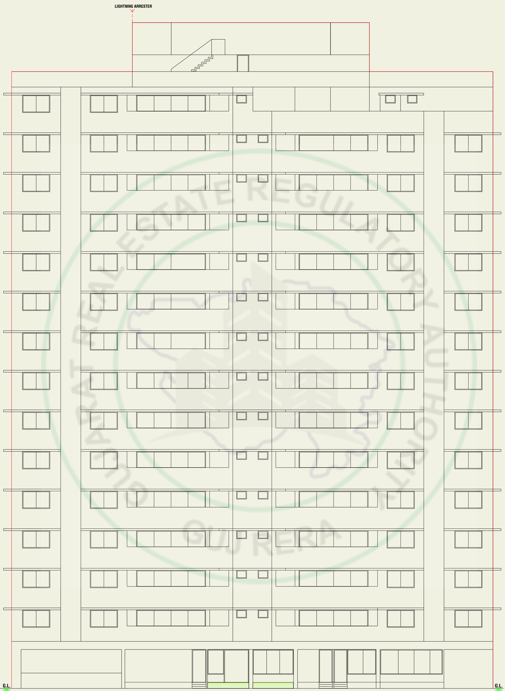
FRONT ELEVATION (BLOCK-A)
