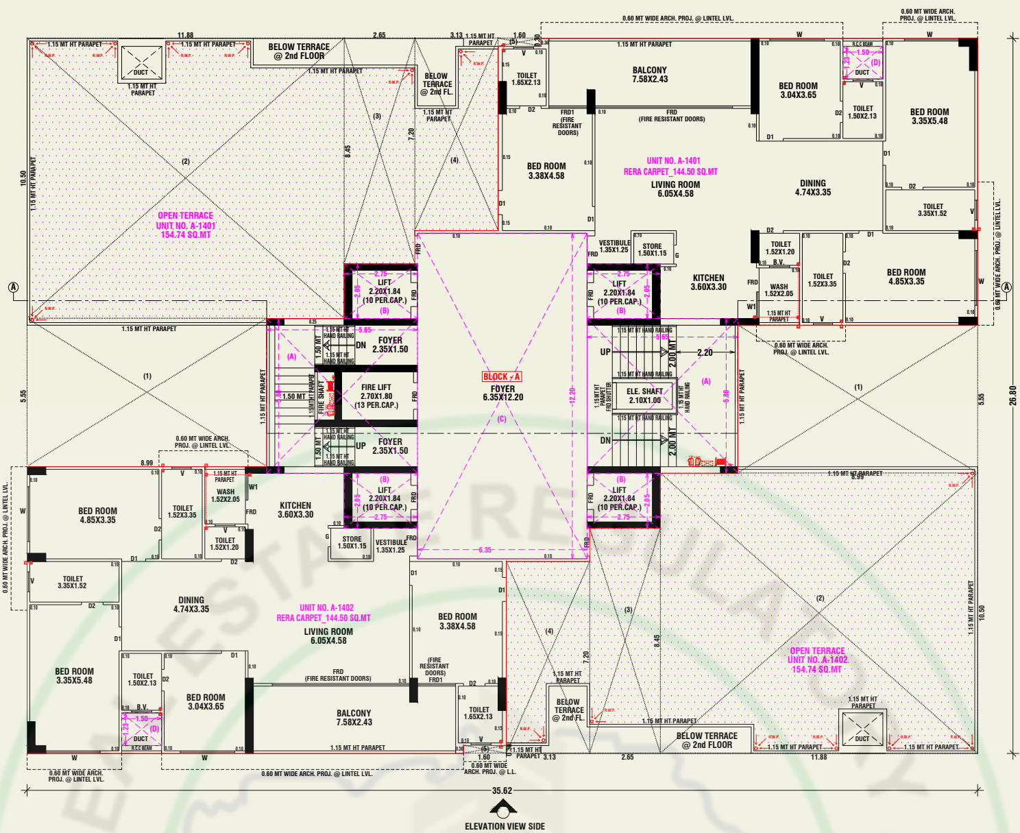
14th FLOOR PLAN (BLOCK-A)
