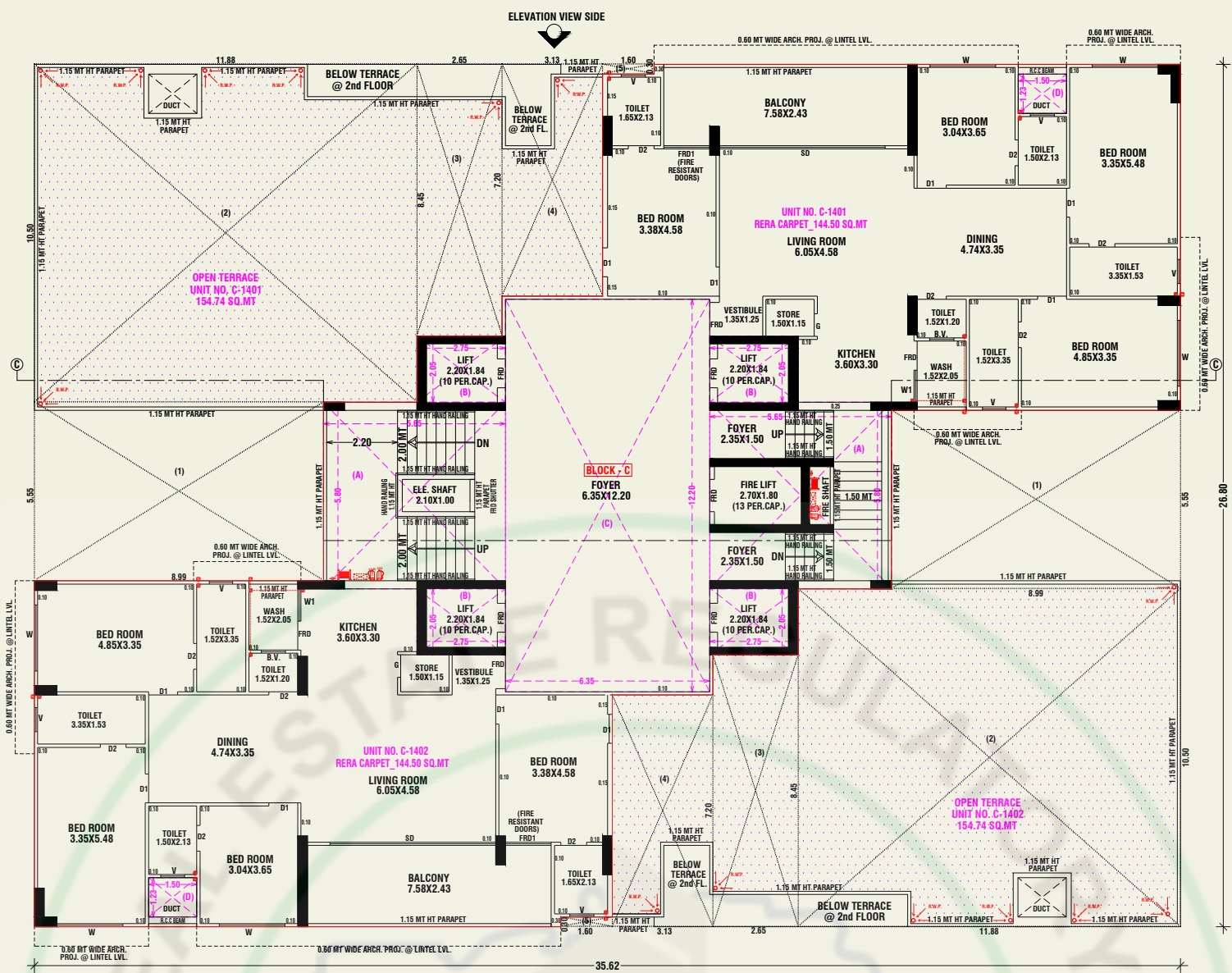
14th FLOOR PLAN (BLOCK-C)
