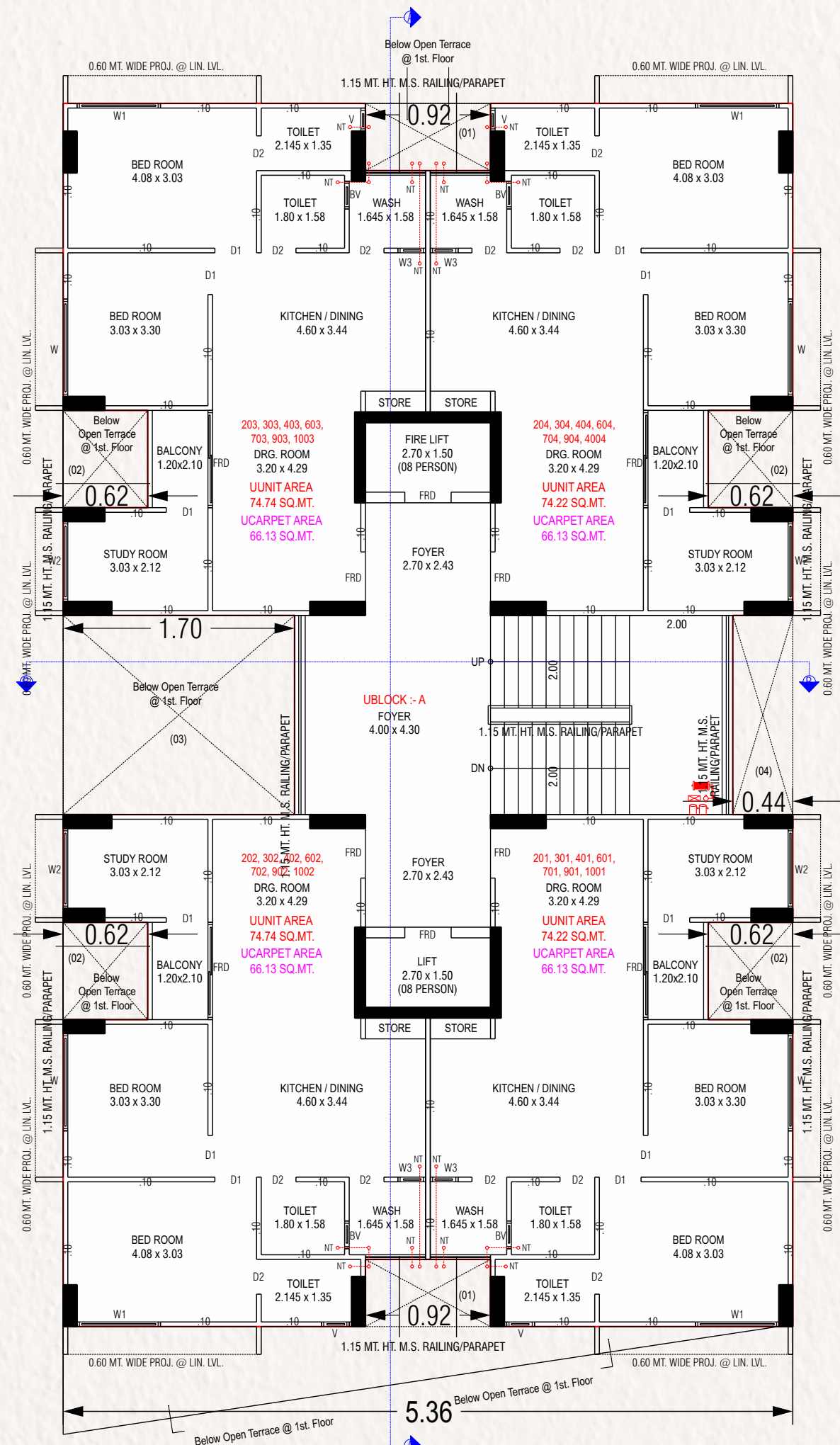
UTYPICAL (2nd. TO 4th., 6th., 7th., 9th., & 10th.) FLOOR PLAN
