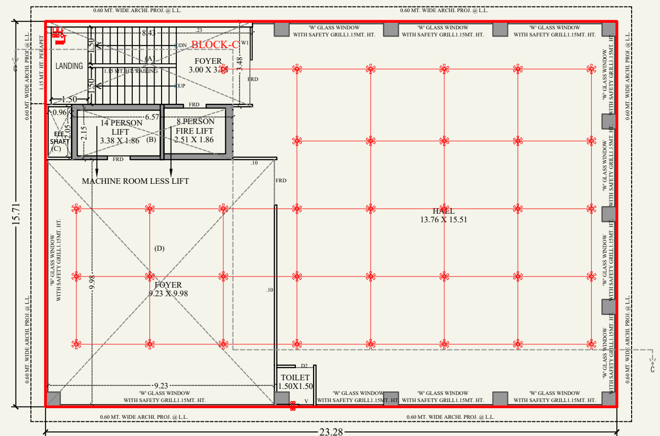
FIRST & SECOND FLOOR PLAN (BLOCK-C)
