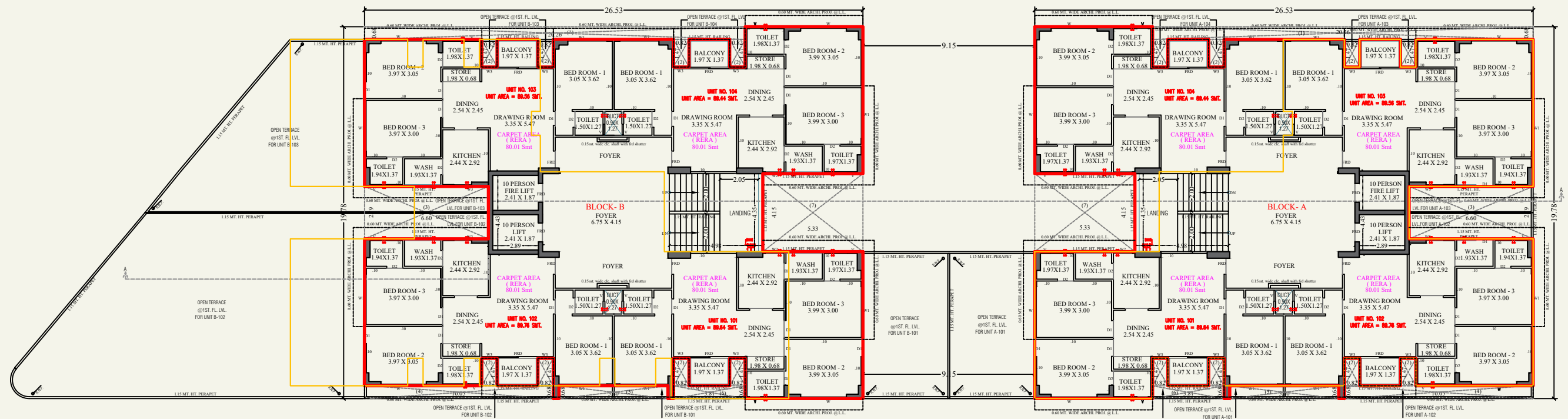
FIRST FLOOR PLAN (BLOCK-A+B)
