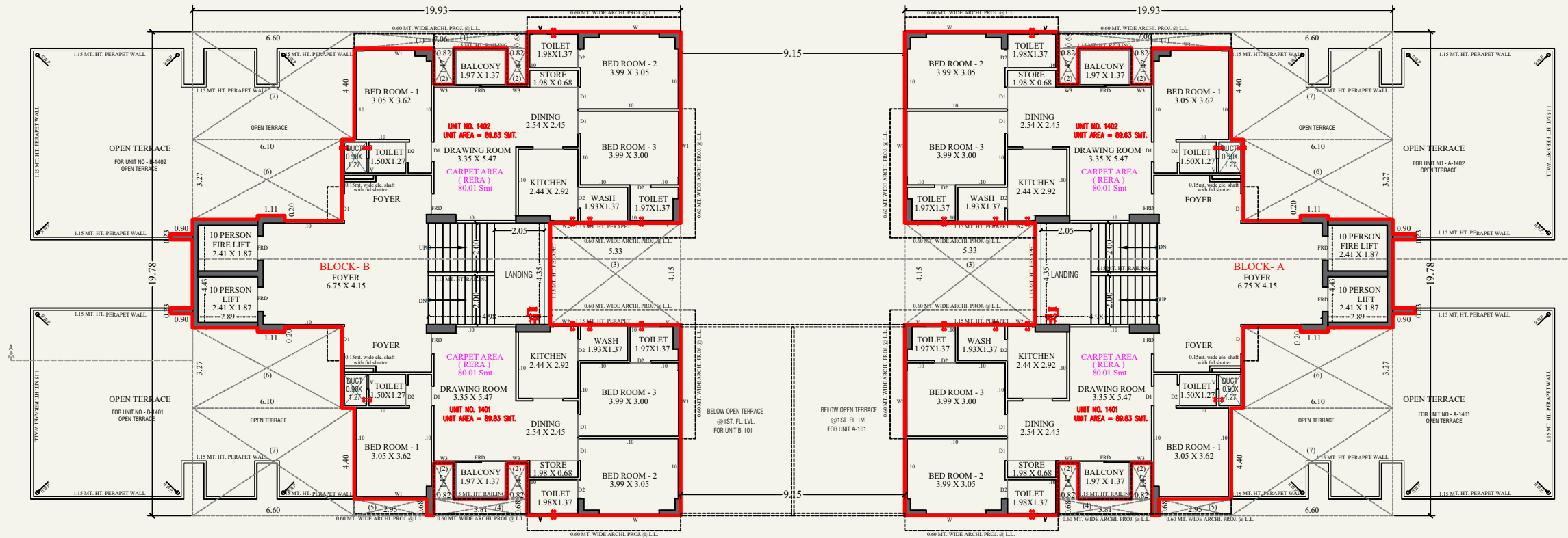
14TH. FLOOR PLAN (BLOCK-A+B)
