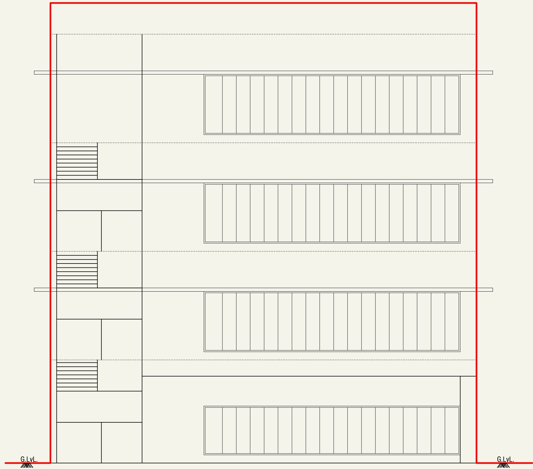
ELEVATION (BLOCK-C)
