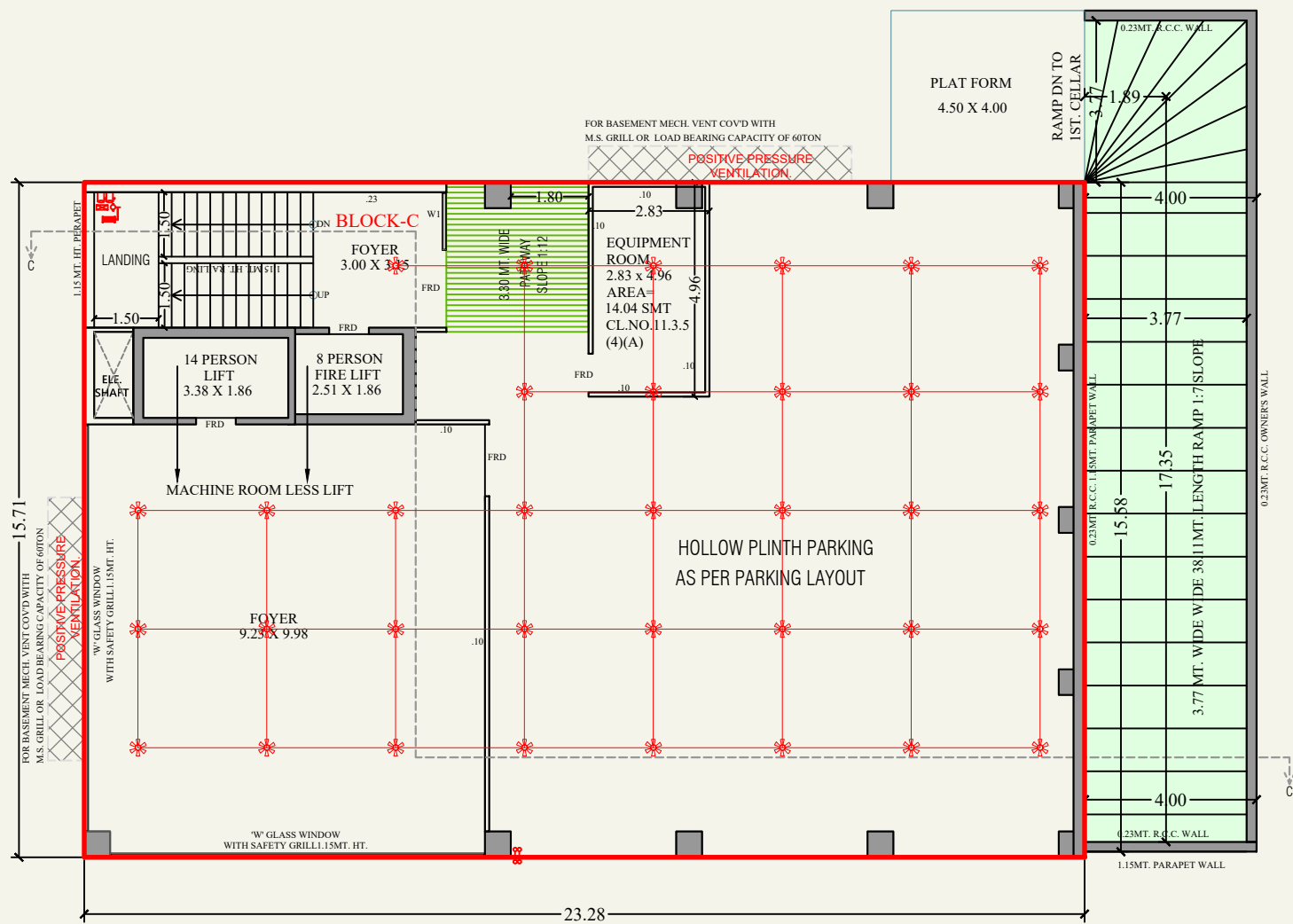
GROUND FLOOR PLAN (BLOCK-C)
