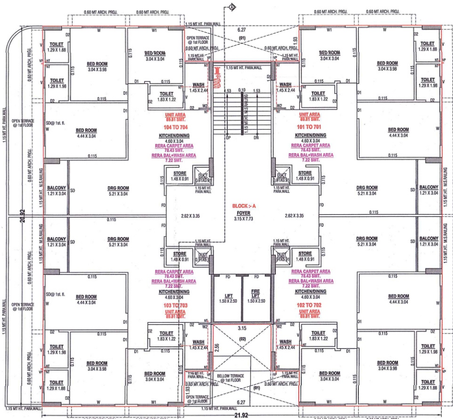
1st to 7th. FLOOR PLAN
