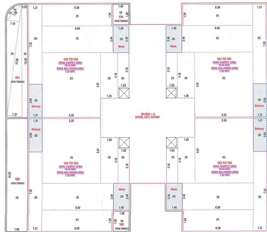
CARPET AREA (RERA) ON (1st to 7th. FLOOR)
