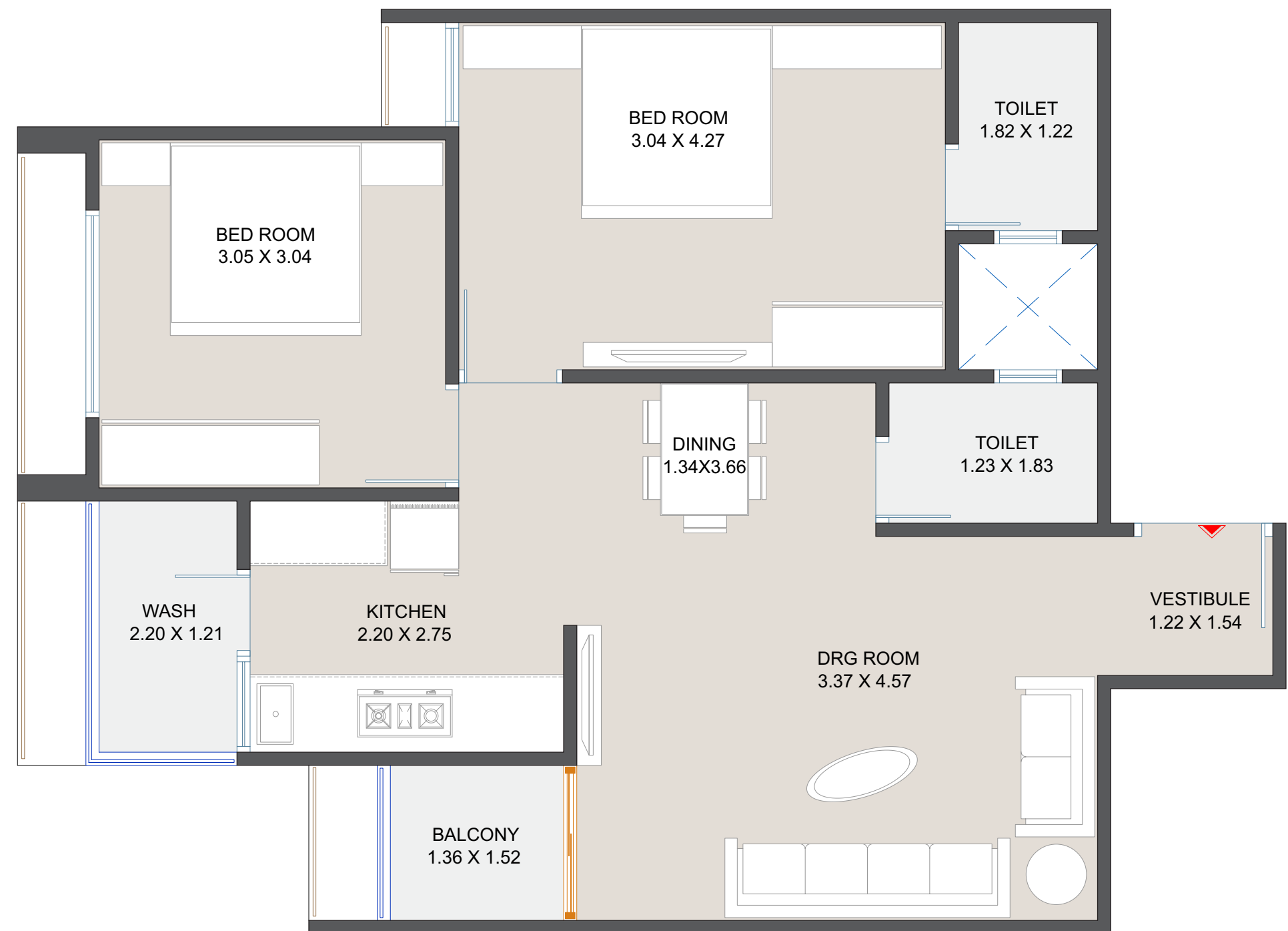
UNIT PLAN TYPE-2
